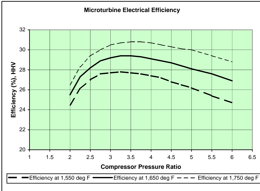
Figure 2. Microturbine Efficiency as a Function of Compressor Pressure Ratio and Turbine Firing Temperature*
