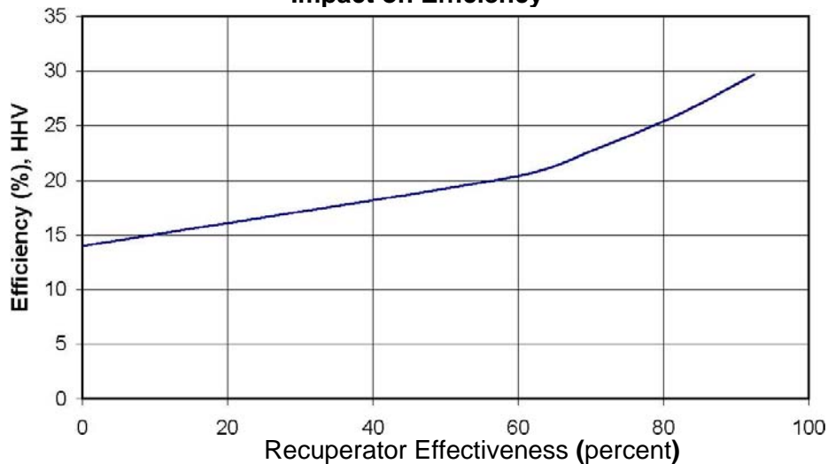
Figure 7. Microturbine Efficiency as a Function of Recuperator Effectiveness
