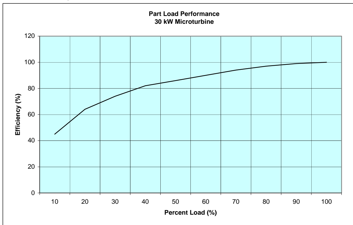
Figure 4. Microturbine Part Load Power Performance
