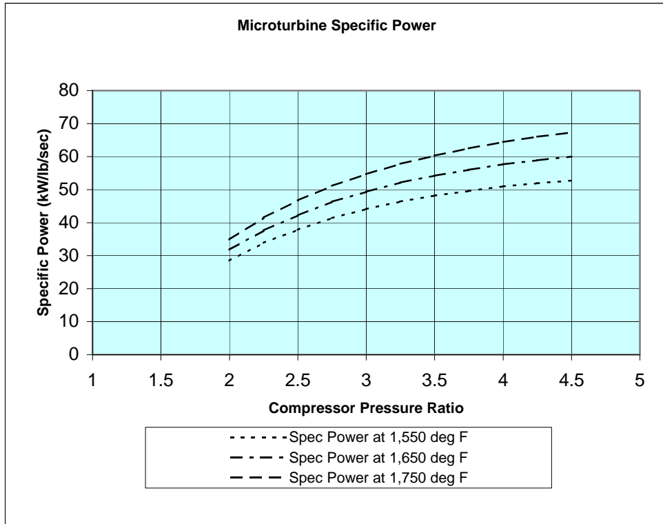
Figure 3. Microturbine Specific Power as a Function of Compressor Pressure Ratio and Turbine Firing Temperature
