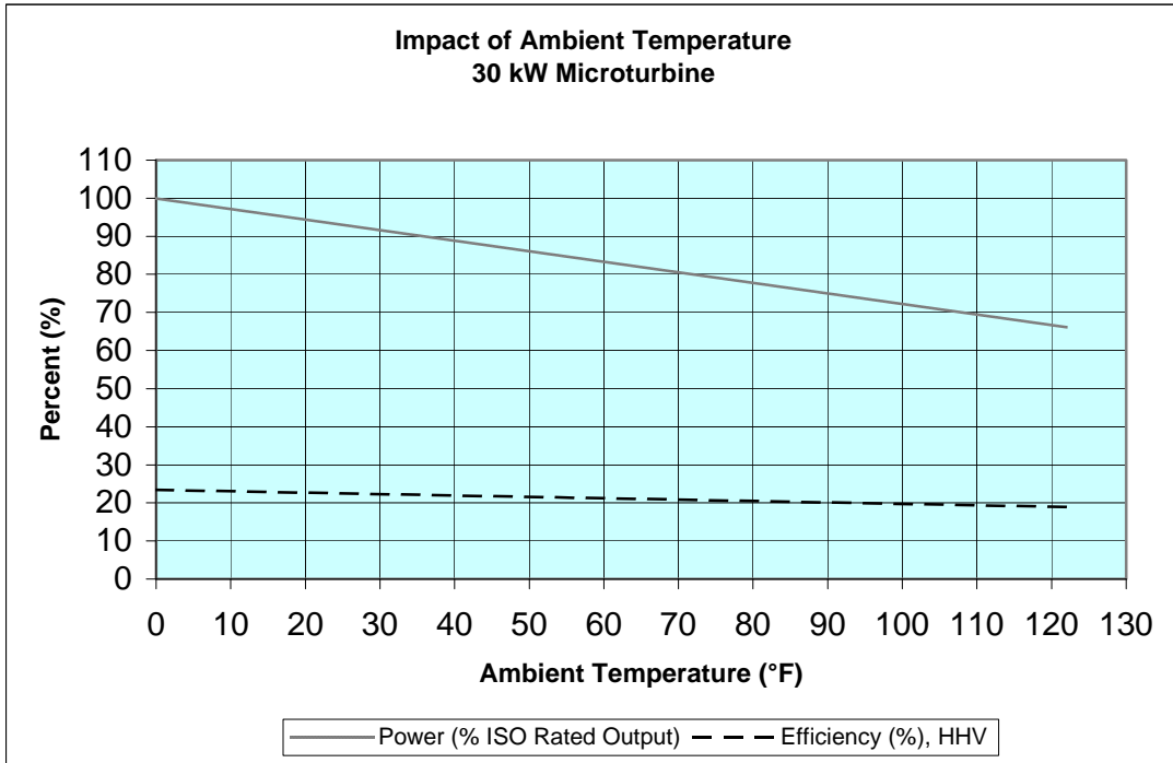
Figure 5. Ambient Temperature Effects on Microturbine Performance
