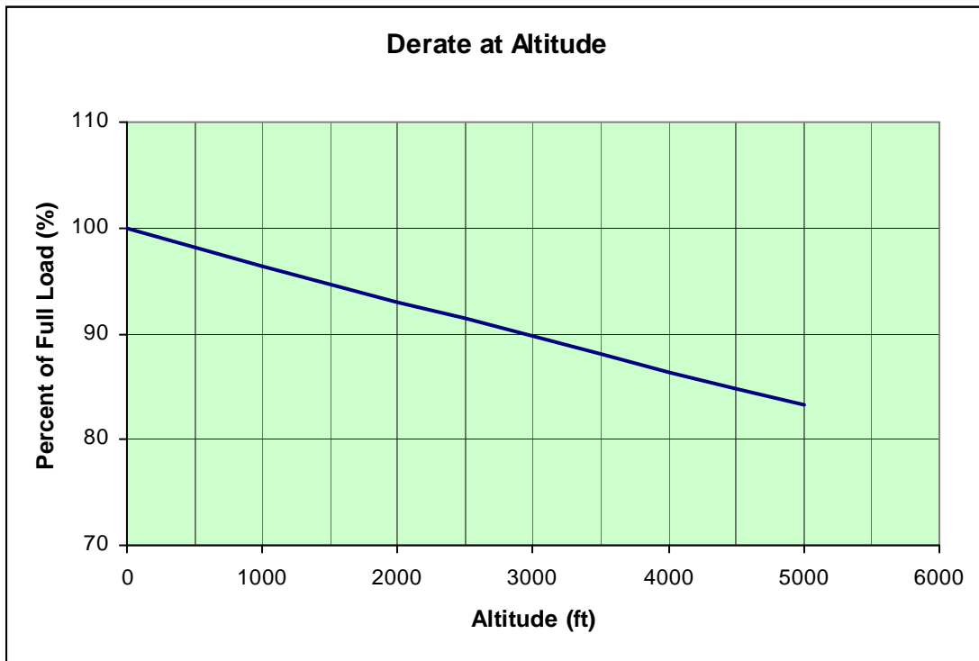
Figure 6. Altitude Effects on Microturbine Performance
