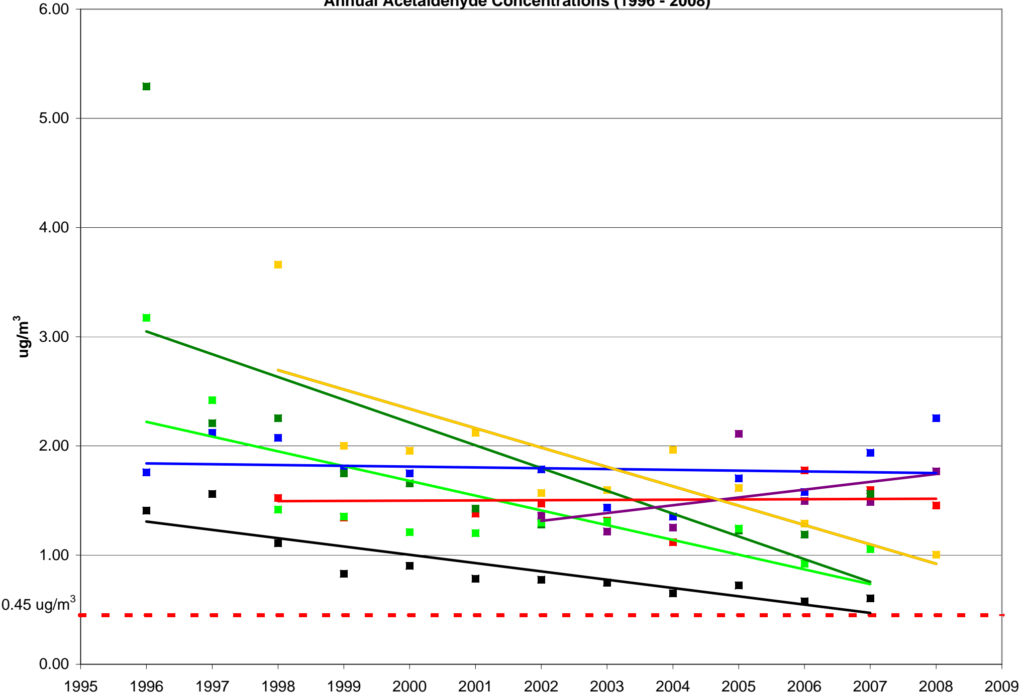
Annual Acetaldehyde Concentrations (1996 - 2008)
