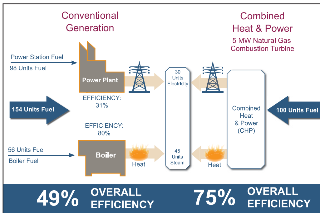
Figure 1. CHP System Efficiency
