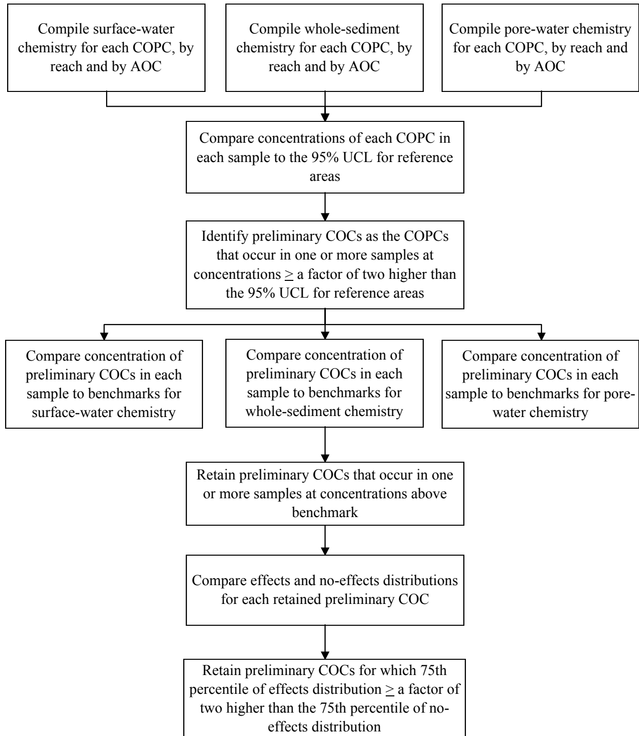
Figure 4-7. Overview of the approach that was used to identify contaminants of concern in surface water, whole sediment, and pore water from the Calcasieu Estuary.
