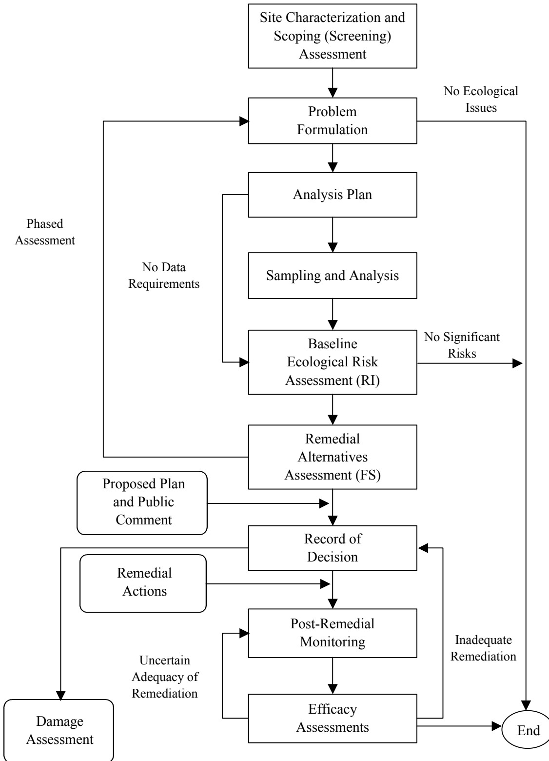
Figure 10-2. A flowchart of the general remedial process for contaminated sites (from Suter et al. 2002).
