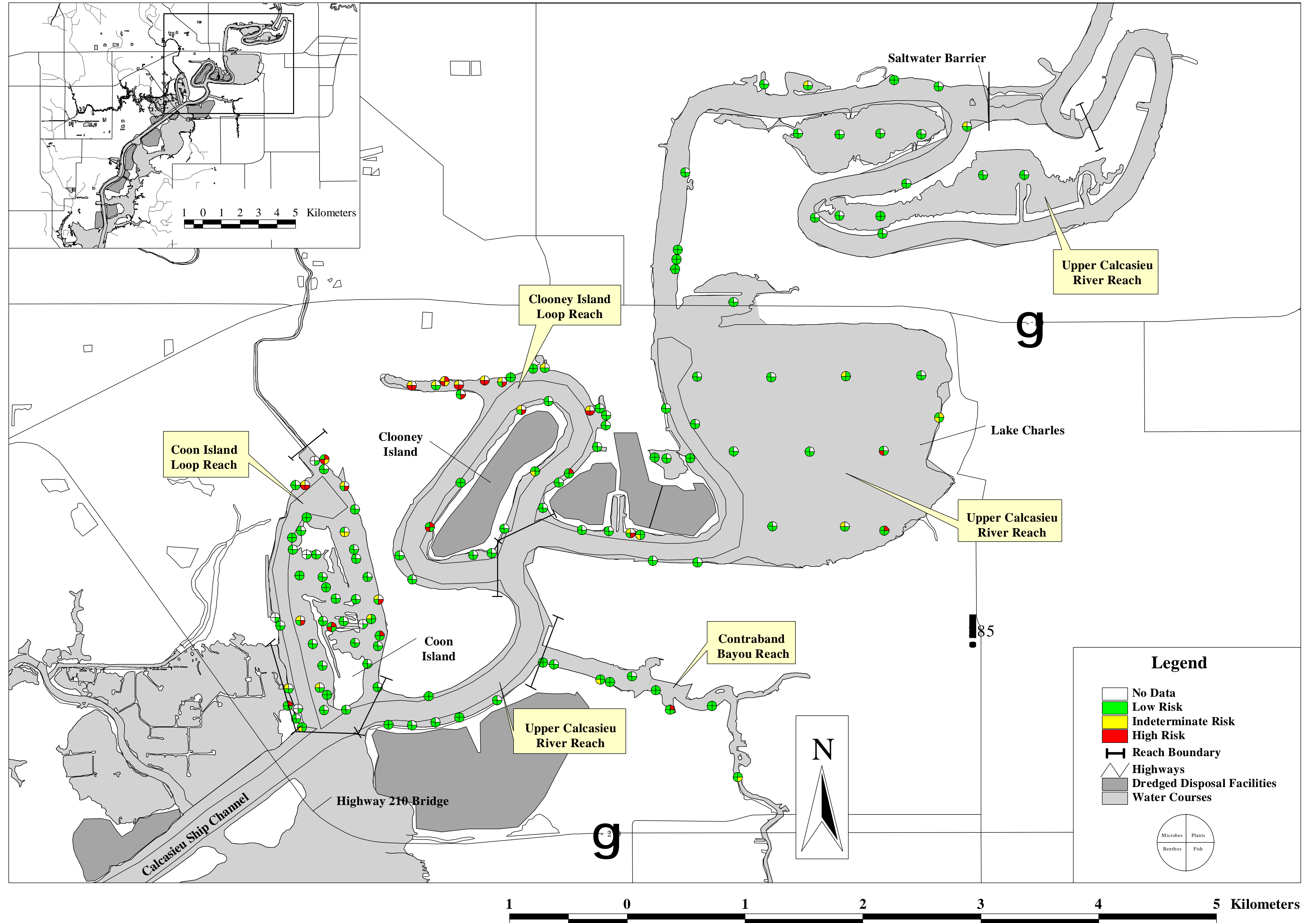
Figure ES-12. Map of the Upper Calcasieu River AOC, showing the reach boundaries and locations of samples (surface water and surface sediments) that pose low, indeterminate or high risk to the microbial, aquatic plant, benthic invertebrate, and fish communities considering multiple lines of evidence.
