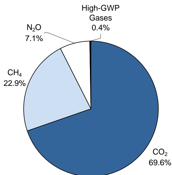
Figure 2-1: Contribution of Anthropogenic Emissions of Greenhouse Gases to the Enhanced Greenhouse Effect from Preindustrial to Present (measured in watts/meter 2 )
