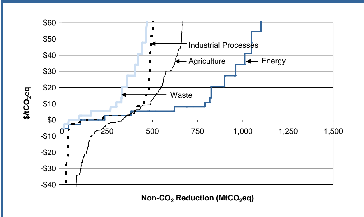
Figure 4-5: Global 2020 MACs for Non-CO 2 Greenhouse Gases by Major Sector
