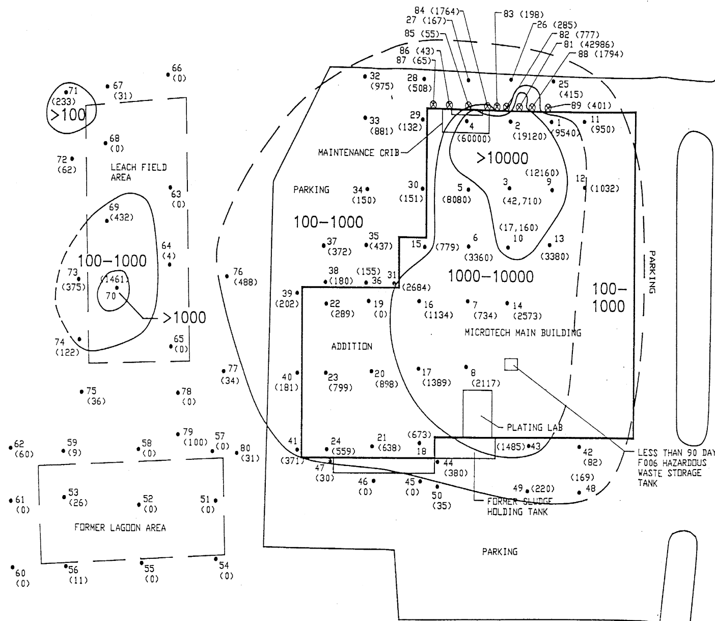
FIGURE 4 PCE DISTRIBUTION IN SOIL GAS MICROTECH, INC. CHESHIRE, CT. HRP #MIC.0018.RA NOT TO SCALE
