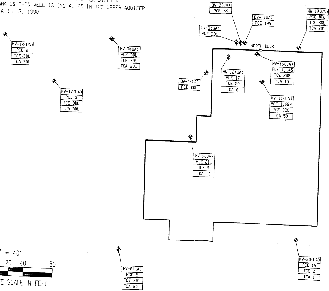
FIGURE 6 SOLVENT DISTRIBUTION IN THE UNCONSOLIDATED AQUIFER MICROTECH, INC. CHESHIRE, CT. HRP # MIC0020.RA T-7 APPROX. SCALE 1" = 40'
