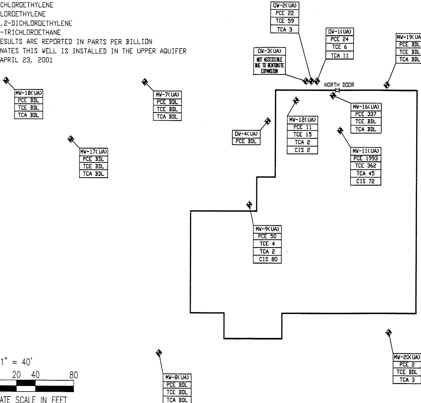
FIGURE 4 SOLVENT DISTRIBUTION IN THE UNCONSOLIDATED AQUIFER MICROTECH, INC. CHESHIRE, CT. HRP # MIC0032.HG APPROX. SCALE 1" = 40'
