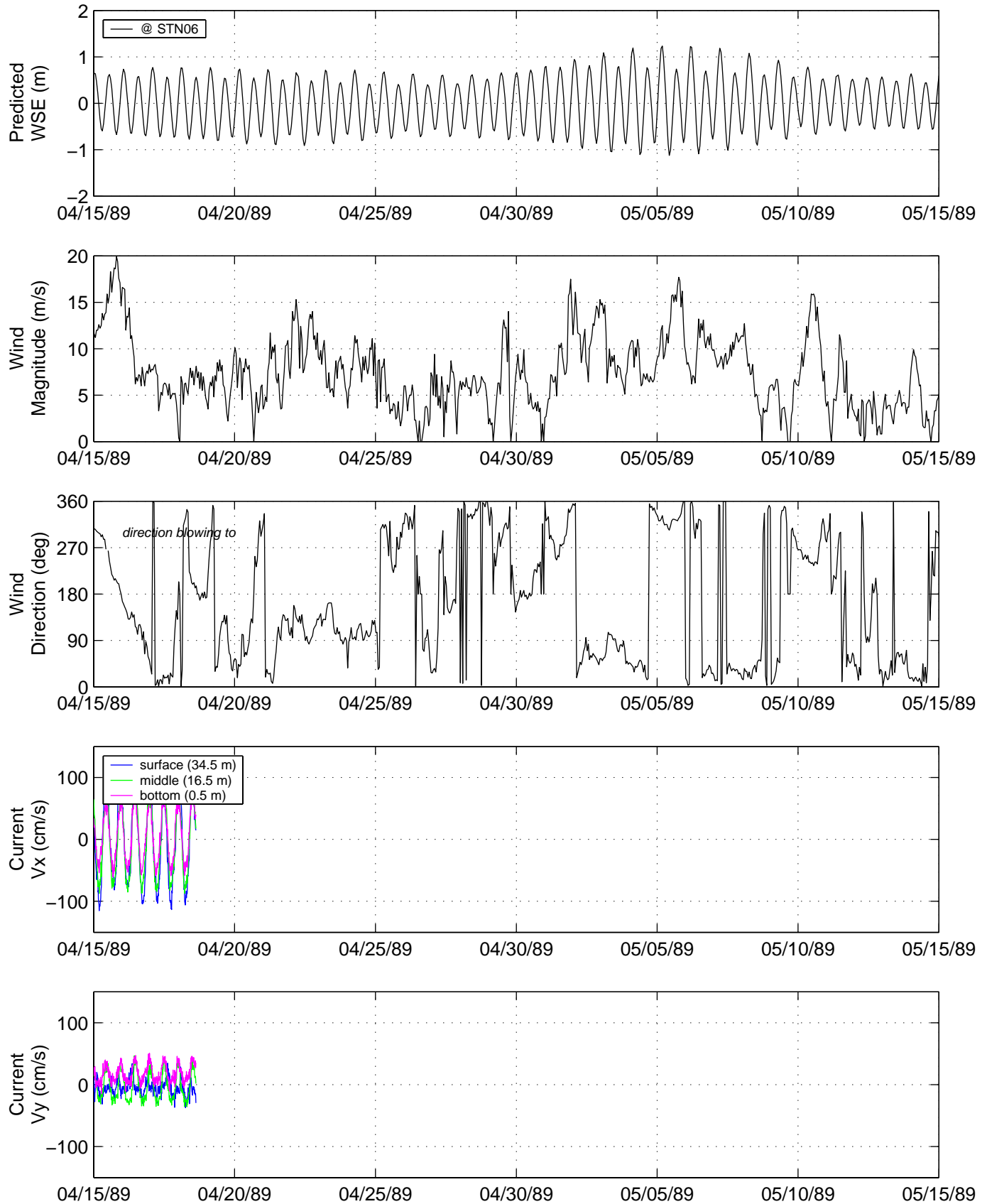
FIGURE 3-22 DIRECTIONAL WATER VELOCITY AND RELATED MEASUREMENTS COLLECTED DURING DEPLOYMENT NOS21-01 (PAGE 2 OF 2)
