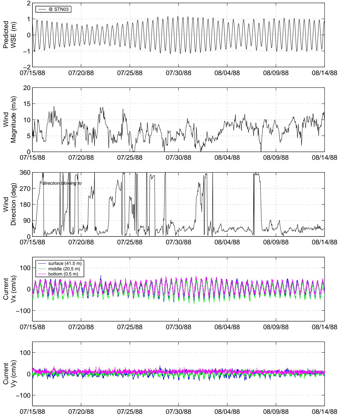
FIGURE 3-19 DIRECTIONAL WATER VELOCITY AND RELATED MEASUREMENTS COLLECTED DURING DEPLOYMENT NOS08-01 (PAGE 1 OF 3)
