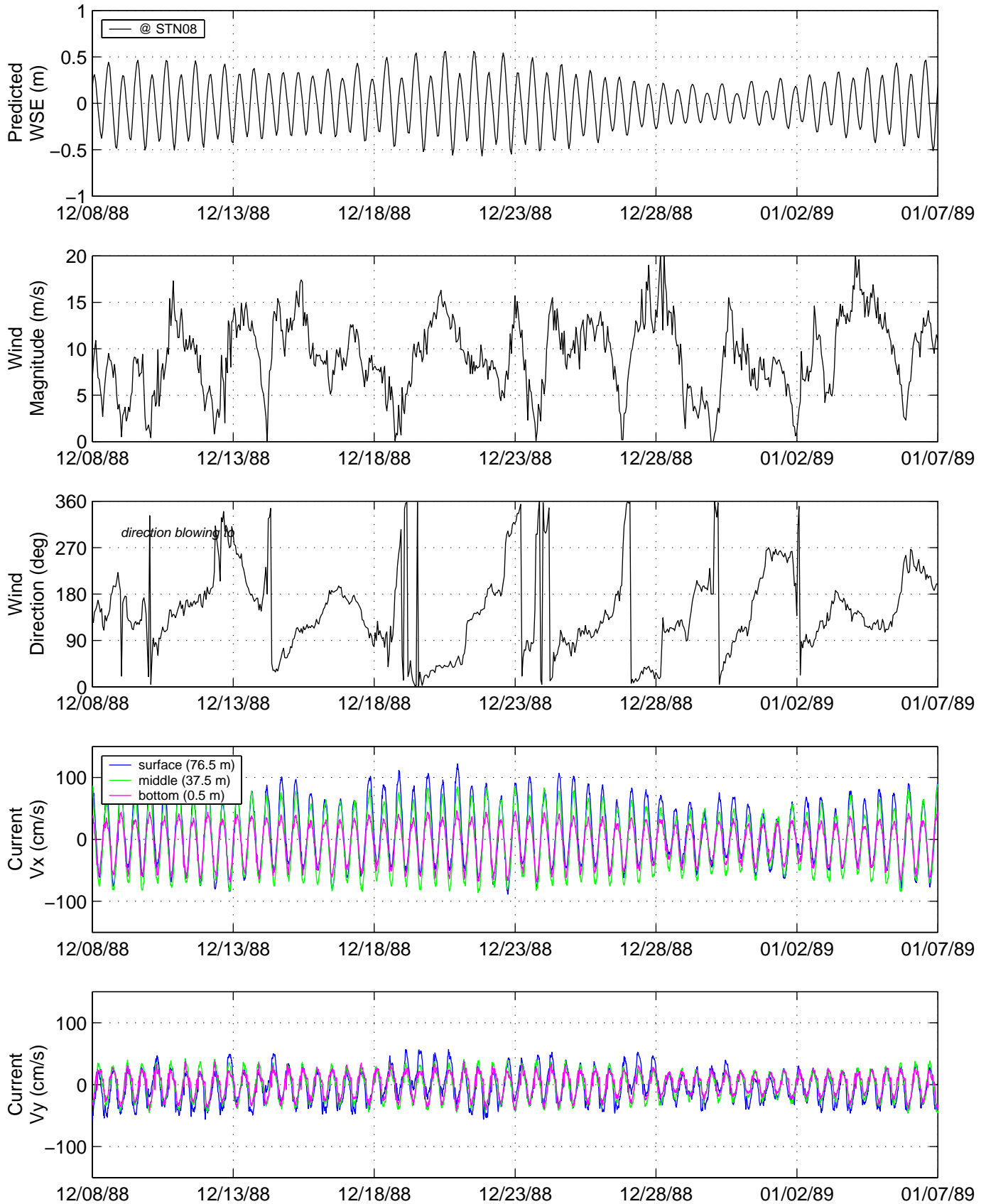
FIGURE 3-21 DIRECTIONAL WATER VELOCITY AND RELATED MEASUREMENTS COLLECTED DURING DEPLOYMENT NOS13-02 (PAGE 1 OF 2)
