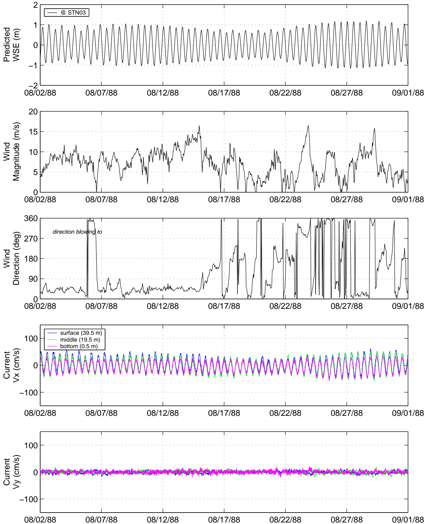
FIGURE 3-20 DIRECTIONAL WATER VELOCITY AND RELATED MEASUREMENTS COLLECTED DURING DEPLOYMENT NOS09-01 (PAGE 1 OF 2)
