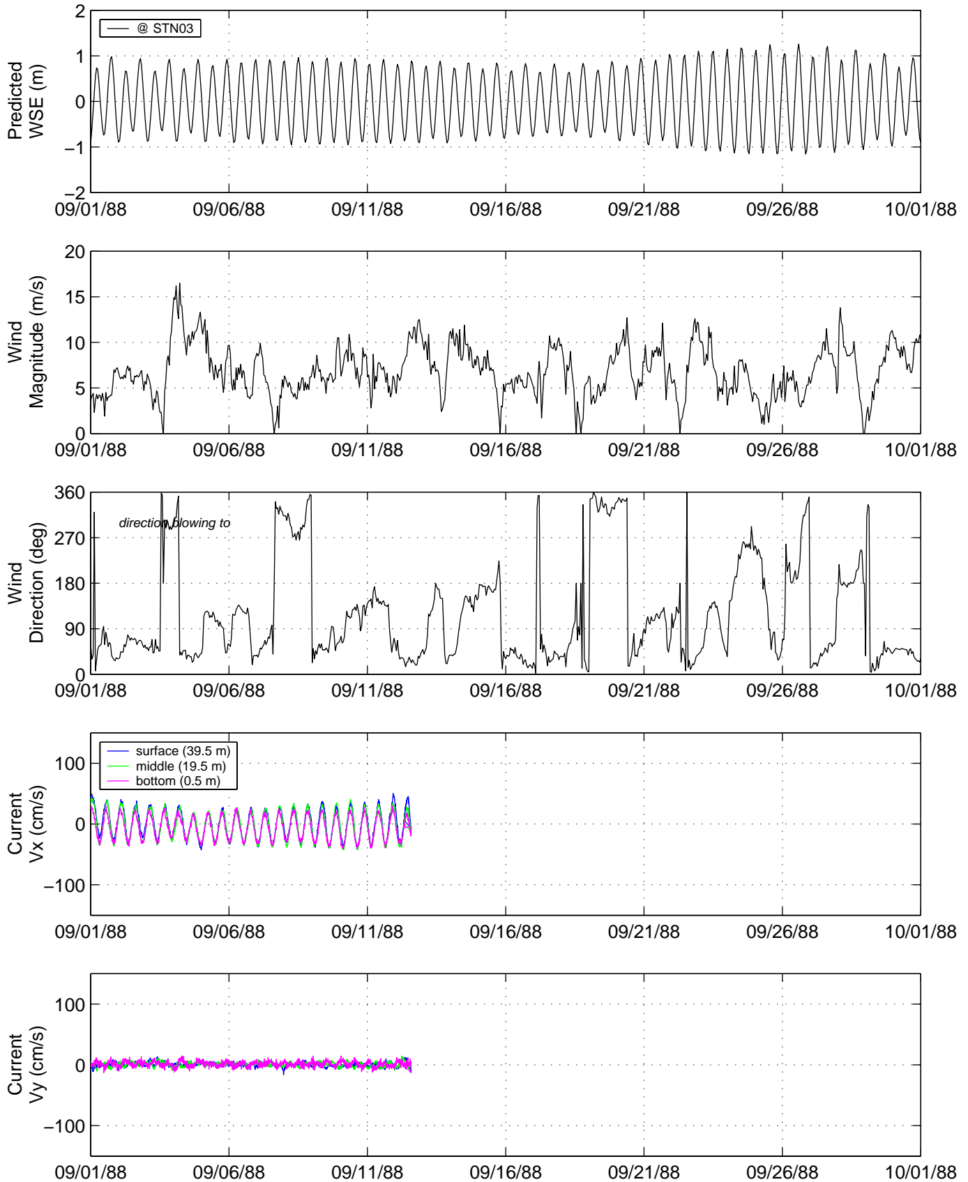
FIGURE 3-20 DIRECTIONAL WATER VELOCITY AND RELATED MEASUREMENTS COLLECTED DURING DEPLOYMENT NOS09-01 (PAGE 2 OF 2)
