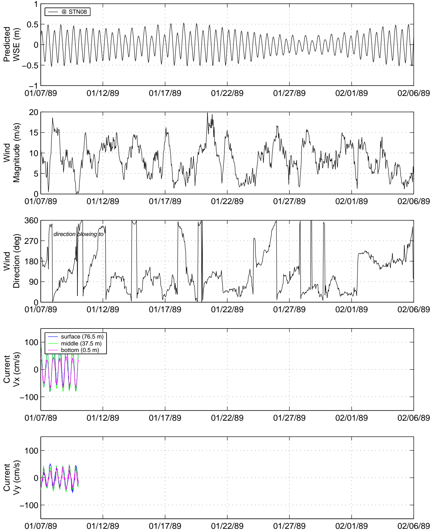
FIGURE 3-21 DIRECTIONAL WATER VELOCITY AND RELATED MEASUREMENTS COLLECTED DURING DEPLOYMENT NOS13-02 (PAGE 2 OF 2)
