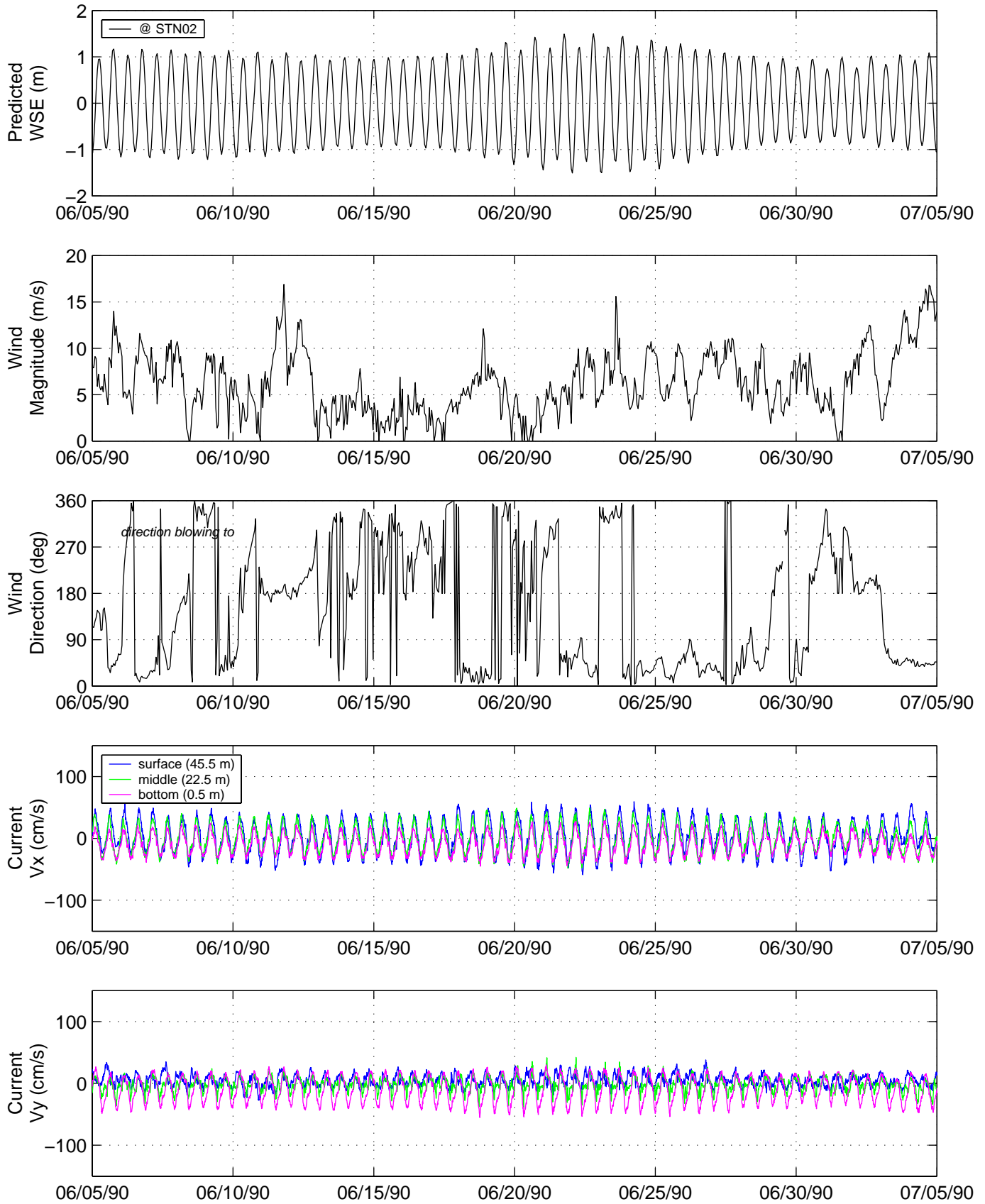
FIGURE 3-18 DIRECTIONAL WATER VELOCITY AND RELATED MEASUREMENTS COLLECTED DURING DEPLOYMENT NOS07-02 (PAGE 2 OF 3)
