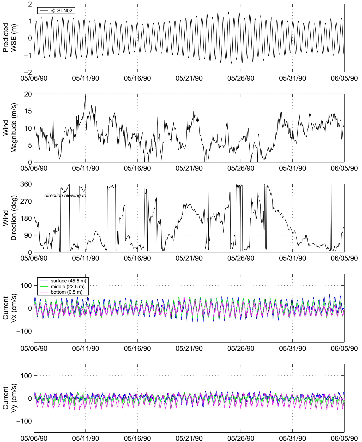
FIGURE 3-18 DIRECTIONAL WATER VELOCITY AND RELATED MEASUREMENTS COLLECTED DURING DEPLOYMENT NOS07-02 (PAGE 1 OF 3)
