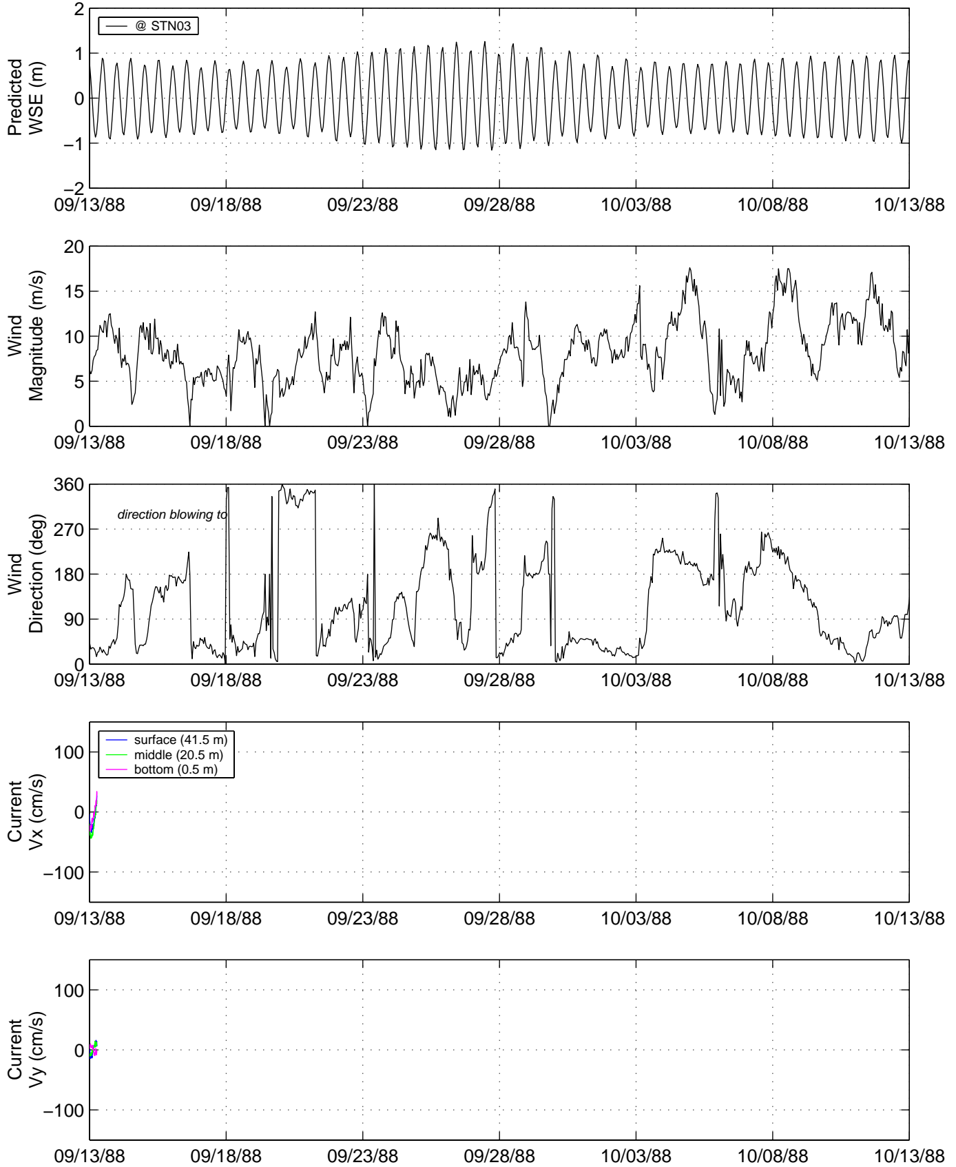
FIGURE 3-19 DIRECTIONAL WATER VELOCITY AND RELATED MEASUREMENTS COLLECTED DURING DEPLOYMENT NOS08-01 (PAGE 3 OF 3)
