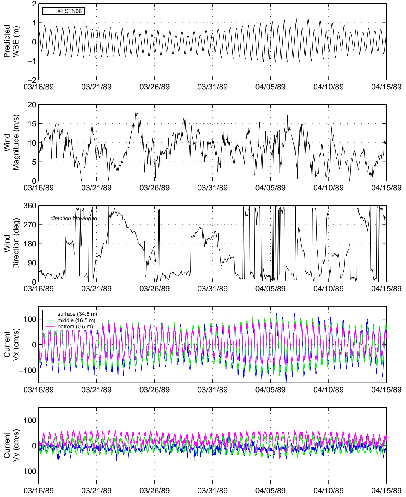
FIGURE 3-22 DIRECTIONAL WATER VELOCITY AND RELATED MEASUREMENTS COLLECTED DURING DEPLOYMENT NOS21-01 (PAGE 1 OF 2)
