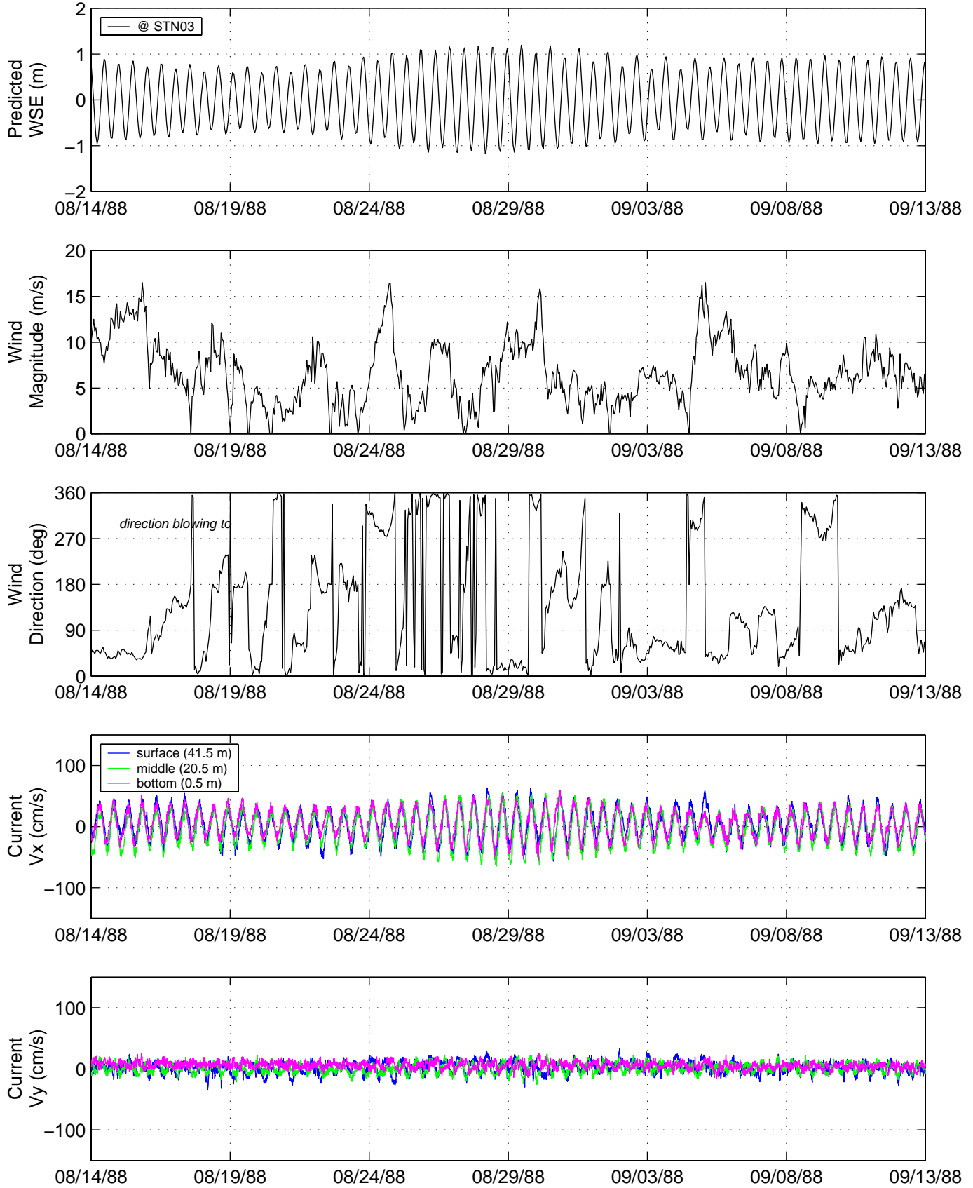
FIGURE 3-19 DIRECTIONAL WATER VELOCITY AND RELATED MEASUREMENTS COLLECTED DURING DEPLOYMENT NOS08-01 (PAGE 2 OF 3)
