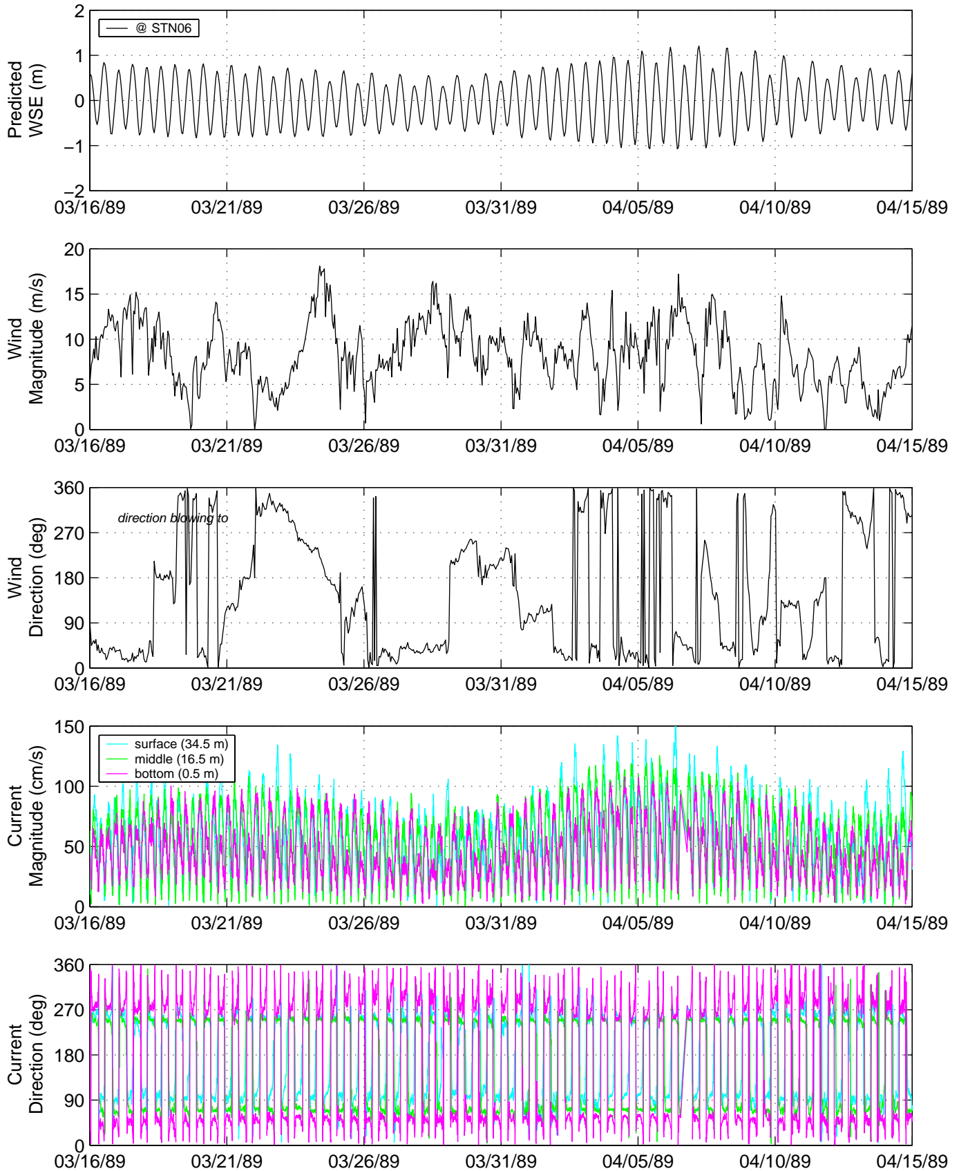
FIGURE 3-17 WATER VELOCITY MAGNITUDE AND RELATED MEASUREMENTS COLLECTED DURING DEPLOYMENT NOS21-01 (PAGE 1 OF 2)
