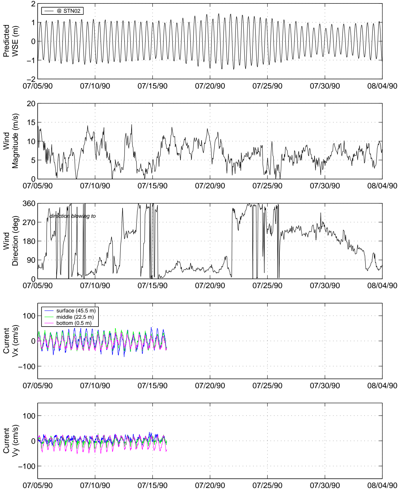
FIGURE 3-18 DIRECTIONAL WATER VELOCITY AND RELATED MEASUREMENTS COLLECTED DURING DEPLOYMENT NOS07-02 (PAGE 3 OF 3)
