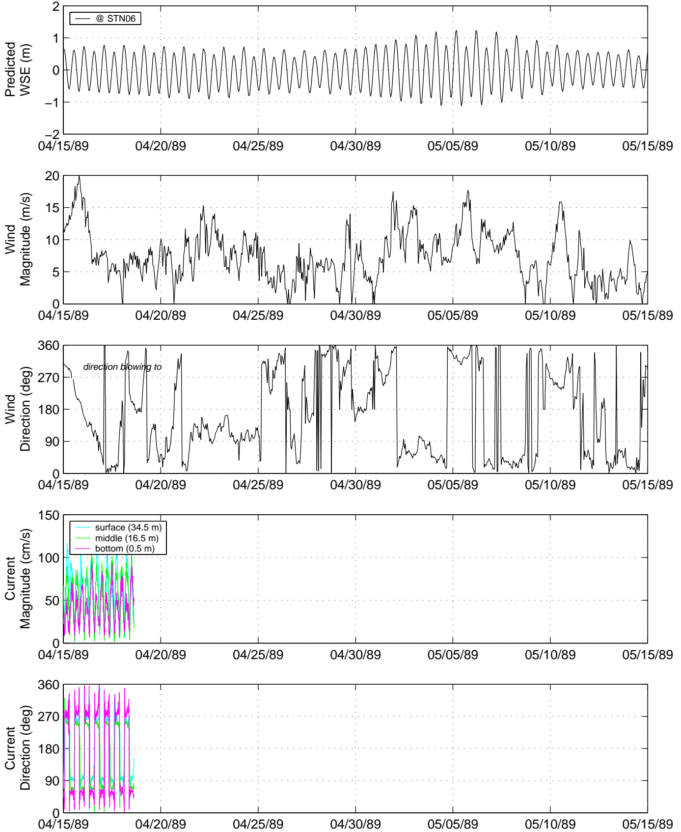
FIGURE 3-17 WATER VELOCITY MAGNITUDE AND RELATED MEASUREMENTS COLLECTED DURING DEPLOYMENT NOS21-01 (PAGE 2 OF 2)
