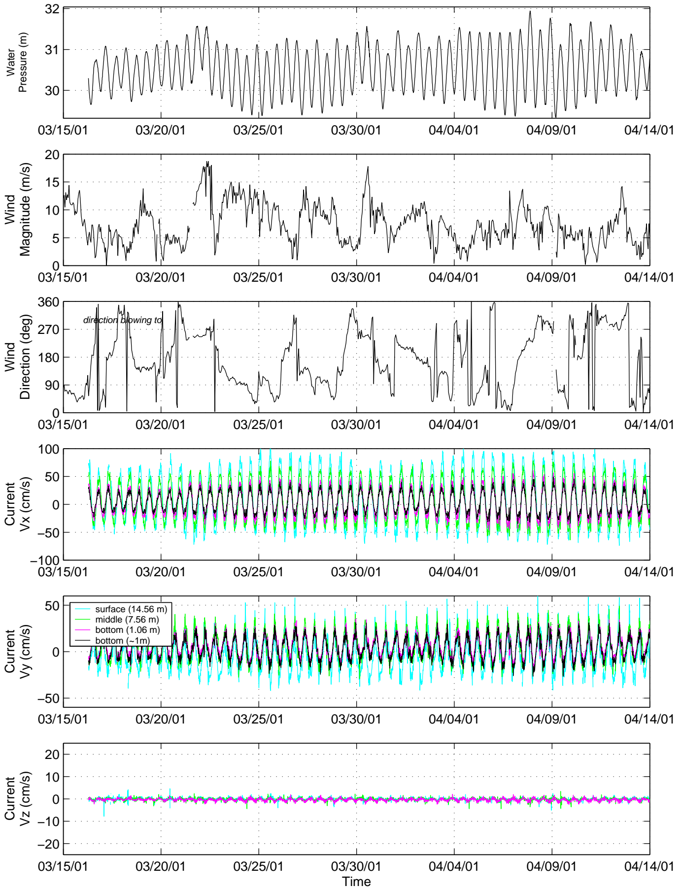
FIGURE 5-17 DIRECTIONAL WATER VELOCITY AND RELATED MEASUREMENTS COLLECTED AT STATION 06 (PAGE 1 OF 2)
