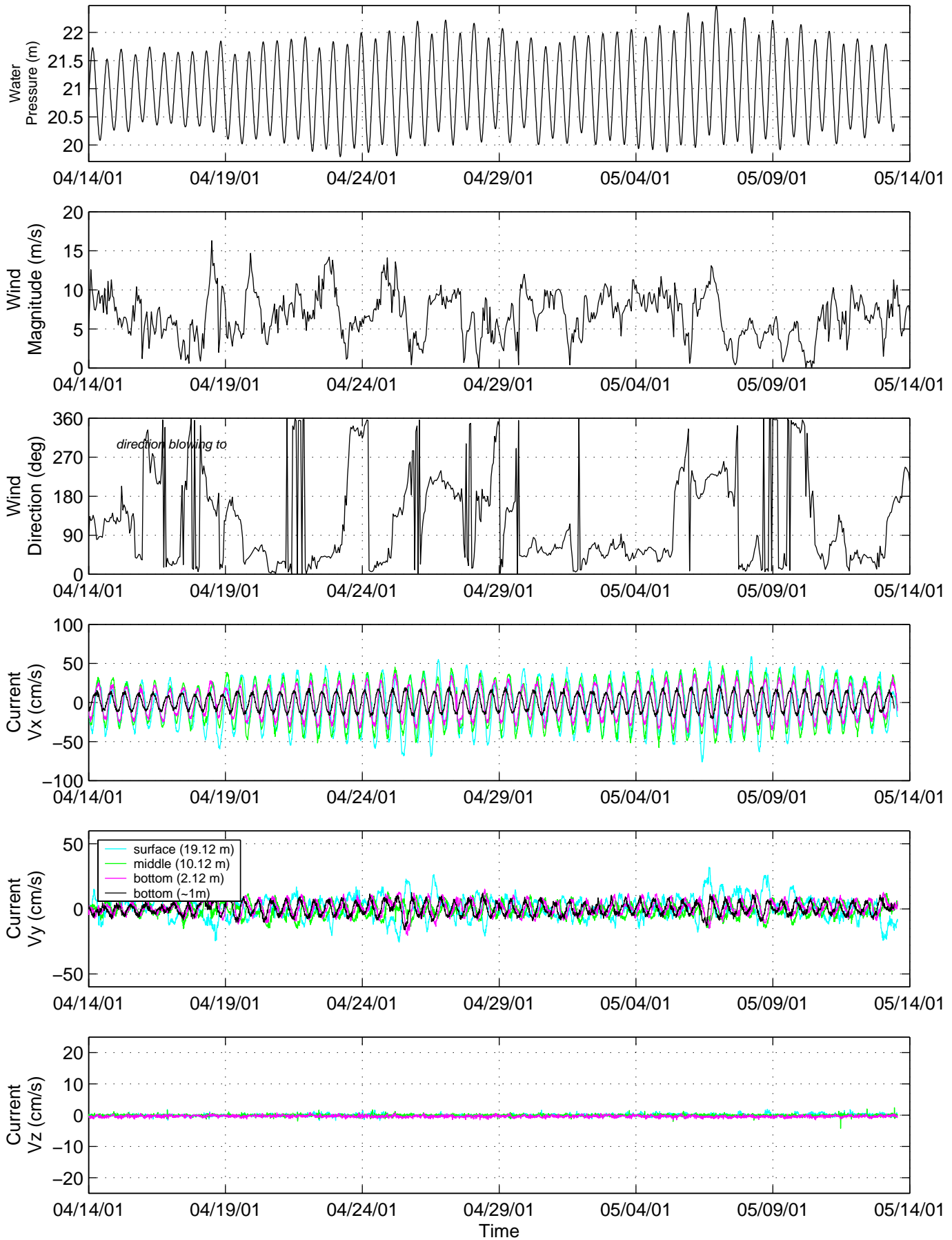
FIGURE 5-16 DIRECTIONAL WATER VELOCITY AND RELATED MEASUREMENTS COLLECTED AT STATION 04 (PAGE 2 OF 2)
