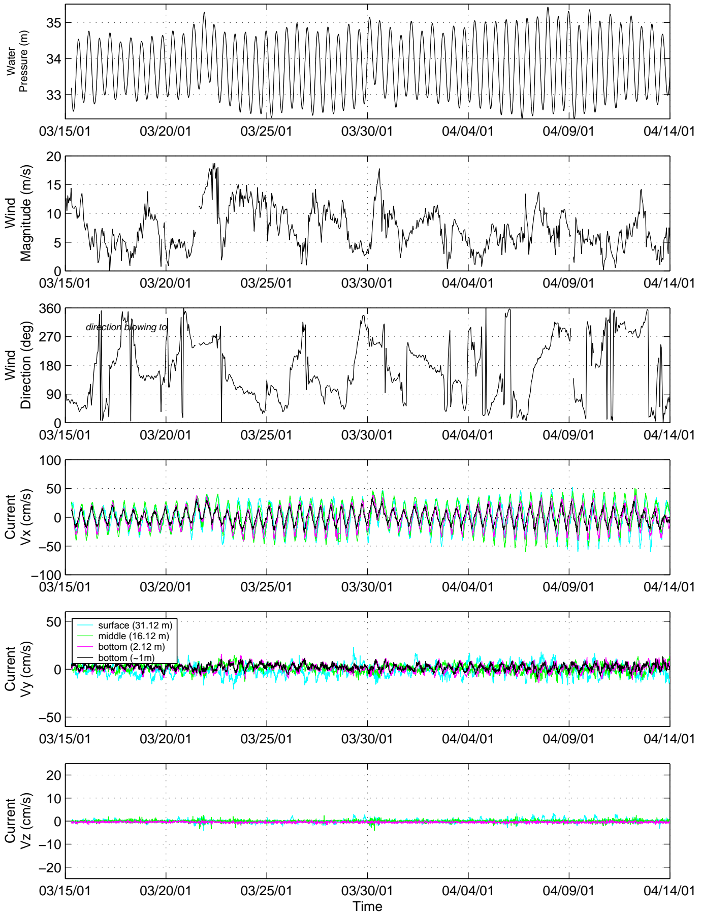
FIGURE 5-15 DIRECTIONAL WATER VELOCITY AND RELATED MEASUREMENTS COLLECTED AT STATION 01 (PAGE 1 OF 2)
