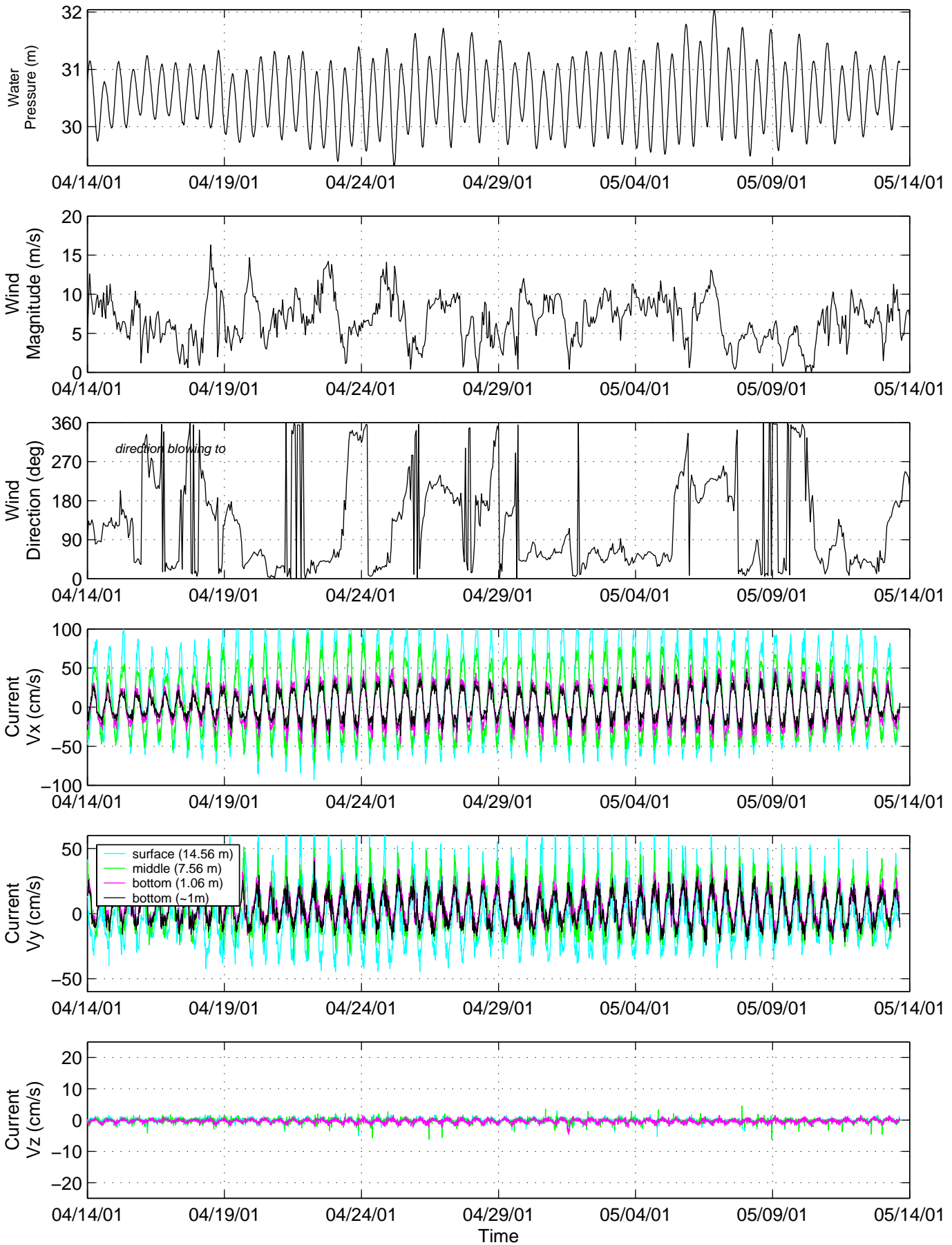
FIGURE 5-17 DIRECTIONAL WATER VELOCITY AND RELATED MEASUREMENTS COLLECTED AT STATION 06 (PAGE 2 OF 2)
