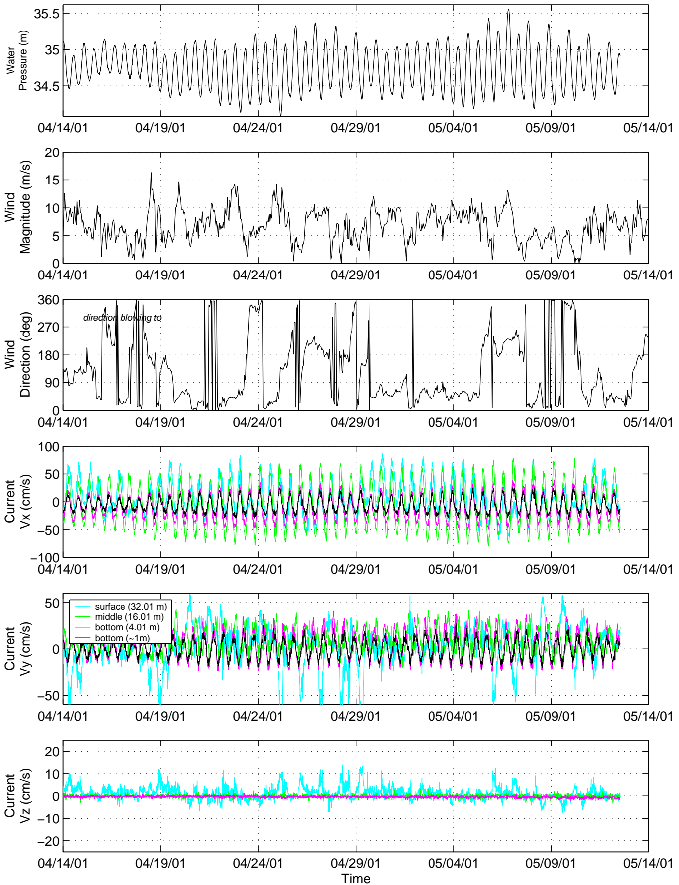
FIGURE 5-18 DIRECTIONAL WATER VELOCITY AND RELATED MEASUREMENTS COLLECTED AT STATION 10 (PAGE 2 OF 2)
