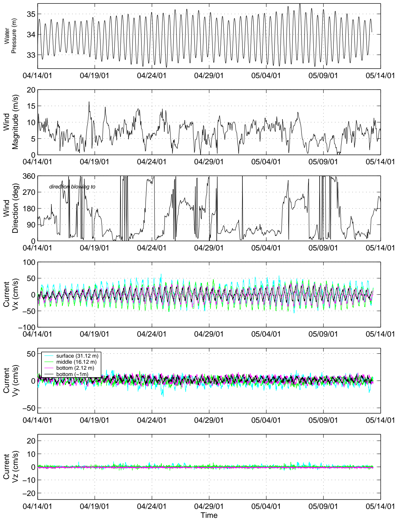
FIGURE 5-15 DIRECTIONAL WATER VELOCITY AND RELATED MEASUREMENTS COLLECTED AT STATION 01 (PAGE 2 OF 2)
