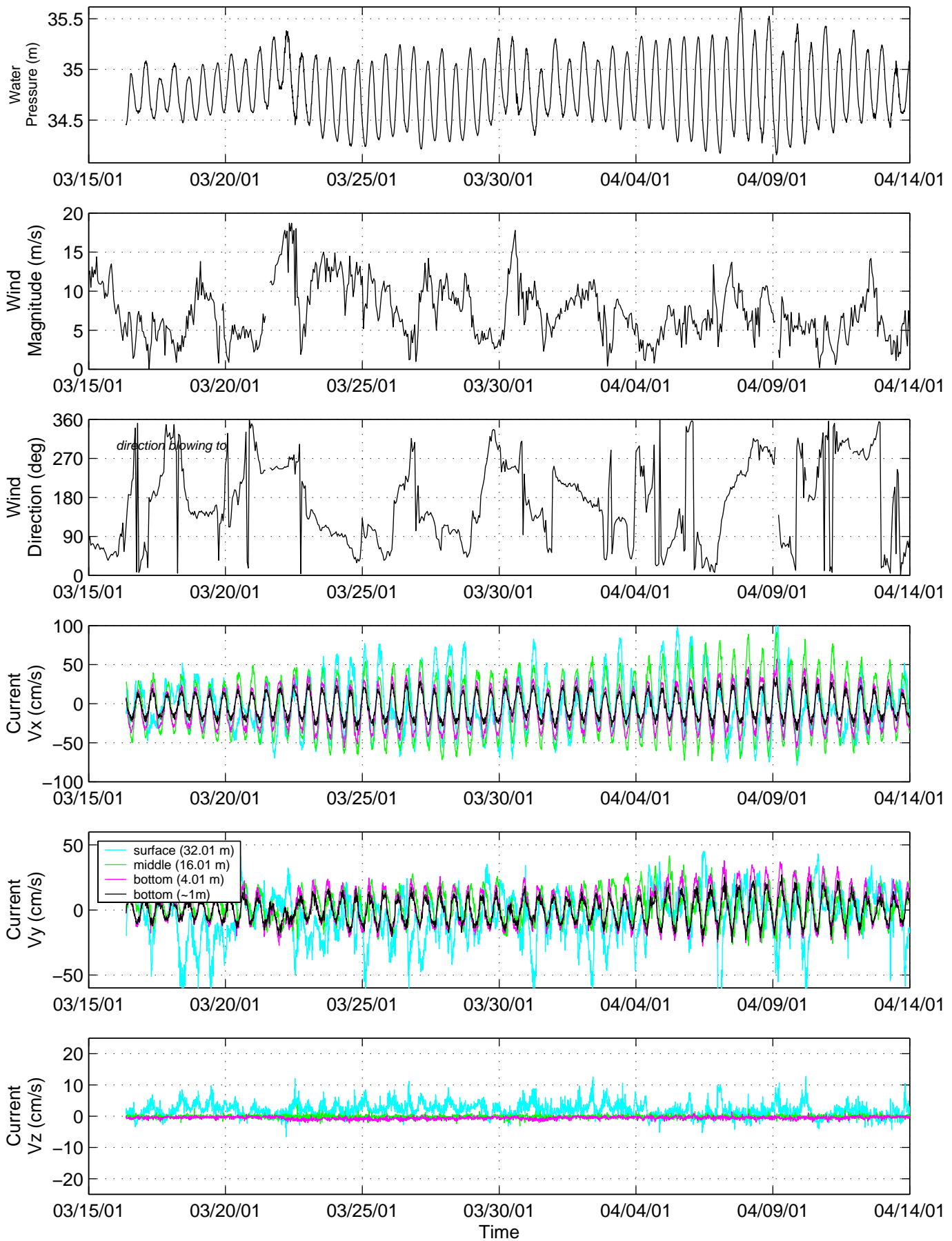
FIGURE 5-18 DIRECTIONAL WATER VELOCITY AND RELATED MEASUREMENTS COLLECTED AT STATION 10 (PAGE 1 OF 2)
