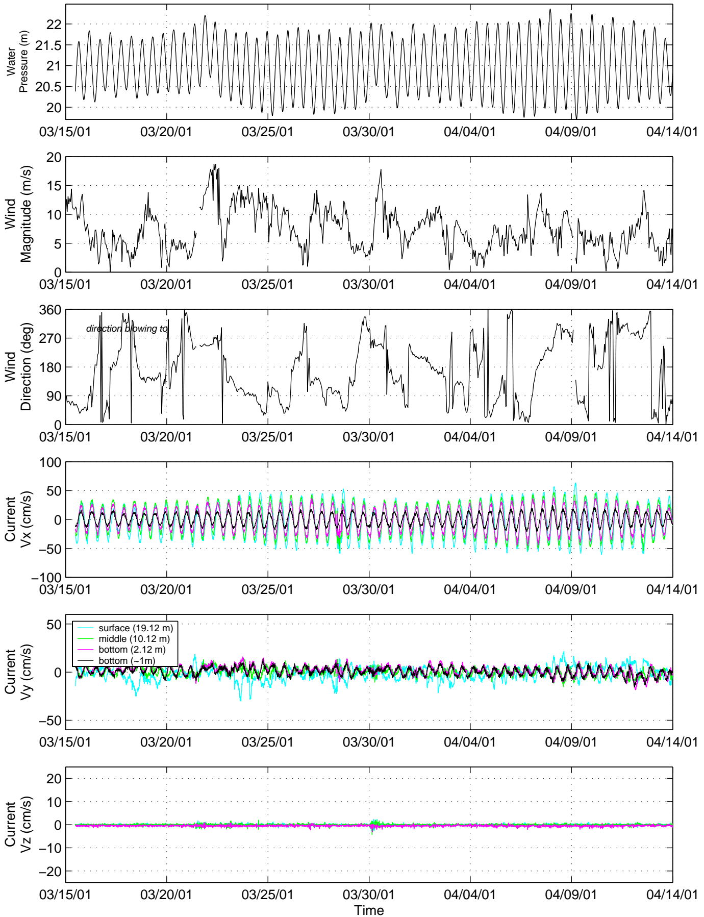
FIGURE 5-16 DIRECTIONAL WATER VELOCITY AND RELATED MEASUREMENTS COLLECTED AT STATION 04 (PAGE 1 OF 2)
