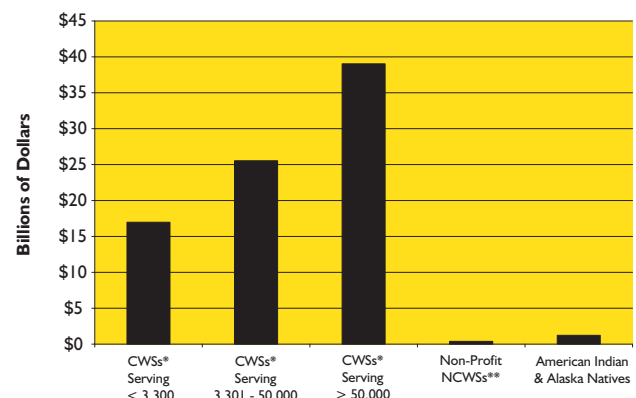
Figure 2: Total Transmission & Distribution Infrastructure Need by System Size (in billions of 1999 $)
