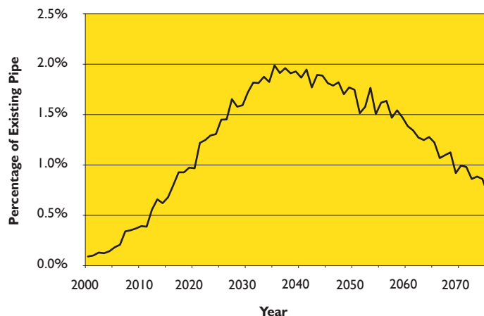
Figure 1: Projected Annual Percentage of Transmission Lines and Distribution Mains Requiring Replacement, 2000 - 2075
