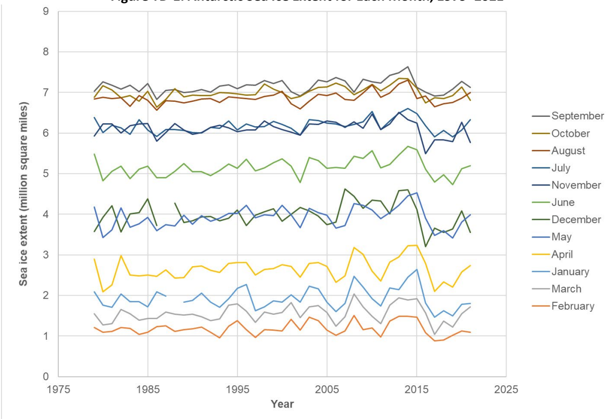
Figure TD-1. Antarctic Sea Ice Extent for Each Month, 1979–2021
