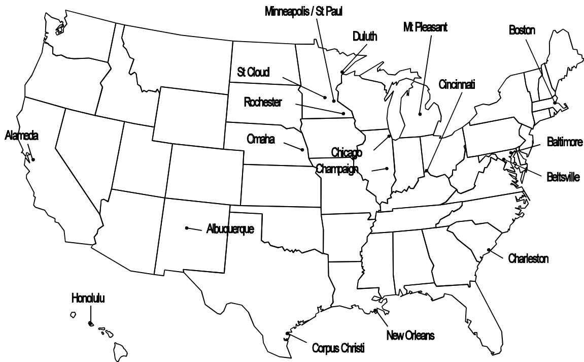
Figure 4-8. Locations of Studies Identified as Citing Gasoline Emissions as a Source of Soil Lead.
