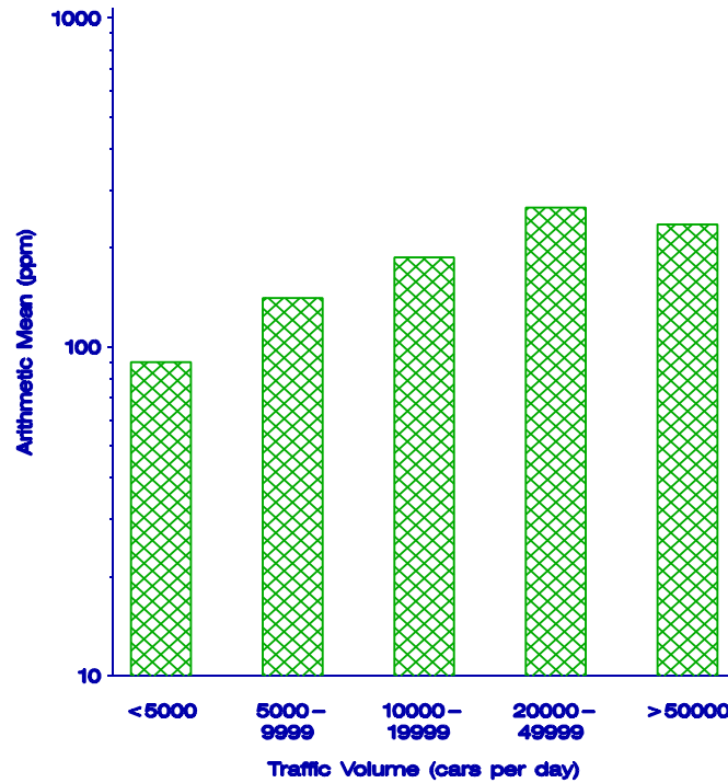
Figure 4-10. Arithmetic Means of Soil Lead Concentrations by Traffic Volume as Reported in the Illinois Soil Lead Study.
