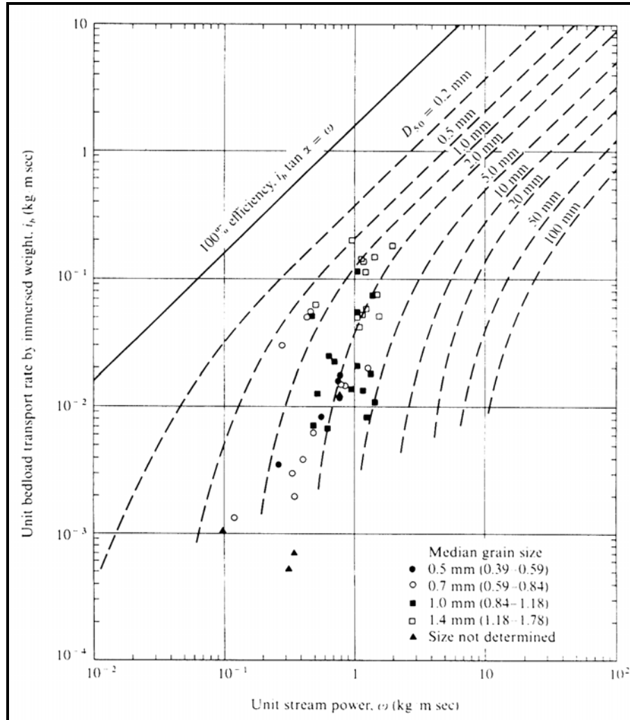
Figure 10. Relation of bedload transport rate per unit width to streampower per unit width, the family of curves being the D_{50} for the moving load. Plotted points are bedload measurements at the East Fork bed-load trap, Wyoming. (from Leopold and Emmett 1976, in Dunne and Leopold 1978)
