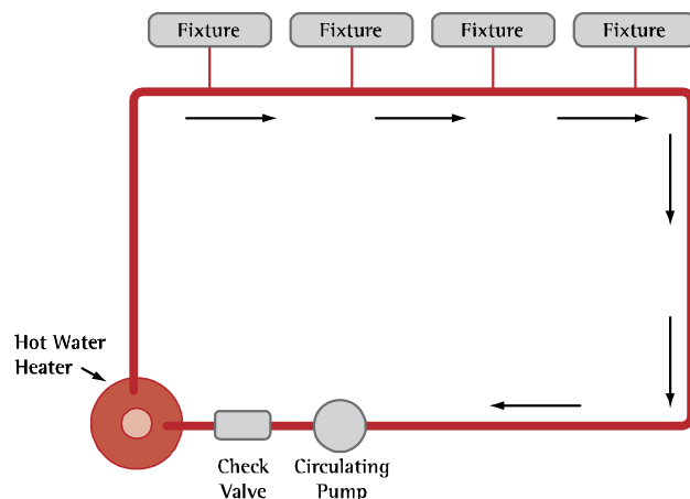
circulating System
