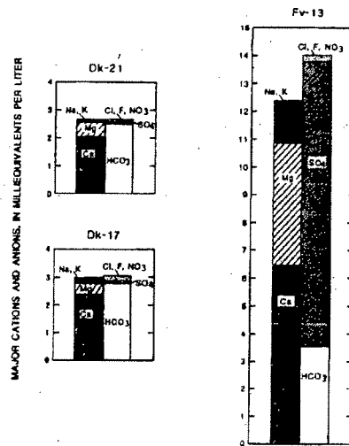
Figure 27.-- Comparison of major cations and anions in wells Dk-21, Dk-17, and Fv-13
