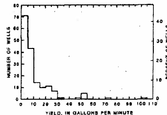
Figure 7.- Frequency distribution of reported well yields (data from Tennessee Division of Water Resources, unpublished data).
