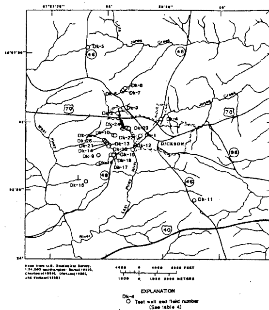
Figure 15.-- Test wells.
