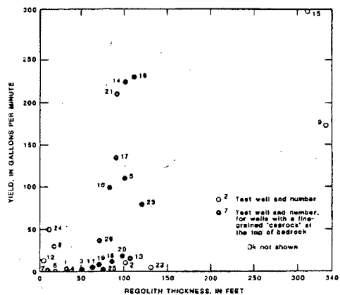
Figure 18.--Regolith thickness versus yield for test wells.
