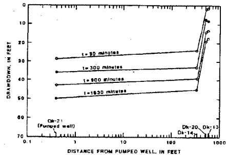
Figure 25.—Drawdown versus distance from the pumped well for the test of Dk-21.
