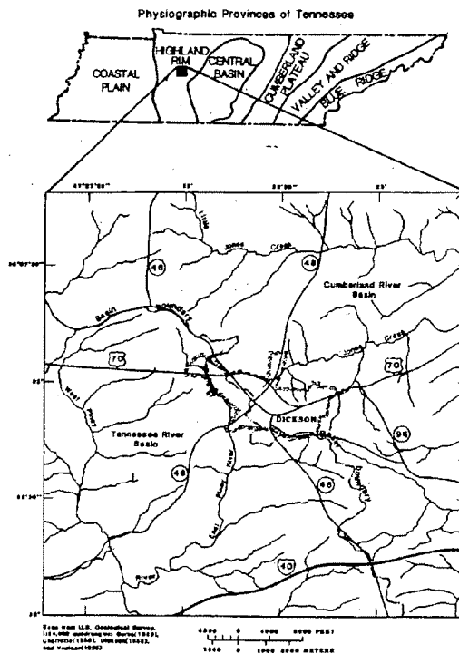
FIGURE 1.—Location of the Dickson area, Tennessee.
