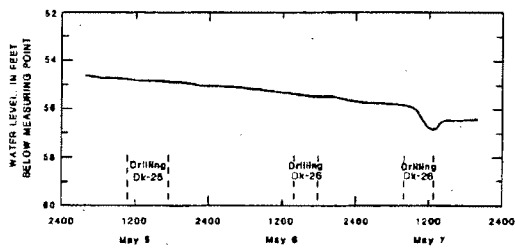
Figure 26.-- Hydrograph for well Dk-14 during May 4-7, 1961.
