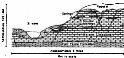
Figure 6.- Concept of ground-water occurrence and flow in the Dickson area.
