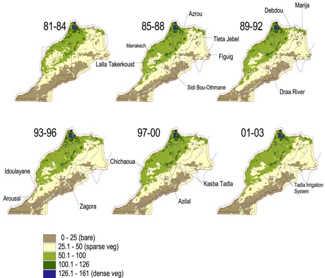
Figure 2. Average NDVI across Morocco for each 4-year temporal group. The marked circle and rectangle designate specific areas discussed in text. (data source: United States Geological Survey; http://earlywarning.usgs.gov/adds/imgbulks3.php?imgtype=nd&spextent=a ). Within the rectangle, a large patch of sparsely vegetated area (NDVI 25 – 50) is evident in the first four-year interval (1981 – 1984). In the next interval (1985 – 1988) it appears to have shrunk considerably, replaced on the margins with the next-higher average NDVI group. This corresponds very well to the conditions of that time, i.e., 1974 – 1984 was a period of drought throughout the inland desert areas of Morocco and the African Sahel while 1985 and 1986 had higher-than-average rainfall. Similarly, the circled area shows a patch with the lowest average NDVI in the early time intervals, which has been gradually replaced over time with the next-higher average NDVI group.
