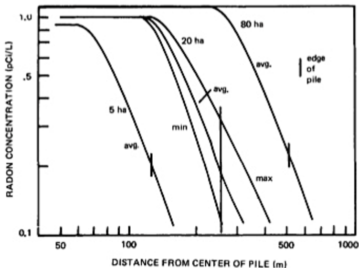
Radon Concentrations in Vicinity of Tailings from Flux of 20 pCi/m 2 -sec Source: US EPA 1982. Final EIS for Remedial Action Standards for Inactive Uranium Processing Sites
