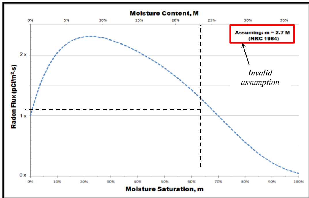
Figure 15: Radon Flux as a Function of Moisture Saturation and Moisture Content
