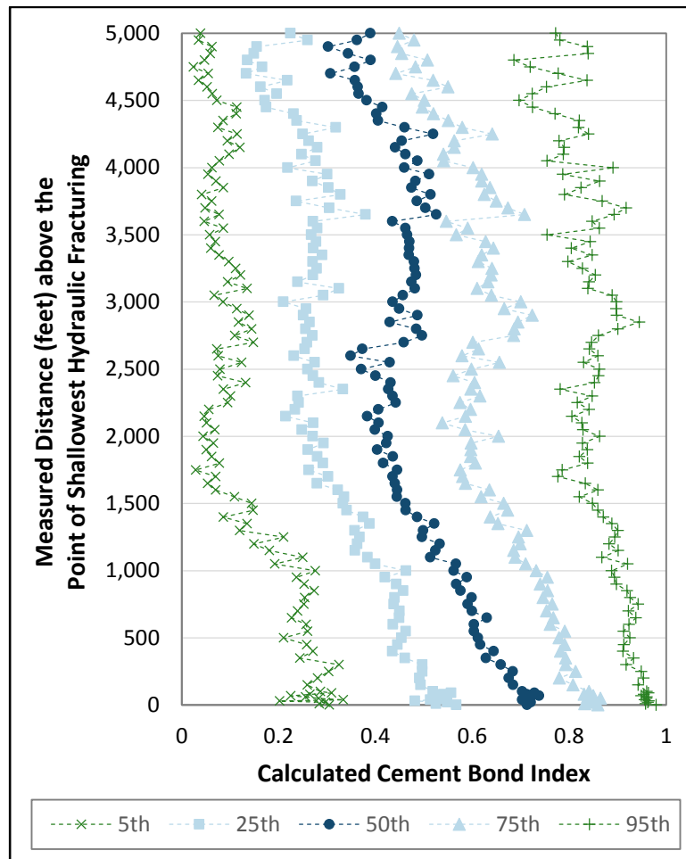
Figure 14. The 5 th , 25 th , 50 th , 75 th , and 95 th percentiles of cement bond indices calculated from standard acoustic cement bond logs.
