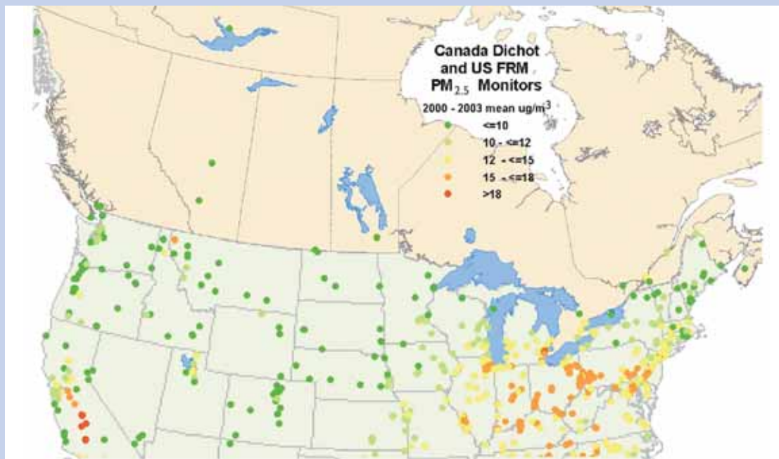
Figure A-1 Mean PM 2.5 Concentrations ( \mu\text{g}/\text{m}^3 ) at Canadian Dichotomous Monitors and U.S. Federal Reference Monitors in the Border Region, 2000-2003
