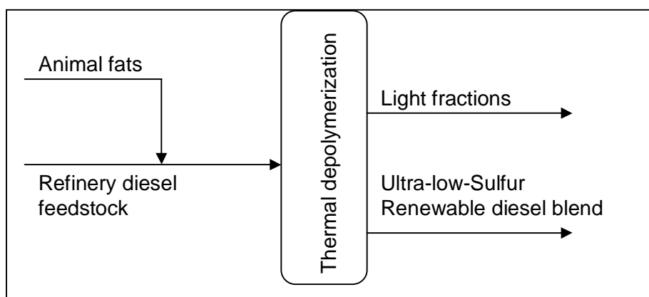
Exhibit 16: Renewable Diesel Co-processing By Thermal Depolymerization
