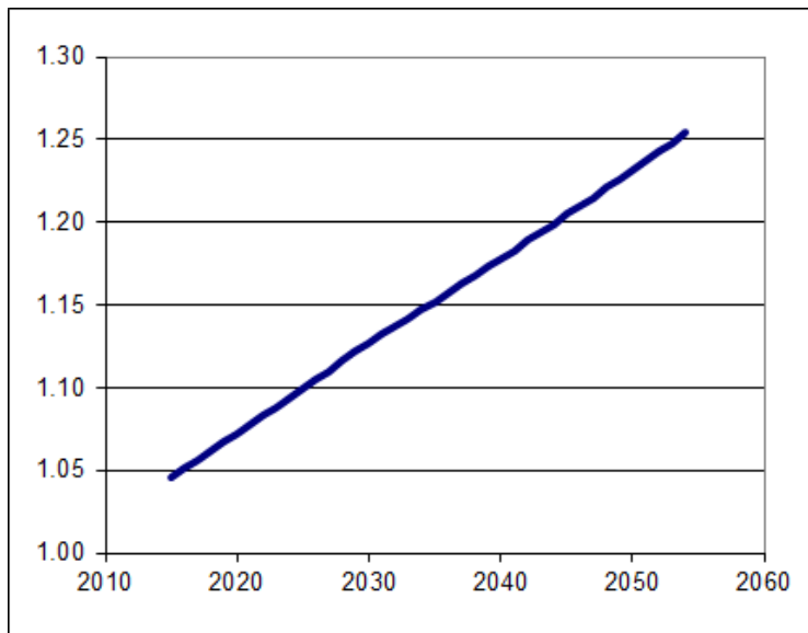
Figure 10-19 Pipeline Cost Growth Factor
