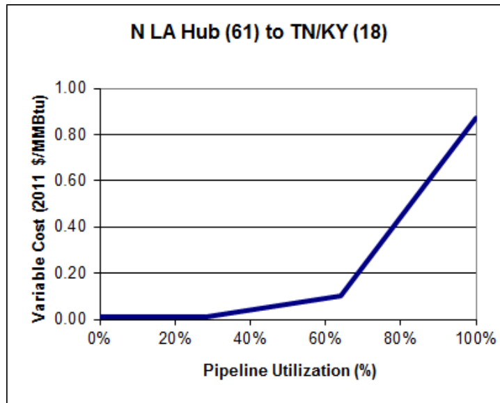
Figure 10-18 Example Pipeline Discount Curve
