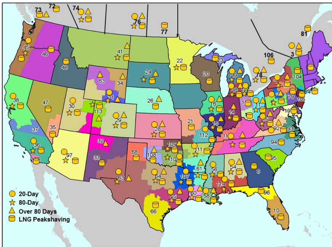
Figure 10-6 Natural Gas Storage Facility Node Map
