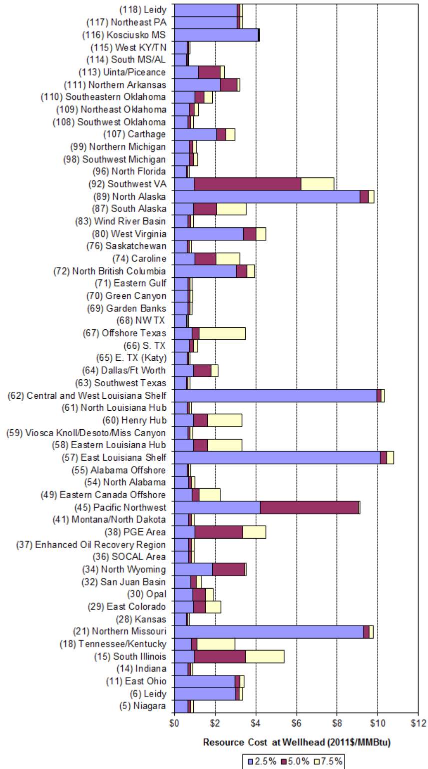
Figure 10-10 Incremental E&D Cost (BOY 2015) by Percentage of Dry Gas Resource Found
