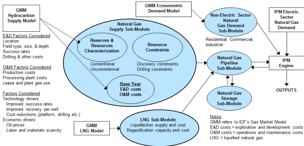
Figure 10-2 Natural Gas Module in EPA Base Case v.5.13
