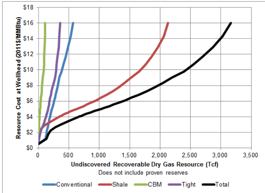
Figure 10-7 Resource Cost Curves at the Beginning of Year 2015
