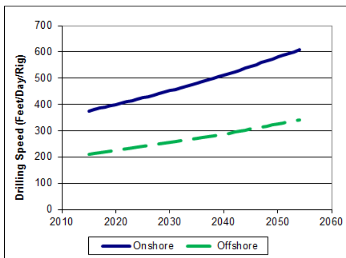
Figure 10-11 Drilling Rig Speed Constraint
