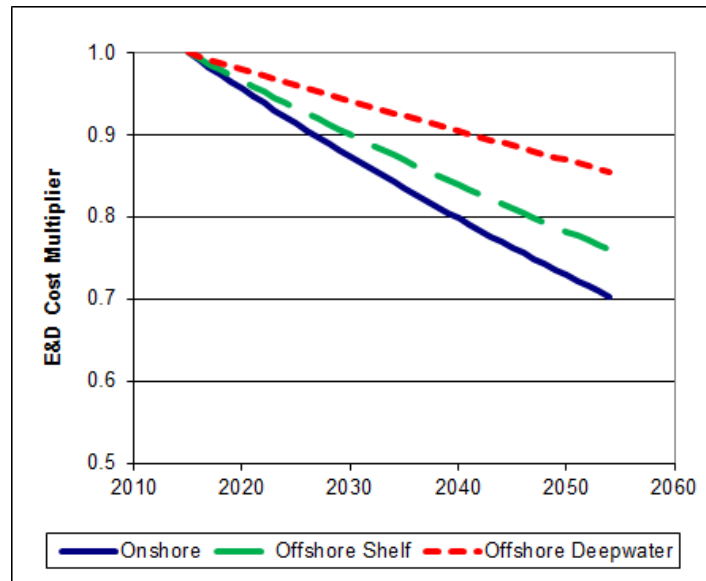
Figure 10-9 E&D and Production Technology Improvement Factor
