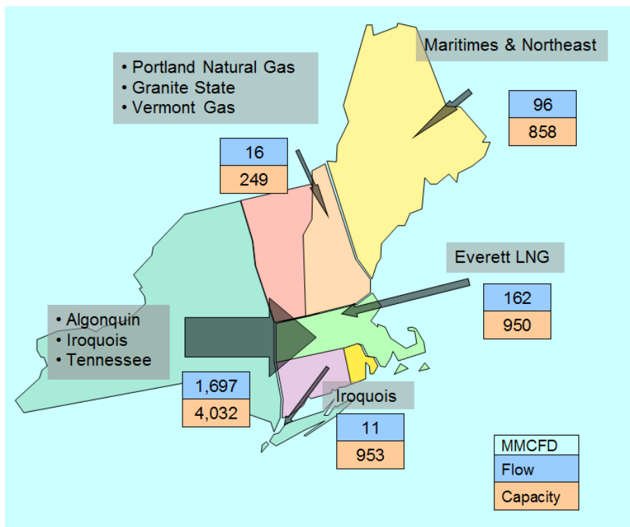
Figure 10-17 New England Pipeline Corridors in 2020
