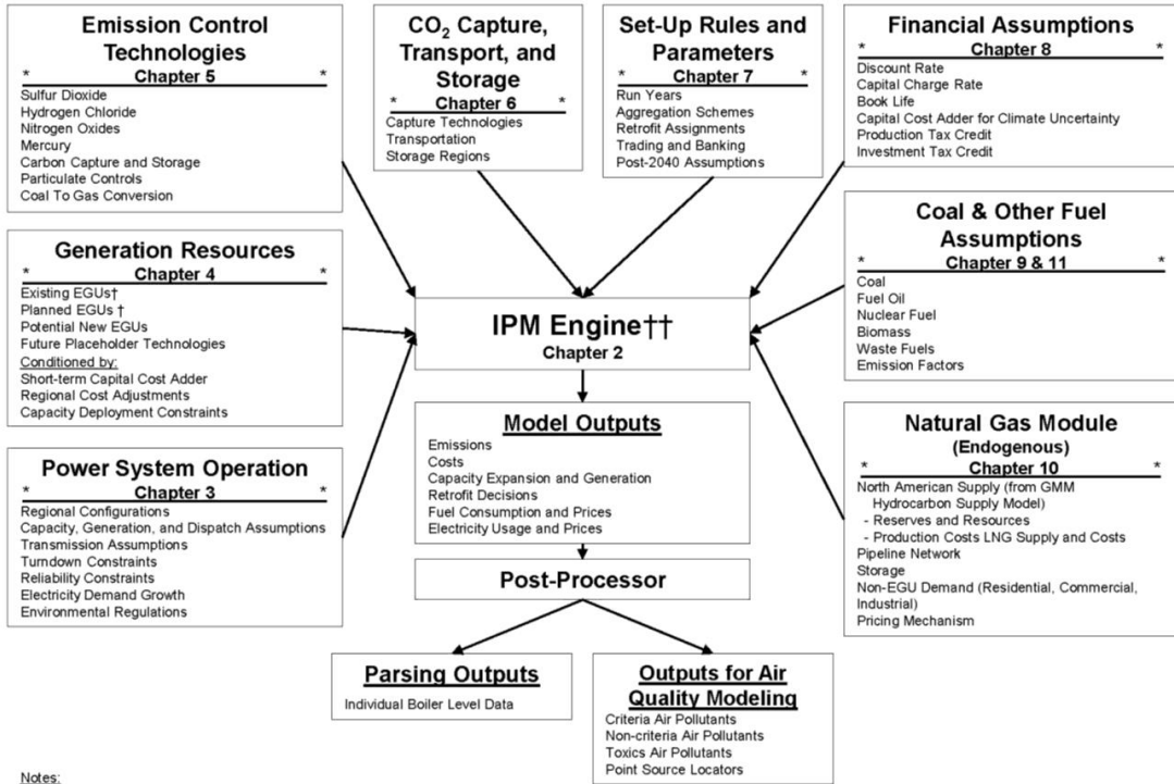
Figure 10-1 Modeling and Data Structure in EPA Base Case v.5.13
