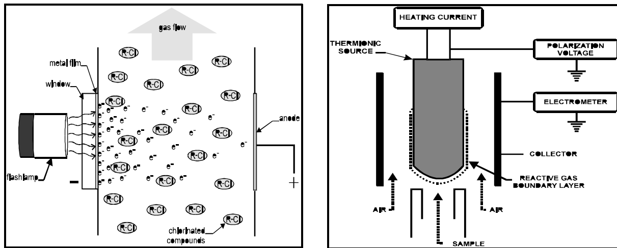
Concept graphics of the ECD (Left) and Thermionic Ionization (Right) sensors
