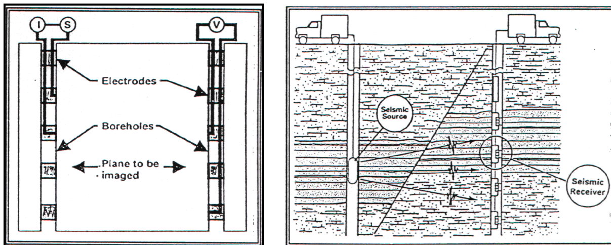
Concept drawings of the electrical resistivity (L) and seismic (R) sensor emplacements.
