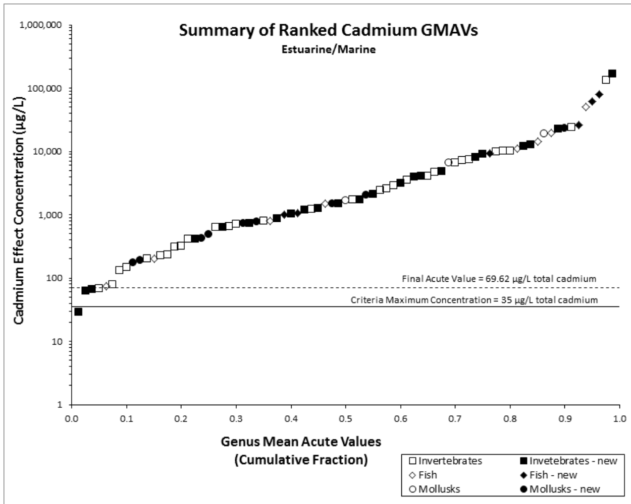
Figure 4. Ranked Estuarine/Marine Cadmium GMAVs.
