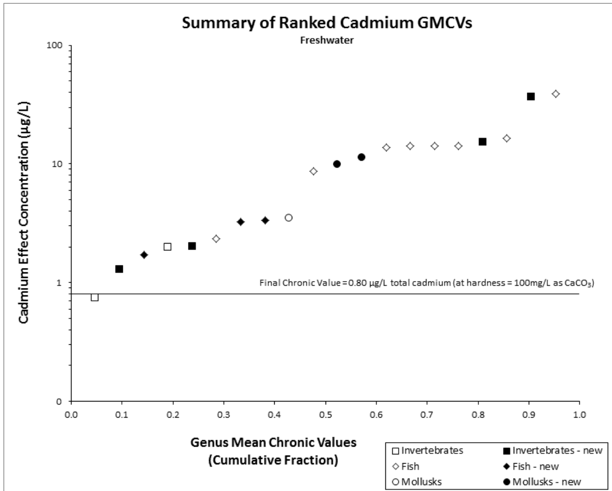
Figure 3. Ranked Freshwater Cadmium GMCVs.
