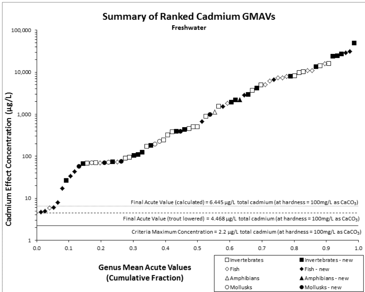
Figure 2. Ranked Freshwater Cadmium GMAVs.
