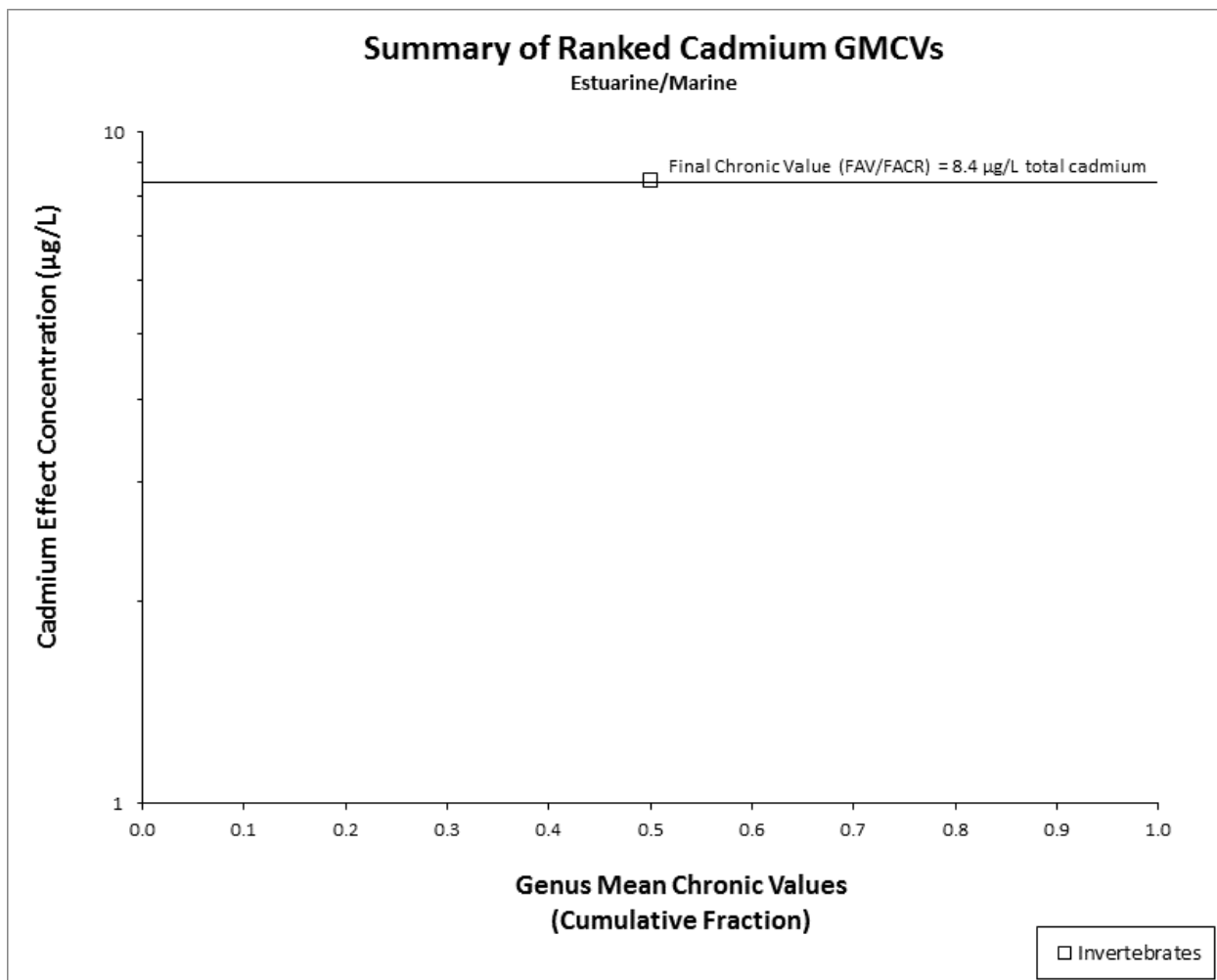
Figure 5. Ranked Estuarine/Marine Cadmium GMCVs.
