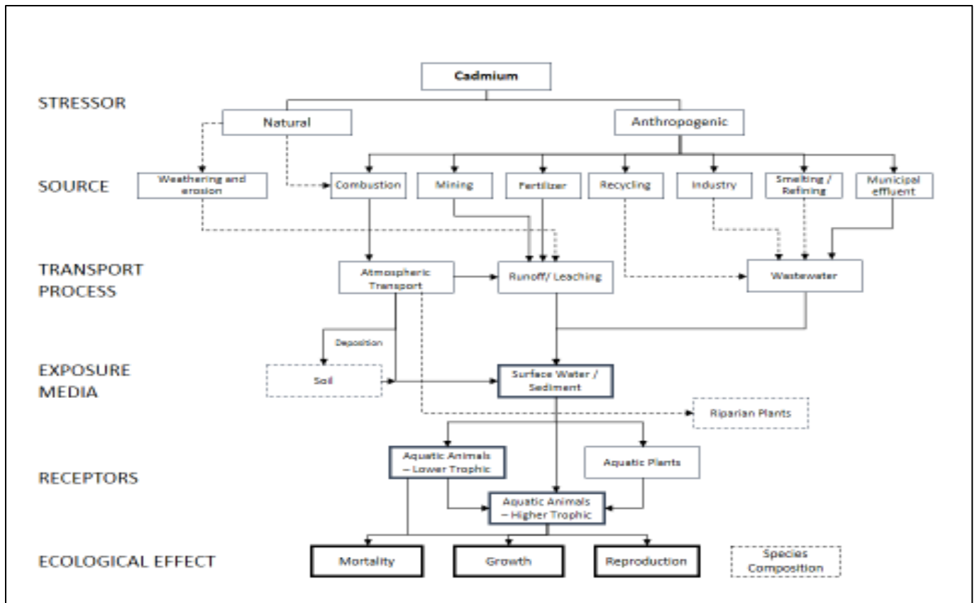
Figure 1. Conceptual Model Depicting the Major Sources, Transport and Exposure Media and Ecological Effects of Cadmium in the Environment.
