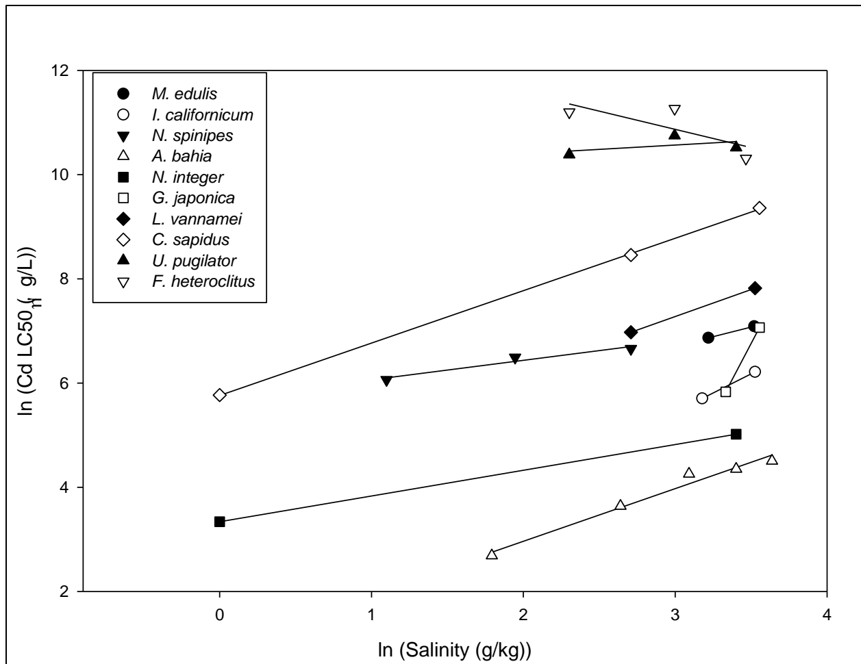
Figure 6. Individual Species Slopes Showing the Relationship between Natural Log Transformed Salinity and Natural Log Transformed Acute Cadmium Toxicity.
