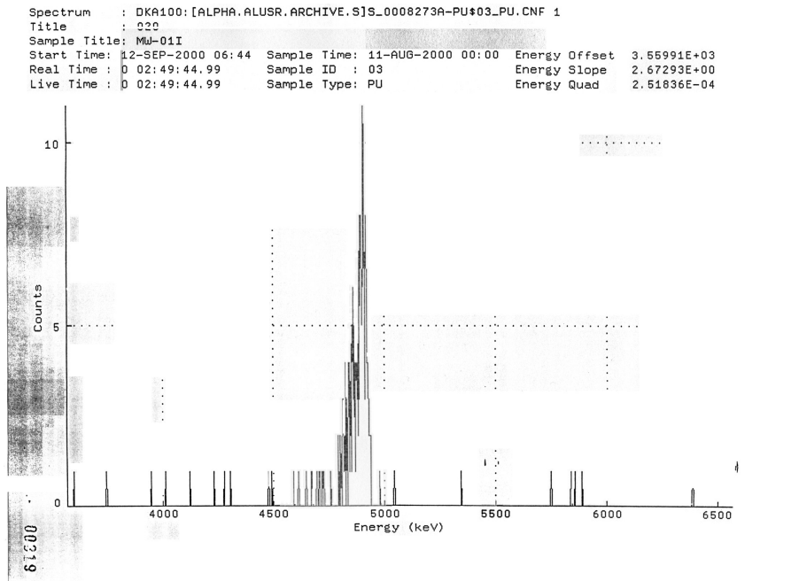
Figure 2. Alpha spectrum of groundwater sample MW-01I (August 2000) showing yield tracer peak Pu-242.
