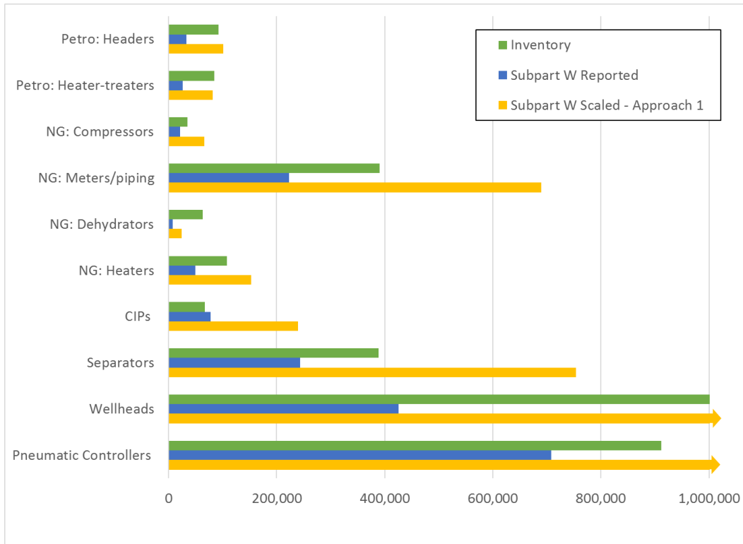
Figure 1. Subpart W Production Segment Major Equipment Counts Scaled to National Activity Representation for Year 2013, by Approach 1
