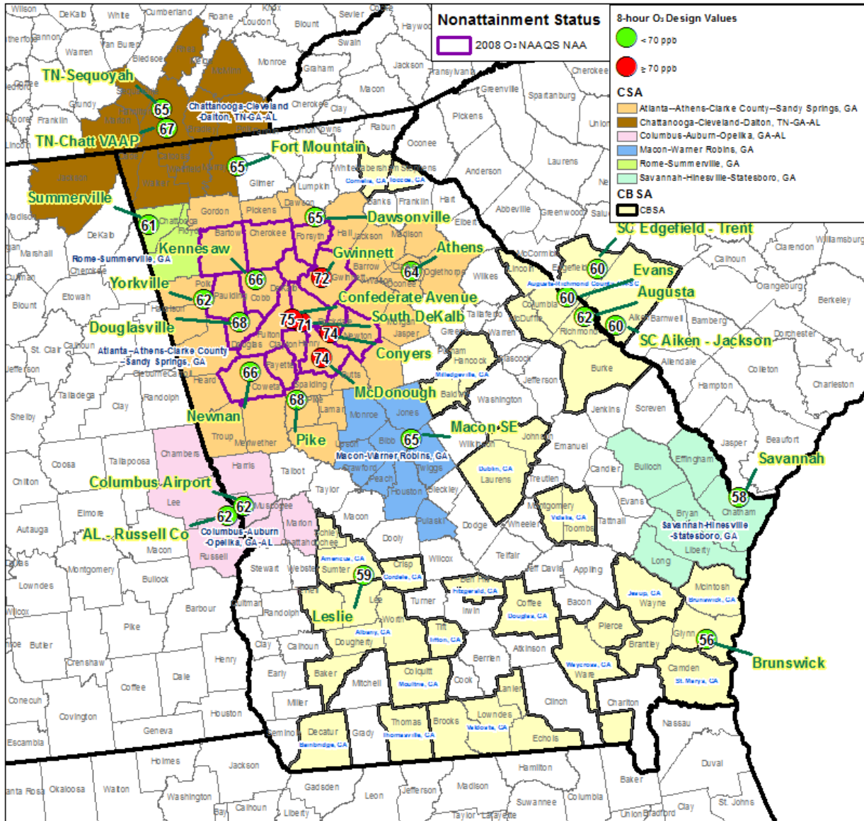
Figure 1. CSA and CBSA boundaries (CBSAs in CSAs are not shown) and preliminary 2014-2016 design values at ozone monitors in and around Georgia. Nonattainment area boundaries for the 2008 ozone NAAQS are outlined in purple.
