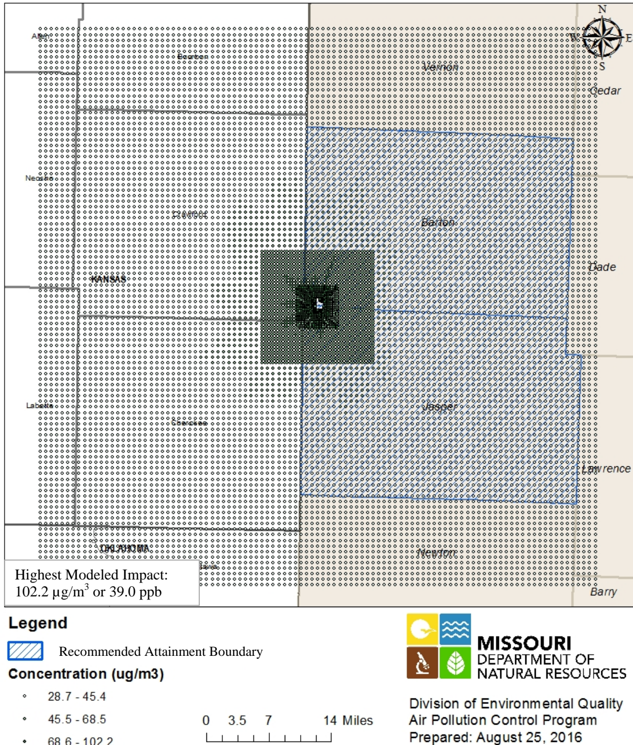
Figure 1 – Asbury Modeled SO 2 Concentrations
