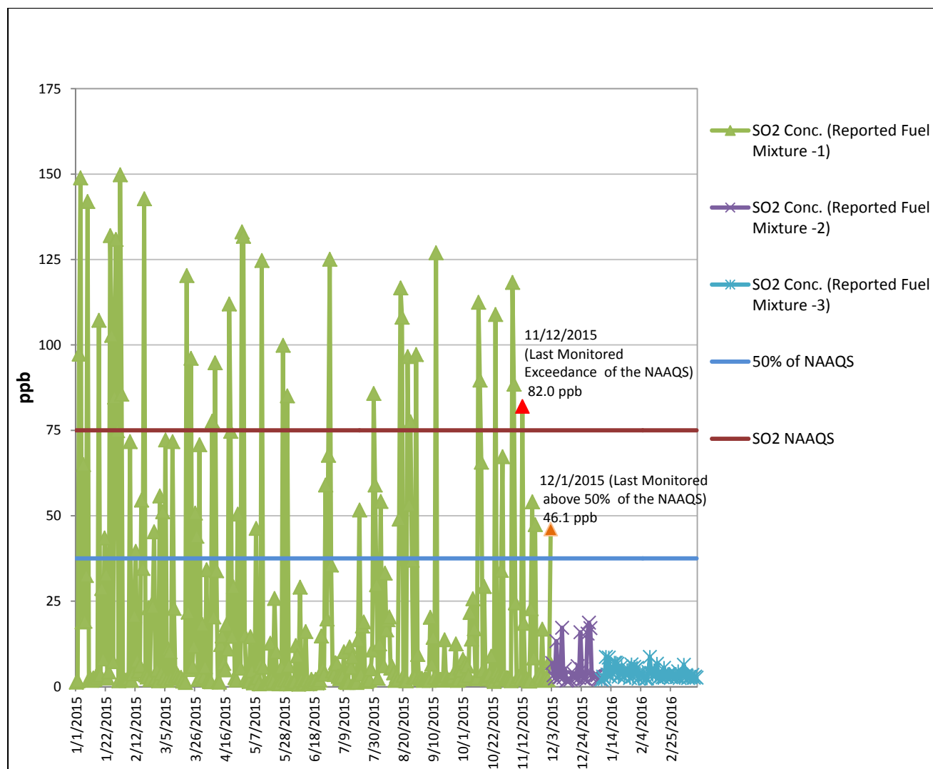
Figure 1 – Troost SO 2 Daily Maximum 1-hour Average Trend for 01/01/2015 - 03/14/2016
