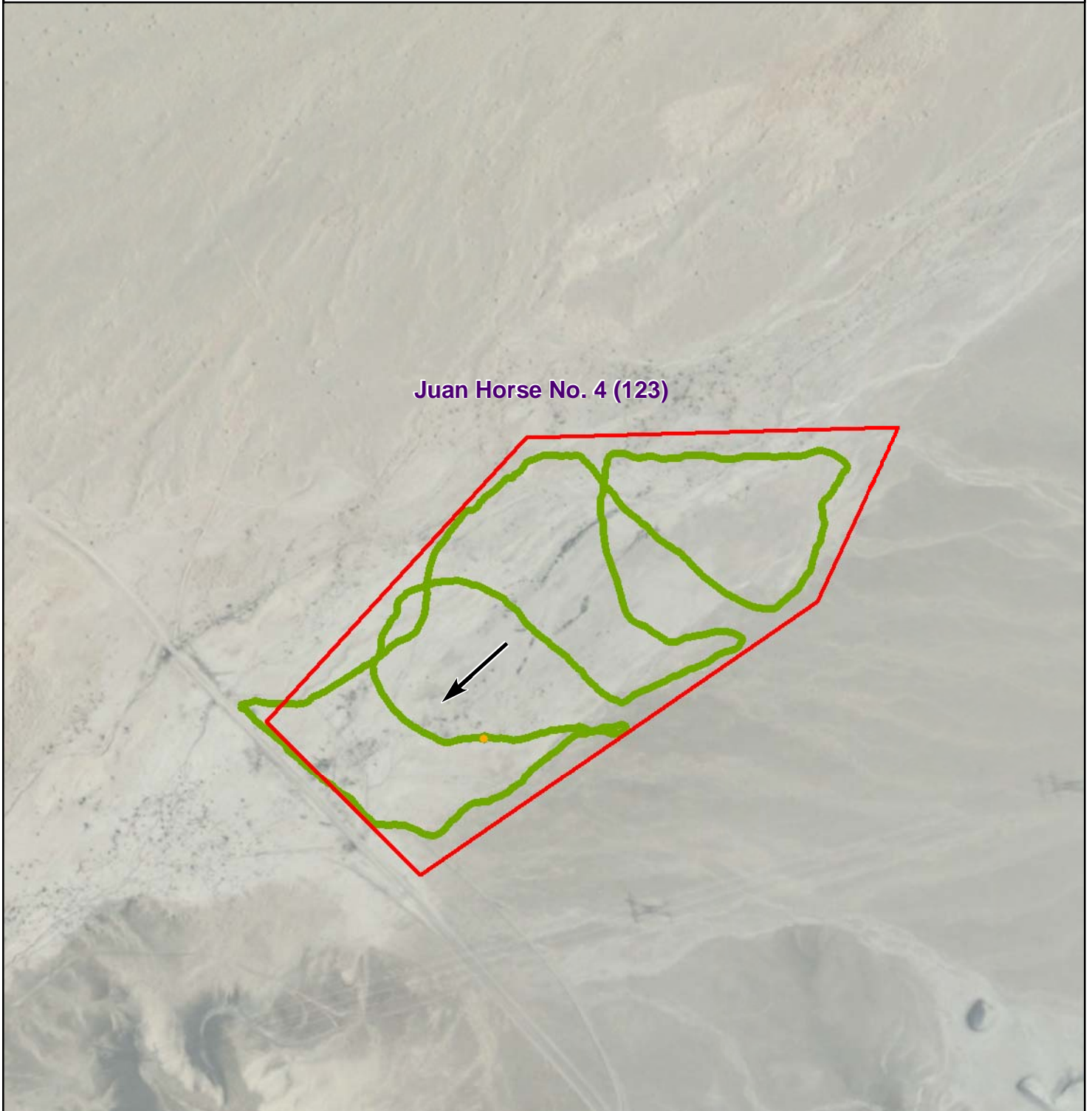
Figure 1 - Gamma Radiation Measurements, Above Two Times Background Juan Horse No. 4 (123) Coalmine Mesa Chapter, Navajo Nation
