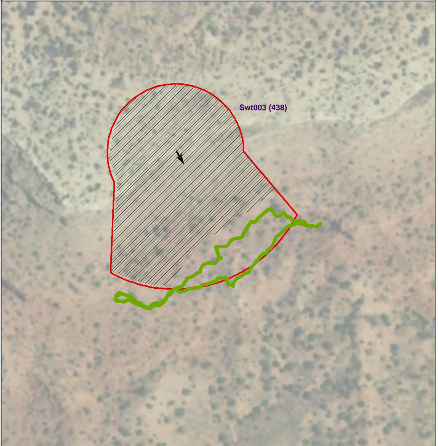
Figure 1 - Gamma Radiation Measurements, Above Two Times Background Sw003 (438) Sweetwater Chapter, Navajo Nation
