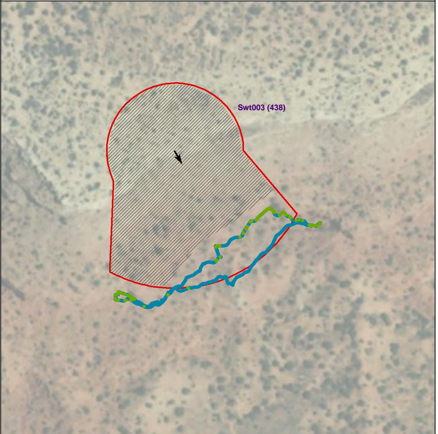
Figure 2 - Gamma Radiation Measurements Swt003 (438) Sweetwater Chapter, Navajo Nation
