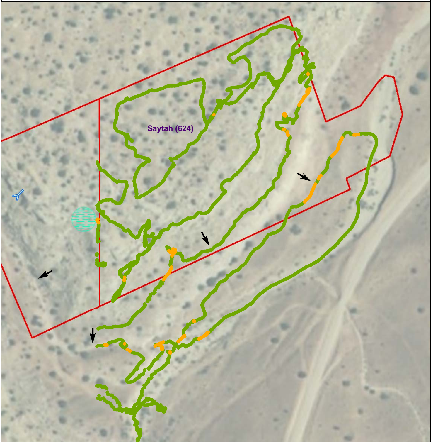
Figure 1 - Gamma Radiation Measurements, Above Two Times Background Saytah (624) Sweetwater / Teec Nos Pos Chapter, Navajo Nation
