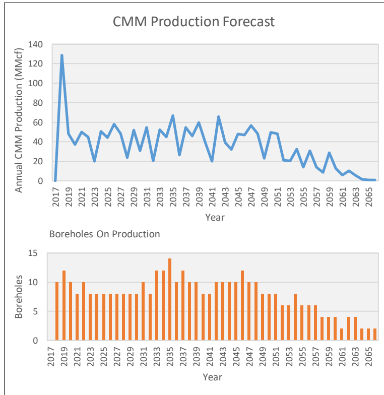
Exhibit 39: CMM Production Forecast for San Juaquin Mine
