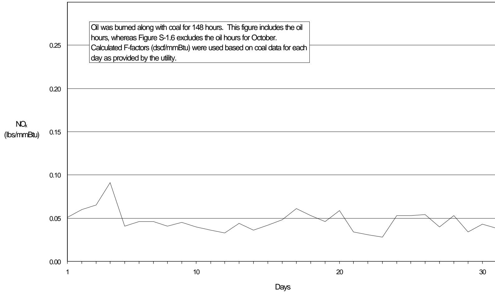
Figure S-1.5 Plant S-1: NO x Emissions Including Oil Hours (24 Hour Averages) October 1-31, 1995
