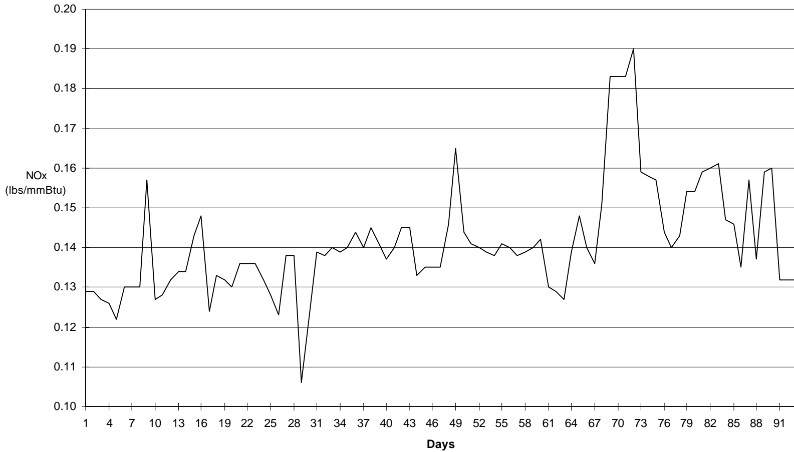
Figure US-4.2 Plant US-4: NO x Emissions (24-Hour Averages)
