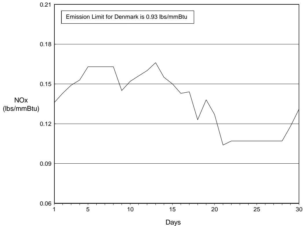
Figure 6.8. \text{NO}_x Emissions (24-Hour Averages) for Danish Plant D-1
