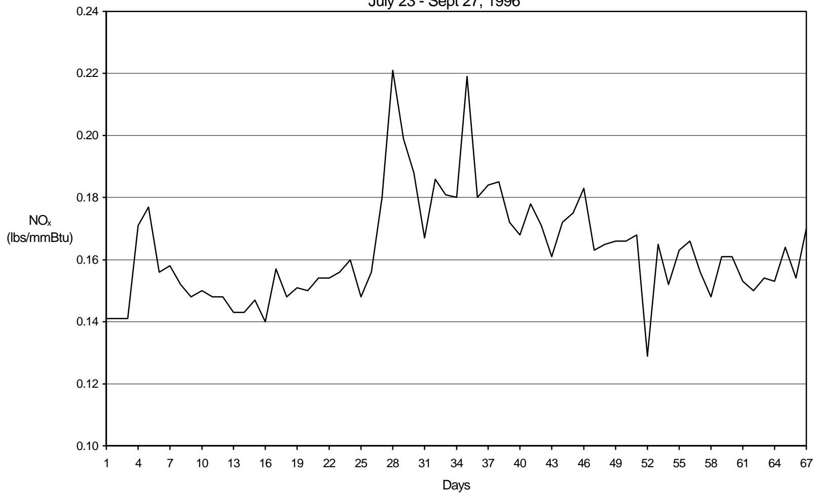
Figure F-1.2 Plant F-1: NO x Emissions (24-Hour Averages)
