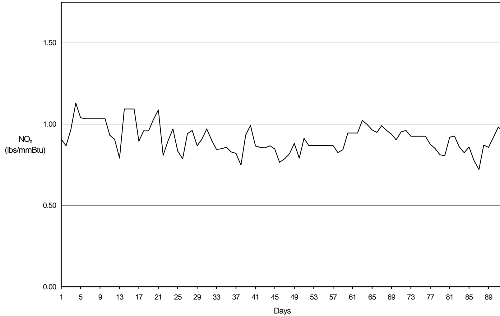
Figure US-6.2 Plant US-6: NO x Emissions (24-Hour Averages)
