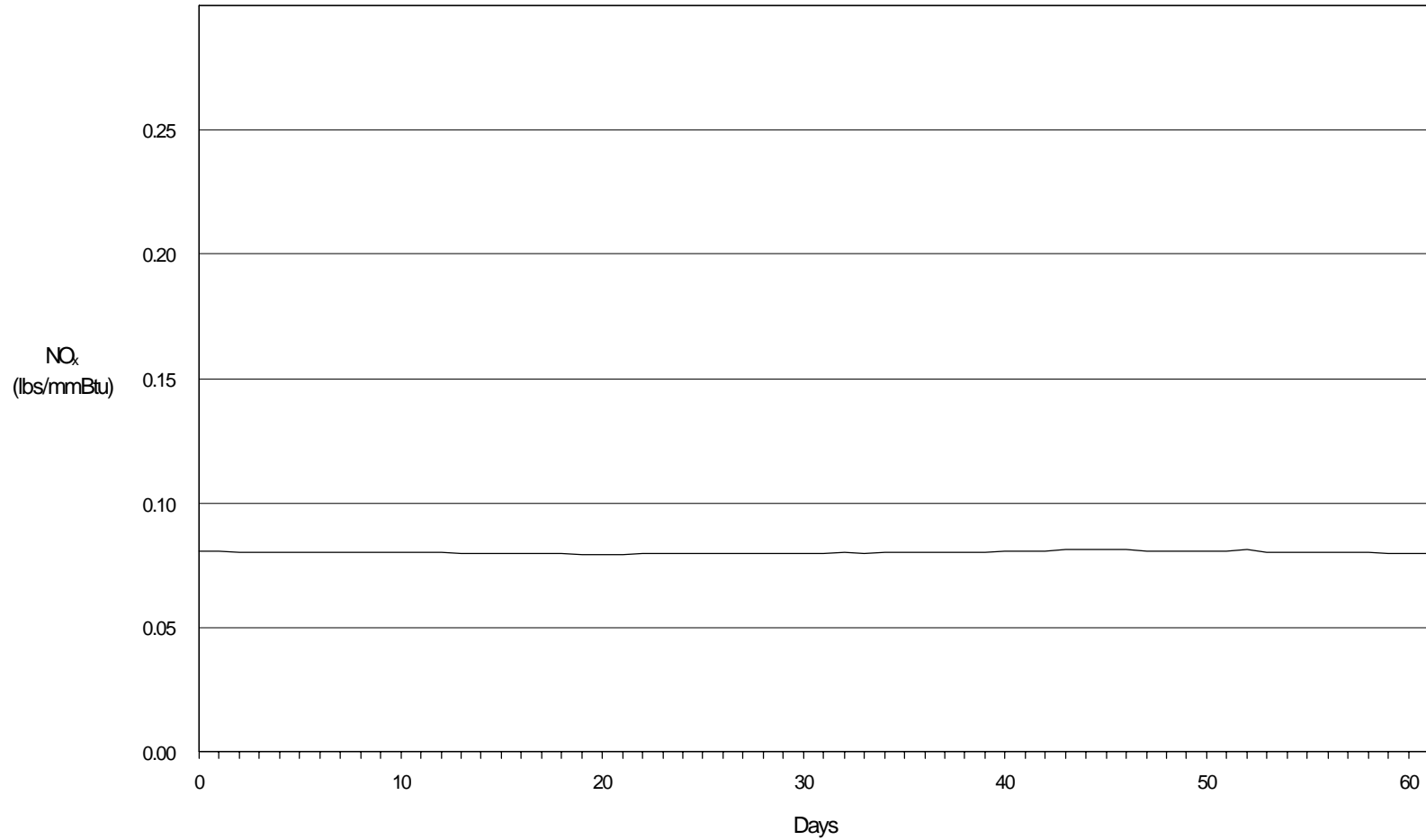
Figure G-4.5 Plant G-4: NO x Emissions (Unit A: 30 Day Rolling Averages) January 1 - March 31, 1996
