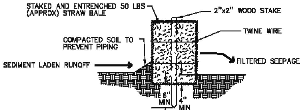
CROSS-SECTION OF PROPERLY INSTALLED STRAW BALE
