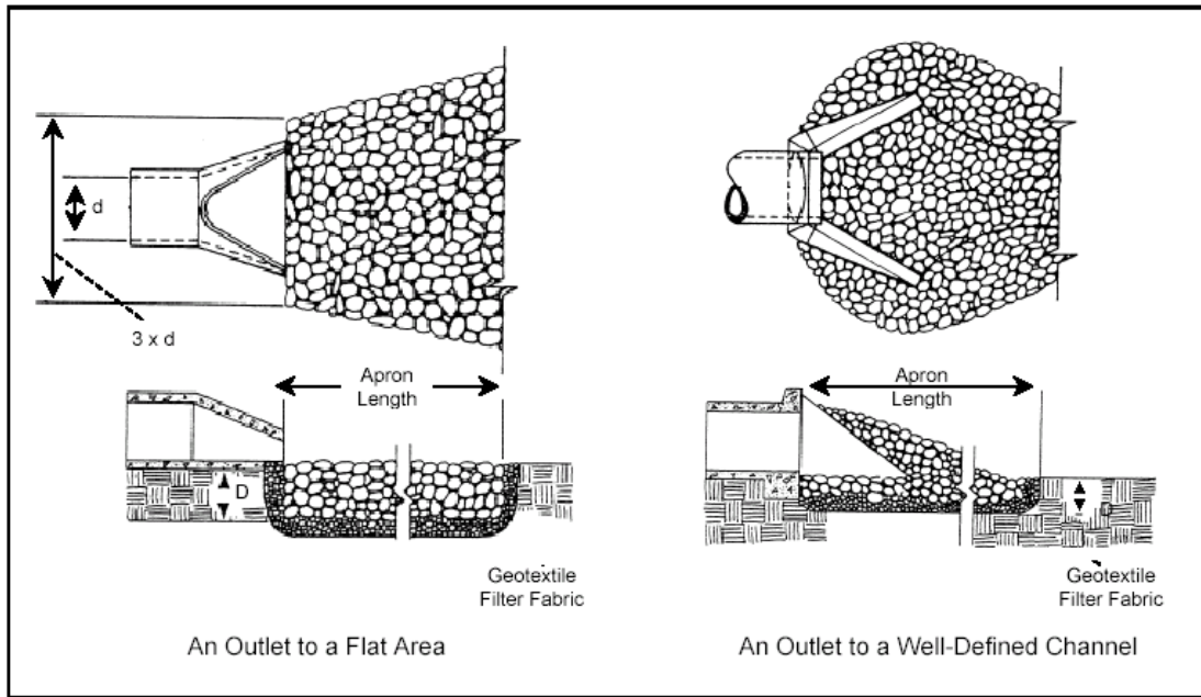
Figure 1: Rock Outlet Protection
