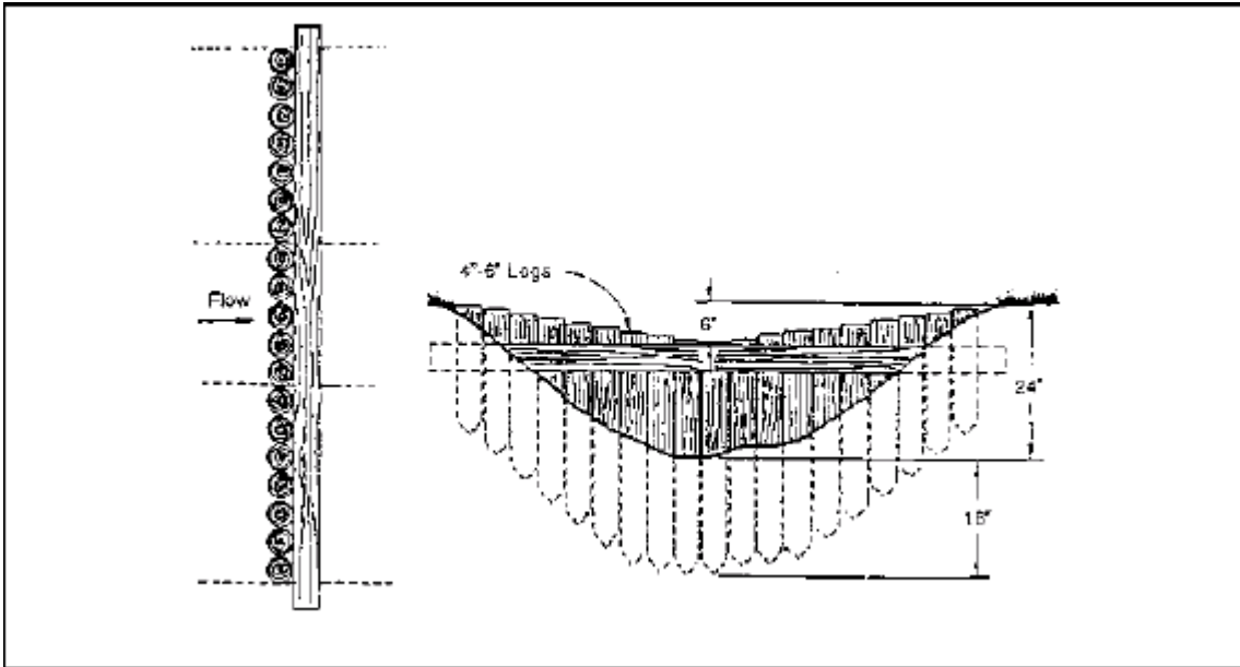
Figure 2. Log Check Dam
