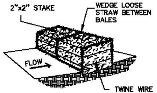
PLACE AND STAKE STRAW BALES
