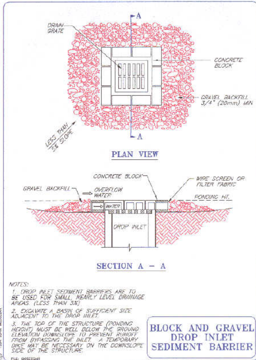
Figure 2: Block and Gravel Drop Inlet
