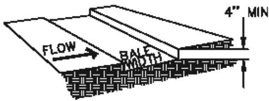
EXCAVATE TRENCH
