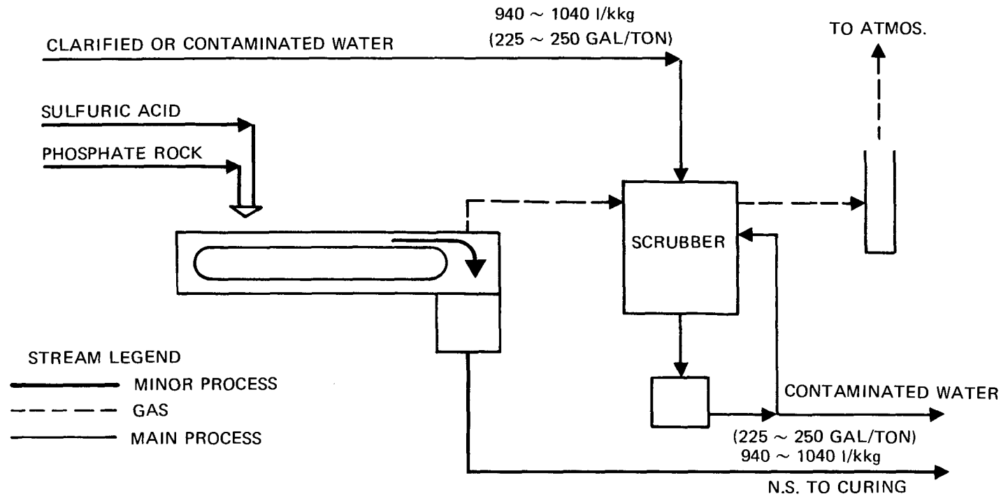
FIGURE 10 NORMAL SUPERPHOSPHATE FLOW RATE PER TON N.S.
