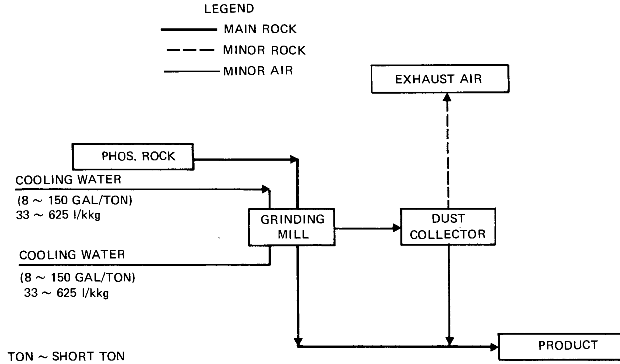
FIGURE 5 ROCK GRINDING FLOW RATE PER TON ROCK
