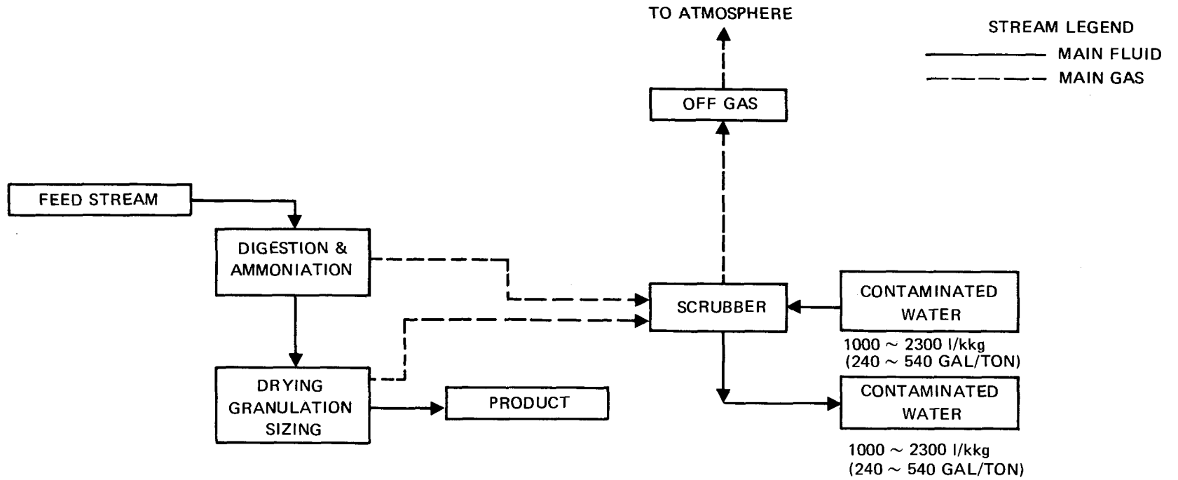
FIGURE 7 NPK PROCESS NITRIC ACID ACIDULATION FLOW RATE PER TON P 2 O 5
