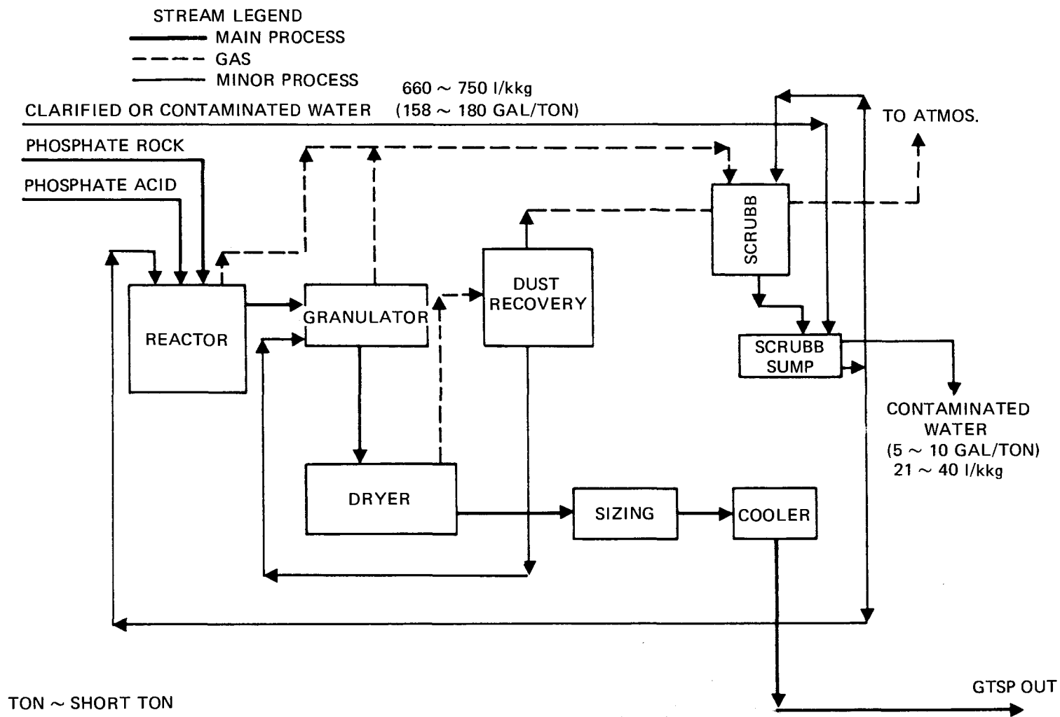
FIGURE 12 GRANULATED TRIPLE SUPER PHOSPHATE FLOW RATE PER TON GTSP
