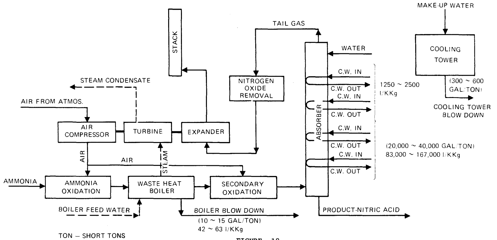
FIGURE 18 NITRIC ACID PLANT FLOW RATE PER TON 100% NITRIC ACID
