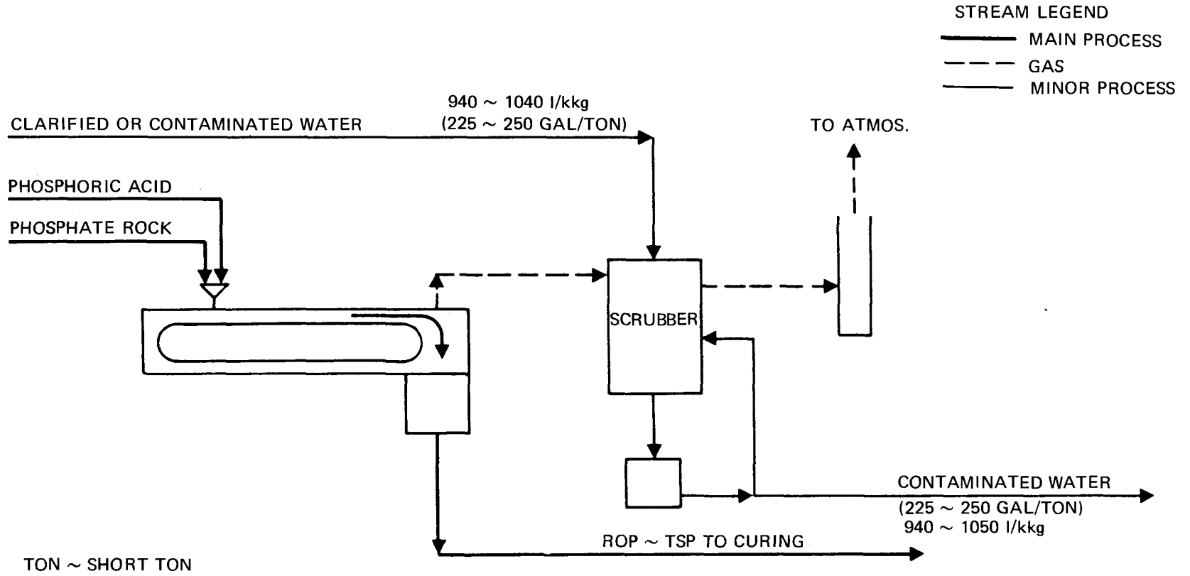
FIGURE 11 TRIPLE SUPERPHOSPHATE (RUN-OF-PILE R.O.P.) FLOW RATE PER TON ROP ~ TSP
