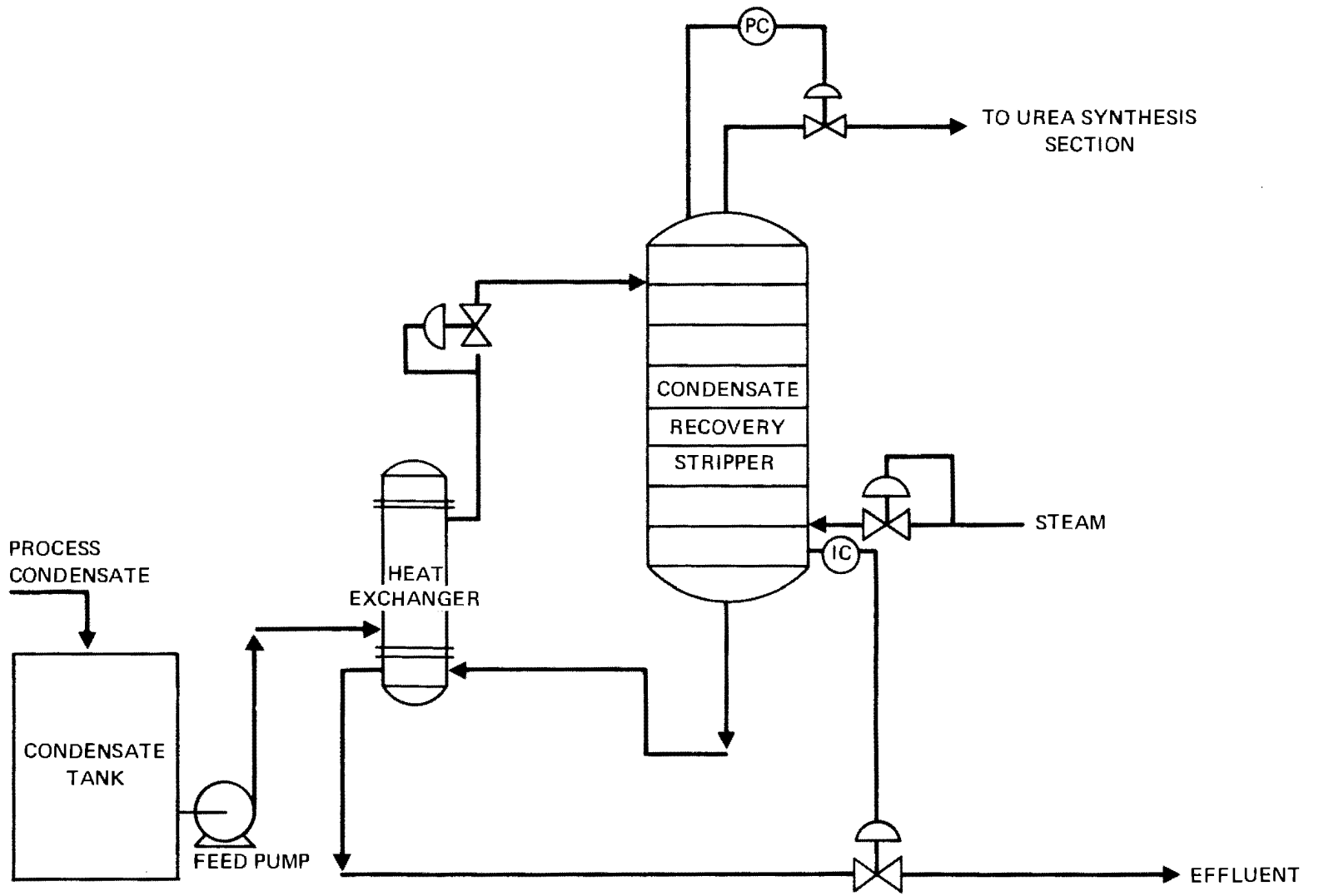
FIGURE 29 UREA HYDROLYSIS
