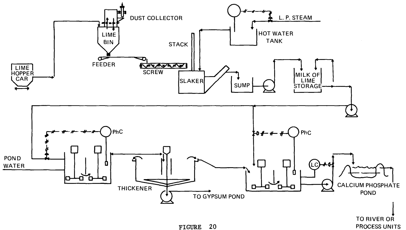
FIGURE 20 POND WATER TREATMENT
