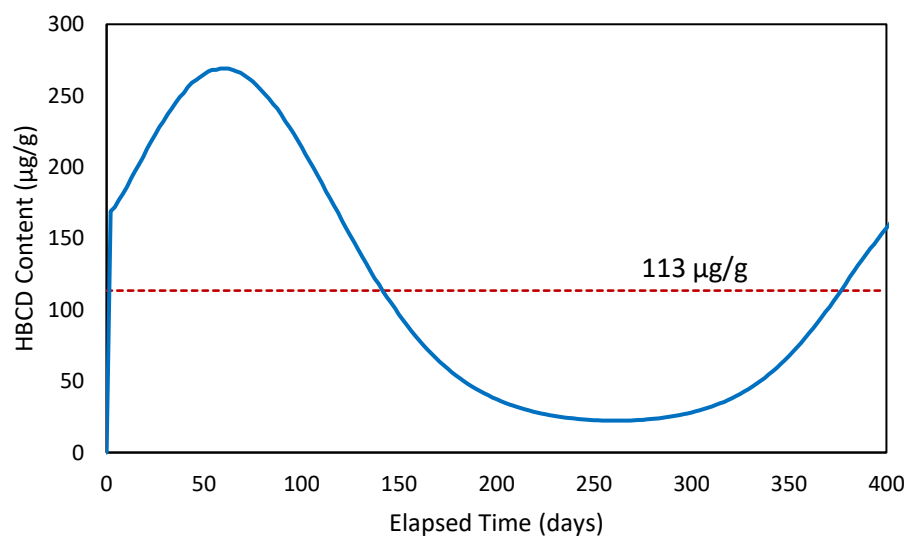
Figure Apx_ F-2. Predicted HBCD concentration in airborne PM in living area.
