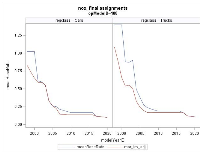
Figure 3-136 NO x : Final assignments for Federal and Estimated CA/S.177 emission rates, for cars and trucks at age 0-3 years, for the start emissions process (opModelID = 108)
