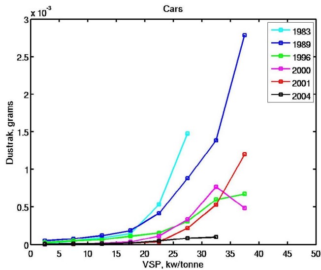
Figure 4-15 Particulate emissions, as measured by the Dustrak, averaged by VSP and model-year group (LINEAR SCALE)
