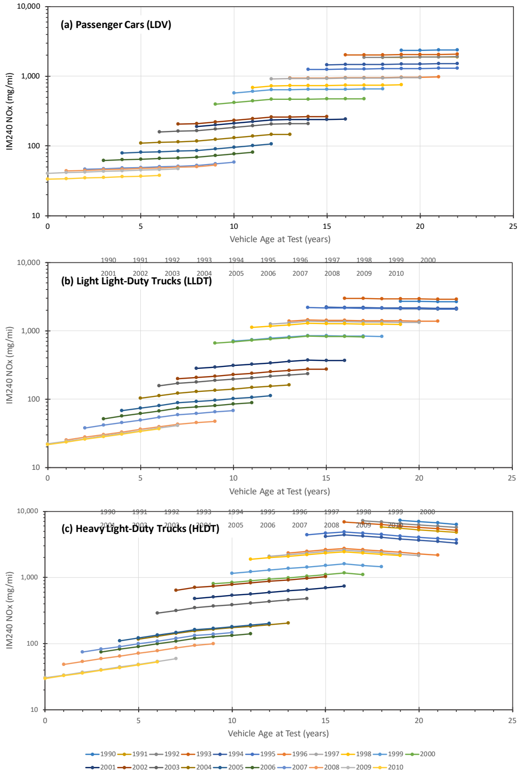
Figure 3-53 NO x : Three-piece linear spline deterioration models for three vehicle classes: (a) Passenger cars, (b) Light Light Duty Trucks, and (c) Heavy Light-Duty Trucks. Note that emissions are expressed on common logarithmic scale
