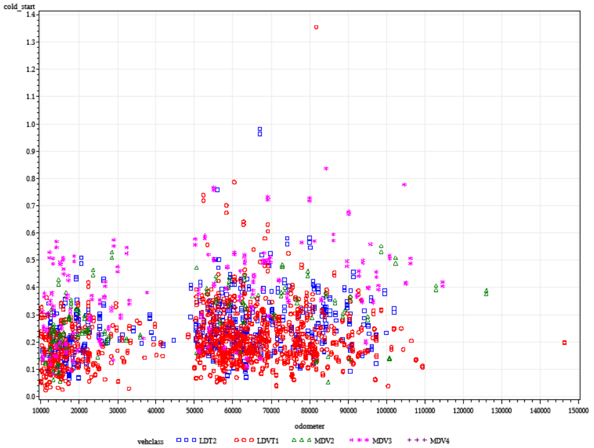
Figure 3-93 Cold-start FTP emissions for NMOG (g) vs. odometer (mi), for LEV vehicles, from the IUVF program
