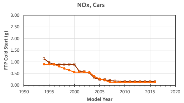
Figure 3-122 Weighted average FTP cold-start emissions, for Federal and CA/S177 standards
