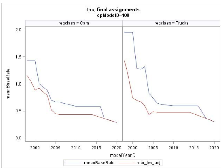
Figure 3-132 THC: Final assignments for Federal and Estimated CA/S.177 emission rates, for cars and trucks at age 0-3 years, for the start emissions process (opModelID = 108)
