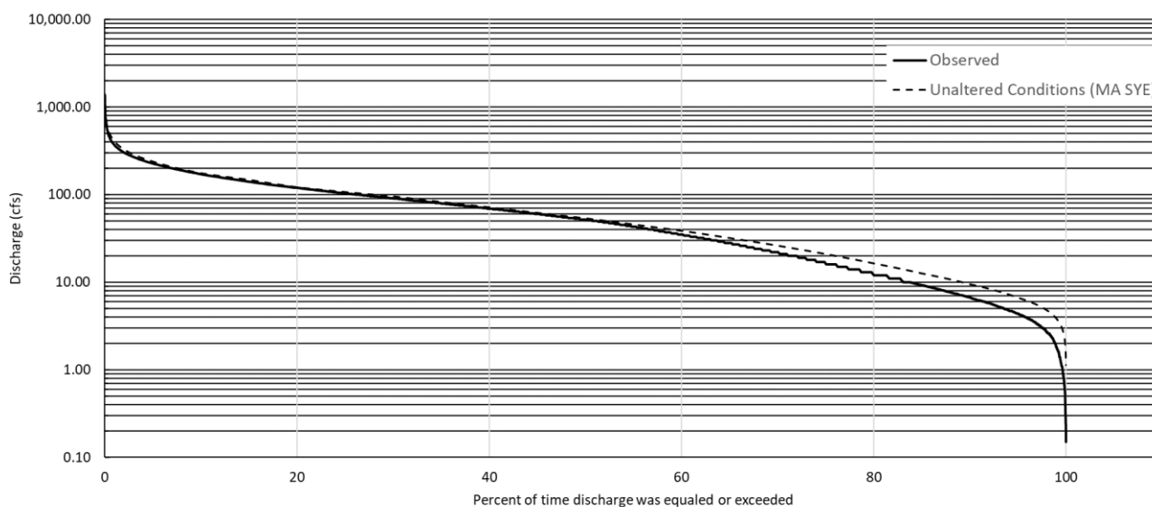
Figure 40. Observed flow duration curve for Wading River for the period of record and the estimated unaltered condition flow duration curve generated from the Massachusetts Sustainable-Yield Estimator.
