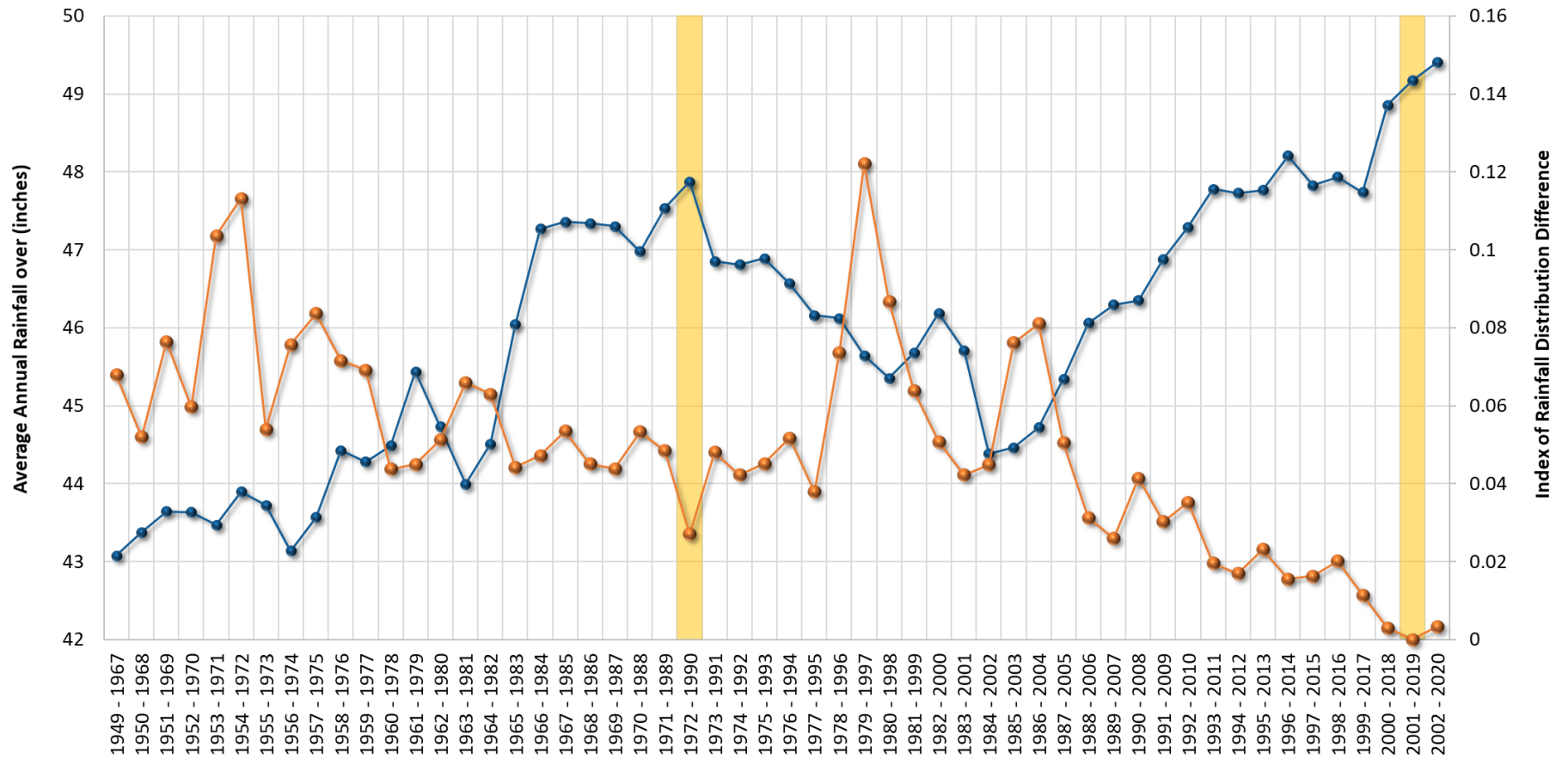
Figure 60. Average annual rainfall depth and distribution (T.F. Green Airport).
