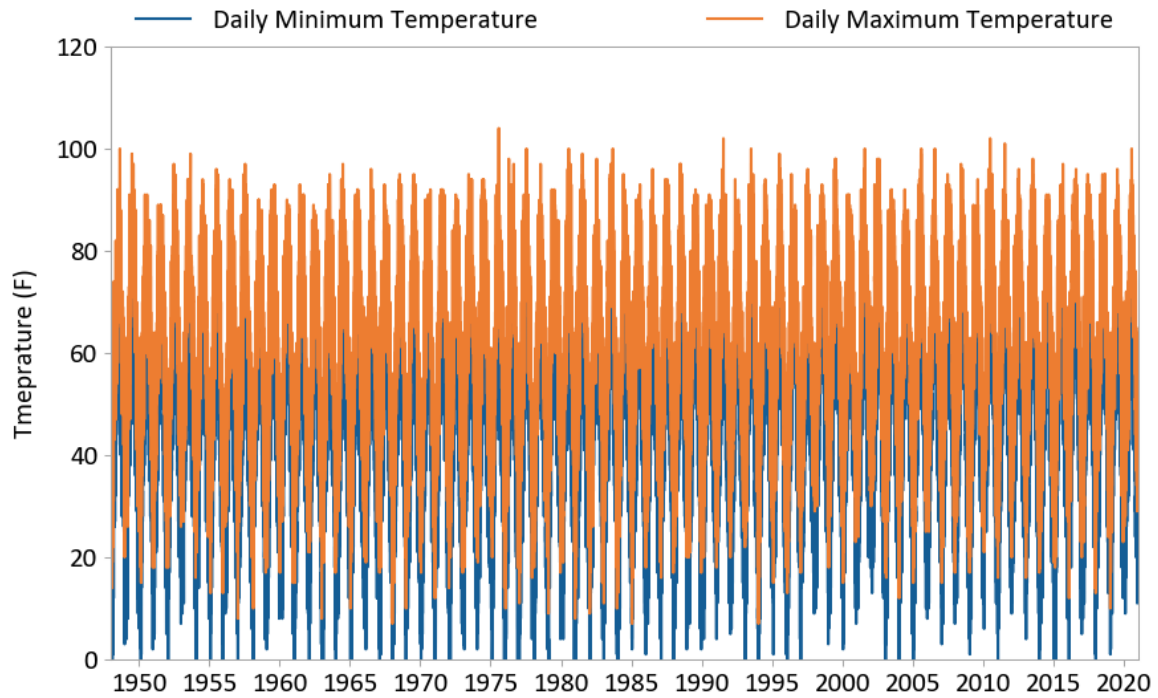
Figure 57. Daily minimum and maximum temperatures (T.F. Green Airport).
