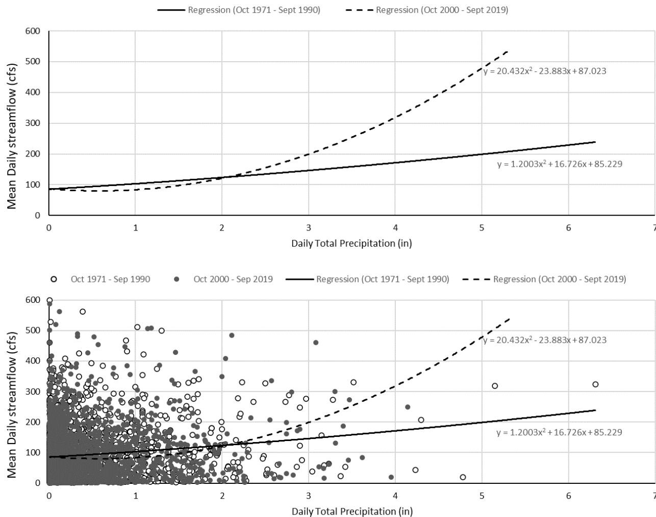
Figure 73. Streamflow versus precipitation for days with measurable precipitation. Regression only (top), regression and data (bottom).
