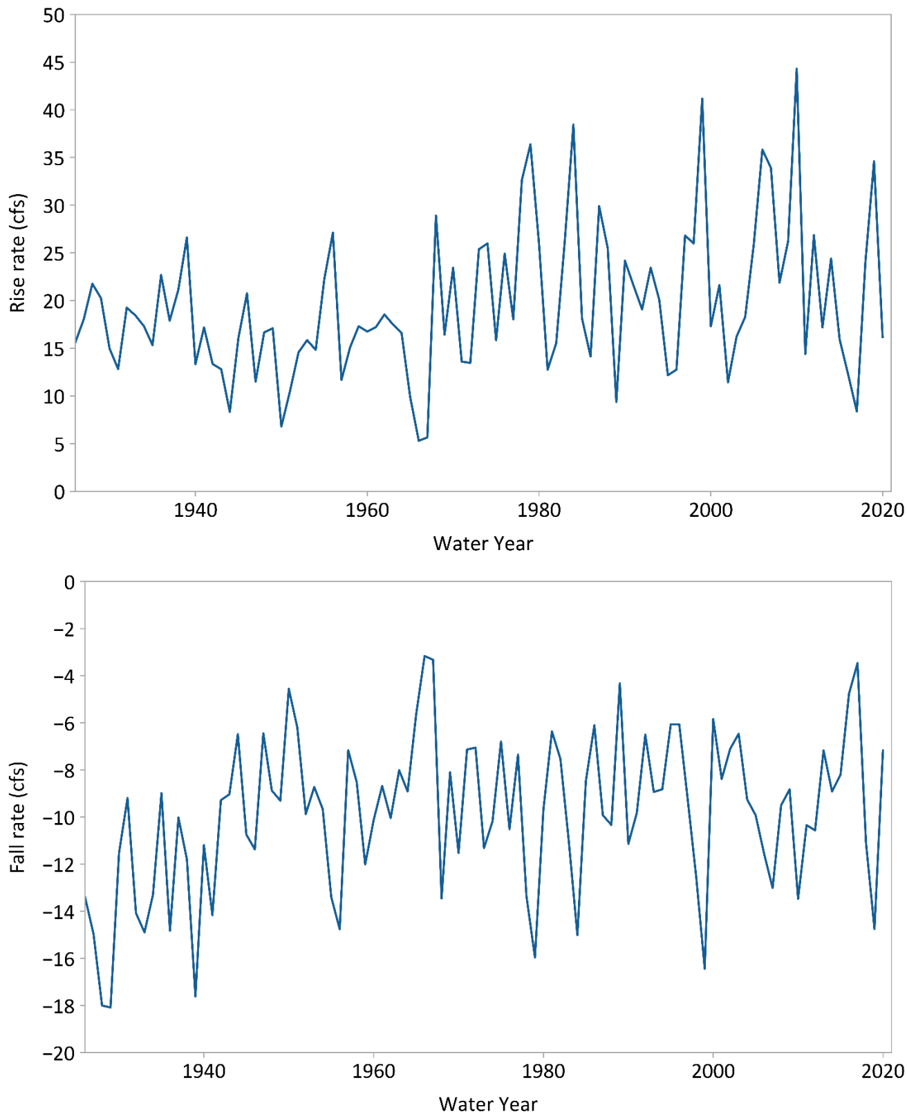
Figure 27. Rise rate (top) and fall rate (bottom).
