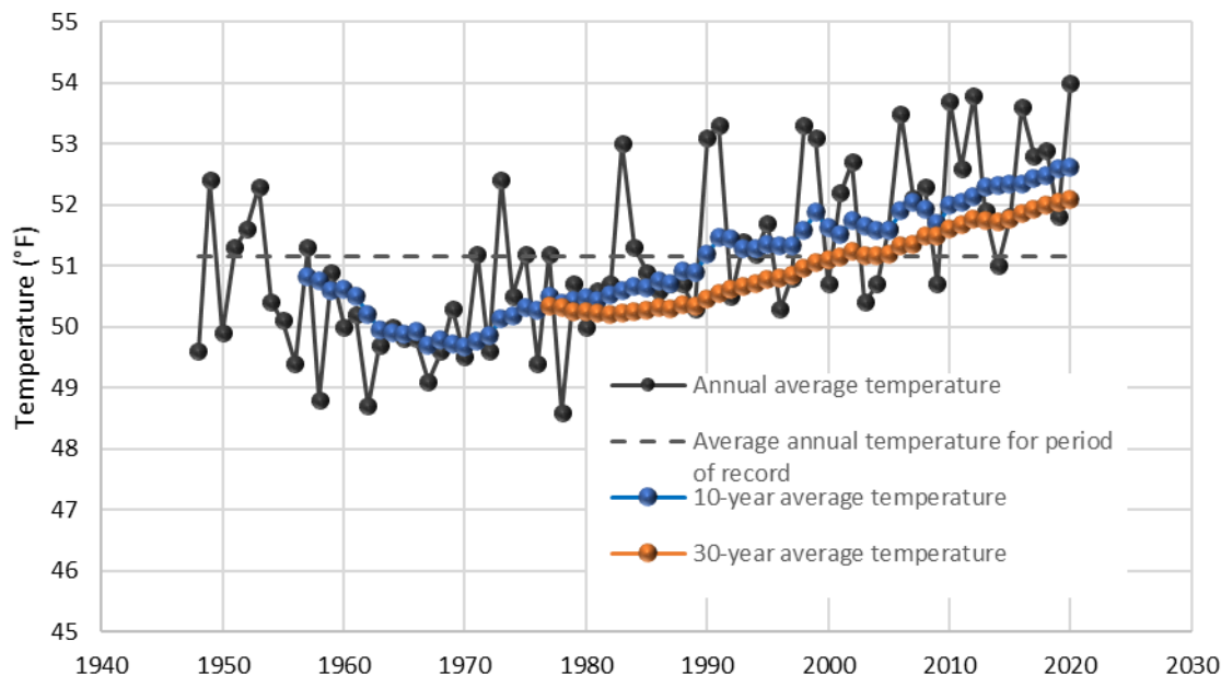
Figure 58. Annual average temperature trends (T.F. Green Airport).
