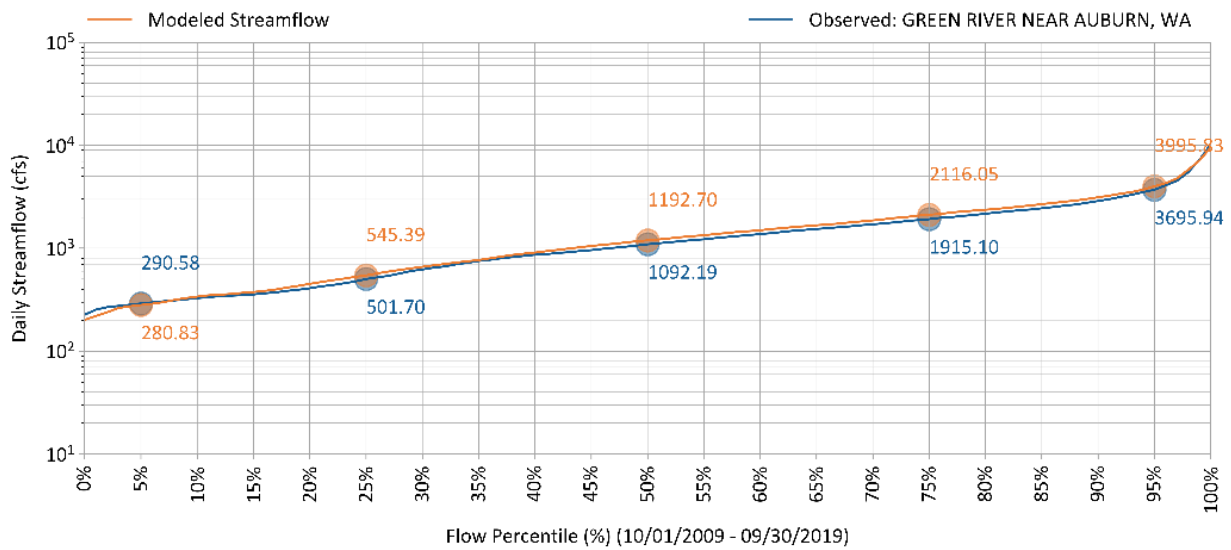
Figure 76. Example comparison of observed and predicted flow duration curves.
