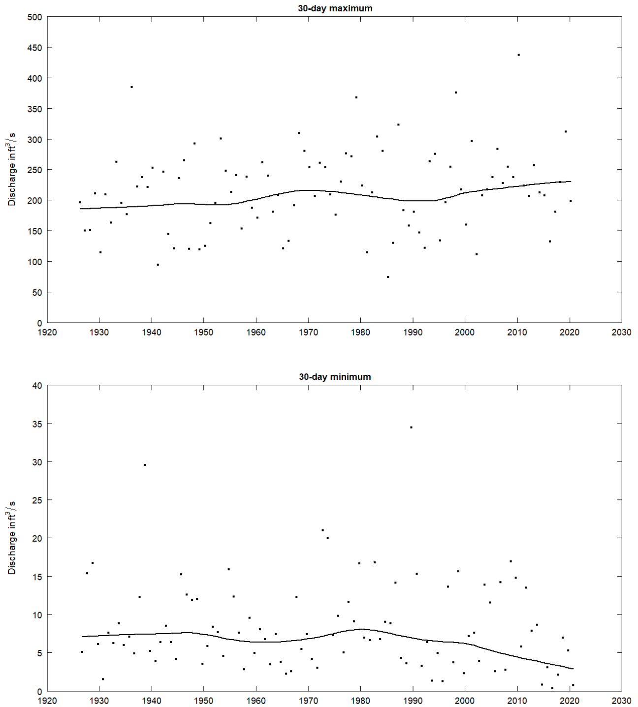
Figure 21. Maximum (top) and minimum (bottom) 30-day mean of daily mean discharges.
