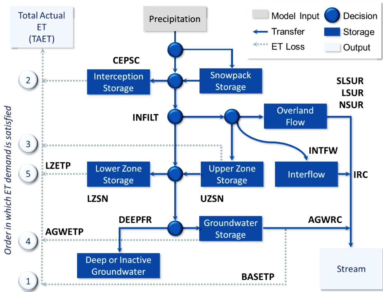
Figure 75. Hydrology model schematic for LSPC (based on Stanford Watershed Model).
