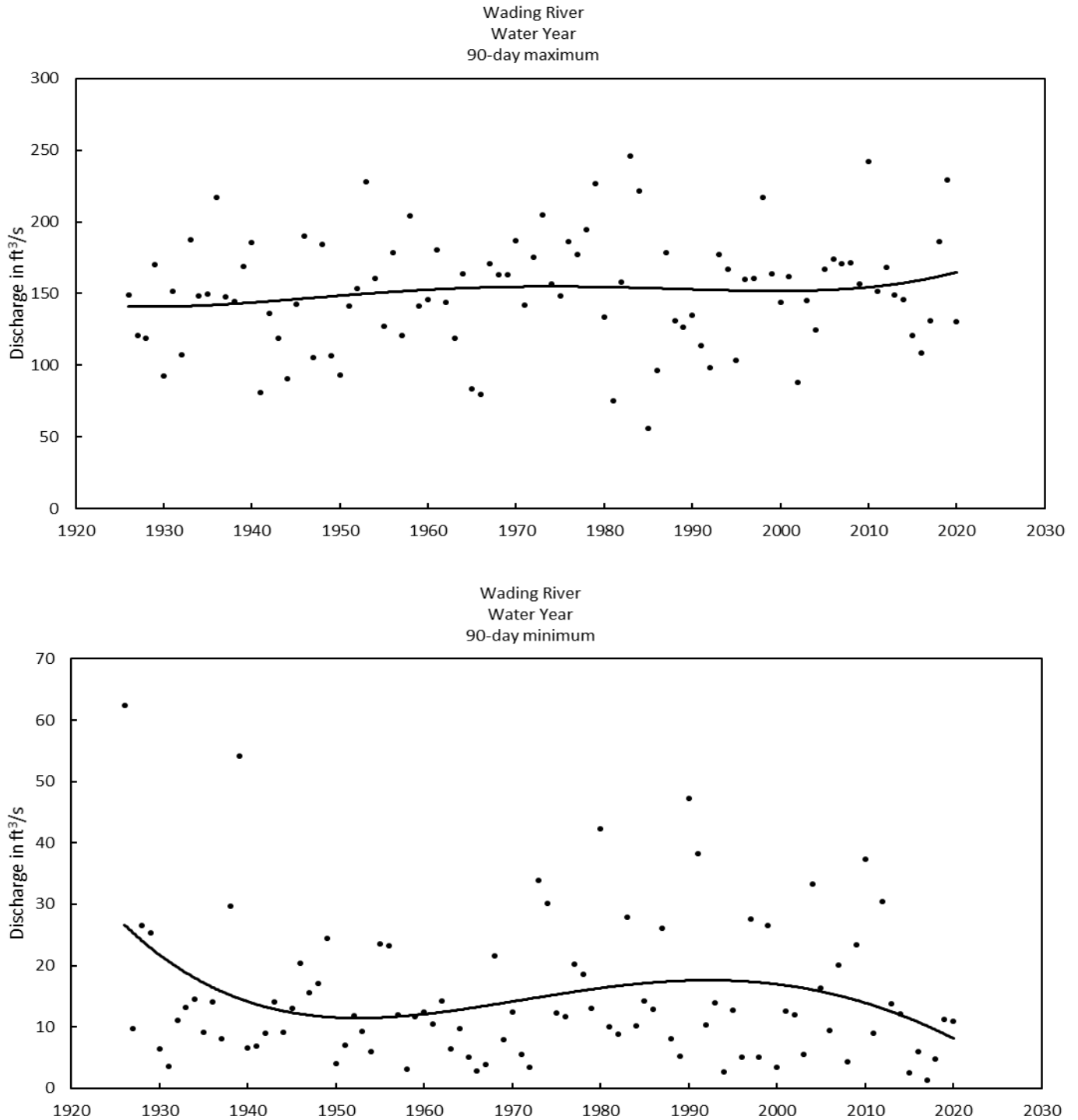
Figure 22. Maximum (top) and minimum (bottom) 90-day mean of daily mean discharges.
