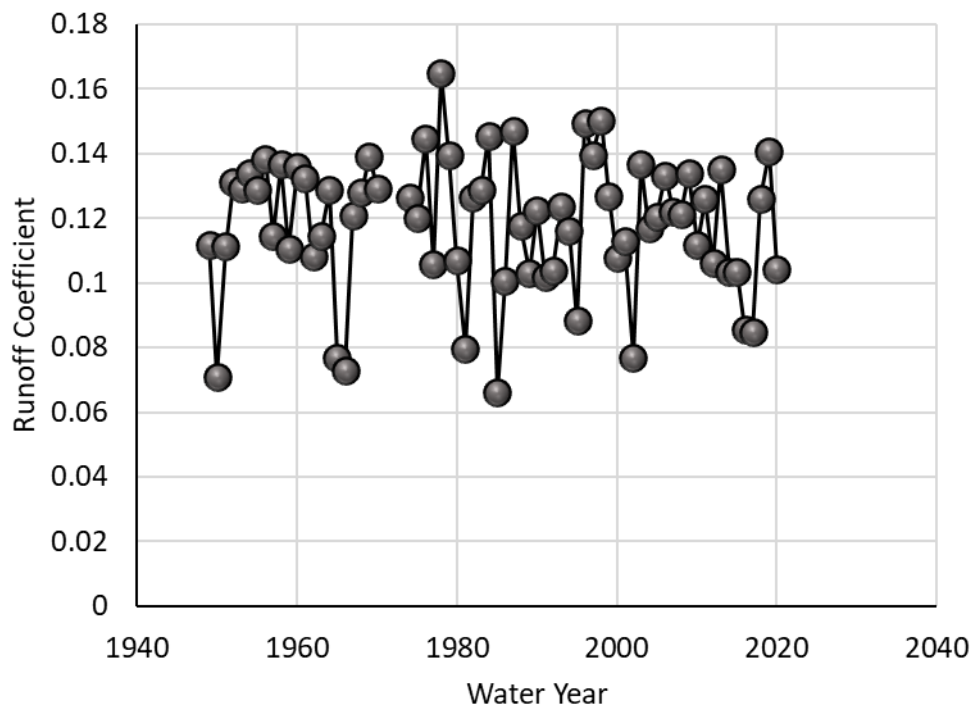
Figure 33. Runoff coefficient by water-year.
