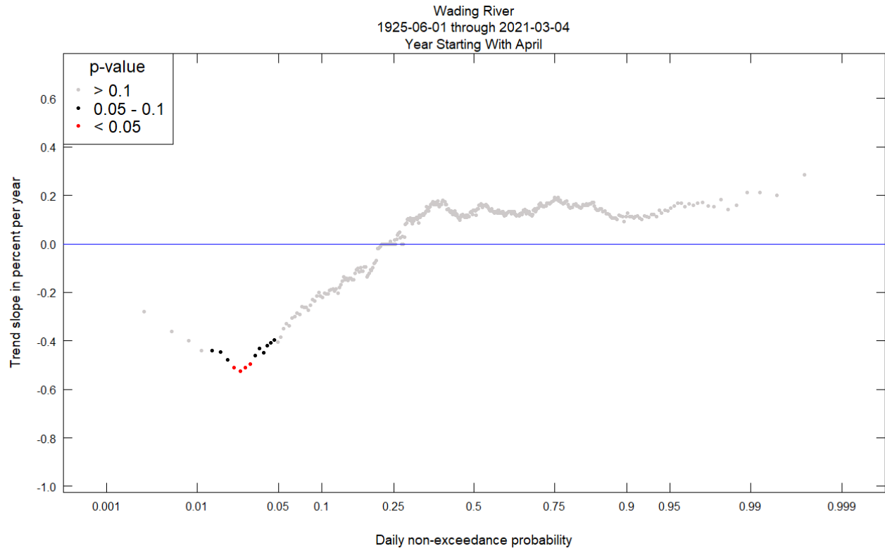
Figure 30. Quantile-Kendall plot 1925-2020.
