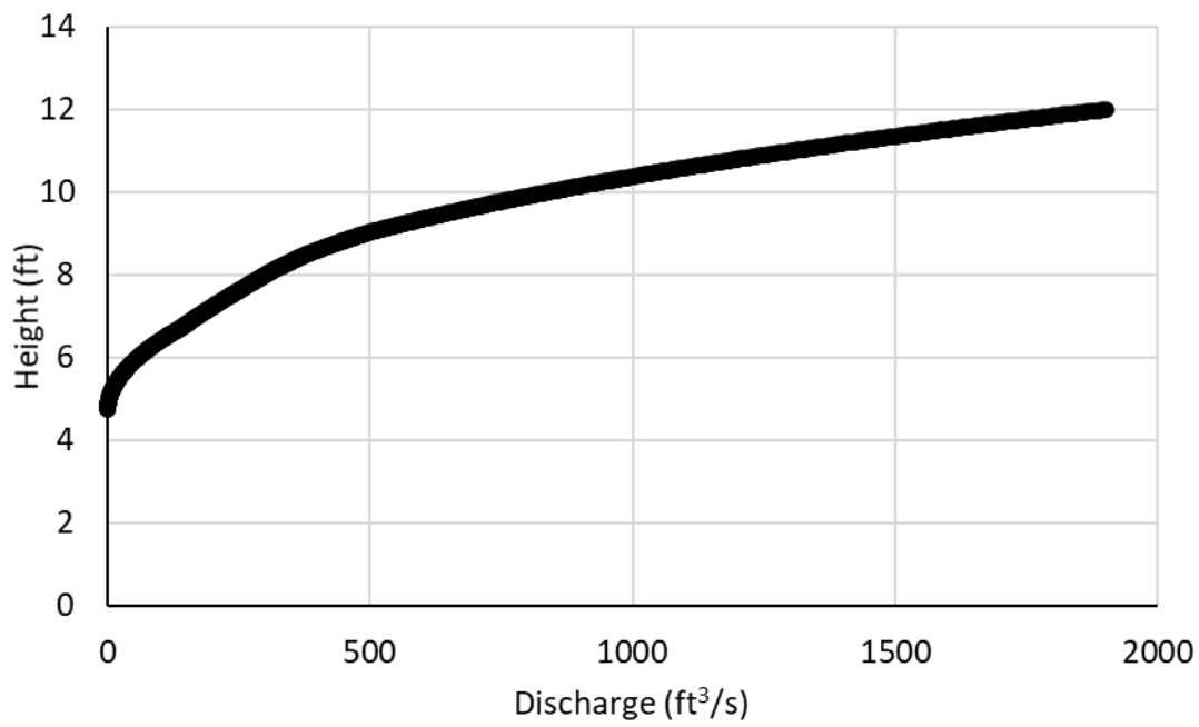
Figure 13. Rating curve for Wading River (01109000).
