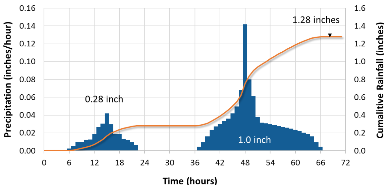
Figure 79. 72-hour storm hyetal distribution from Little Bear Creek Basin Plan (Snohomish County Public Works, 2017).
