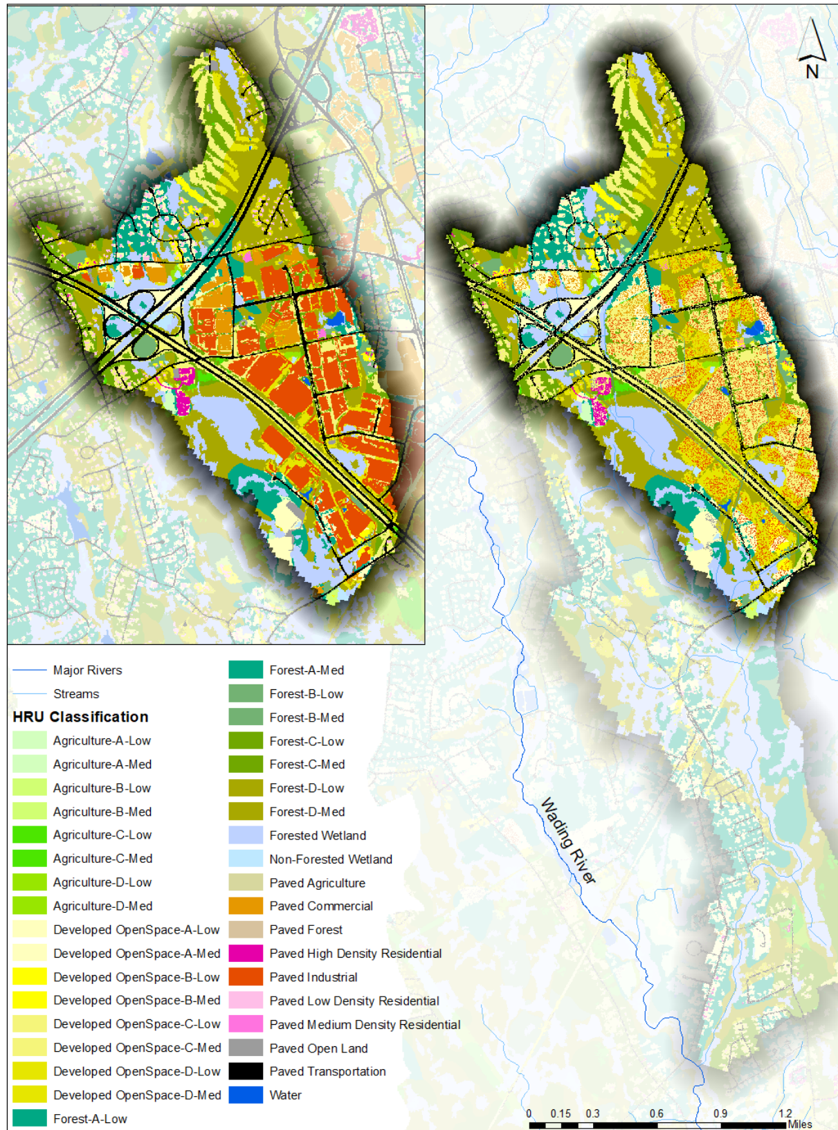
Figure 67. Peppered HRUs representing the effective impervious areas for Upper Hodges Brook (MIA on left and EIA on right).
