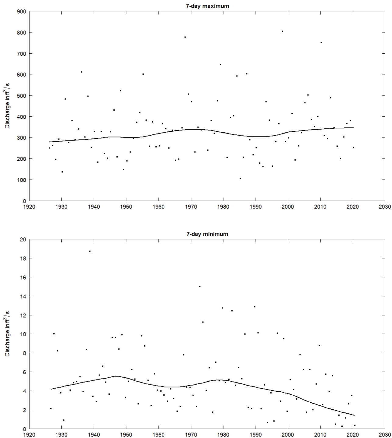
Figure 20. Maximum (top) and minimum (bottom) 7-day mean of daily mean discharges.
