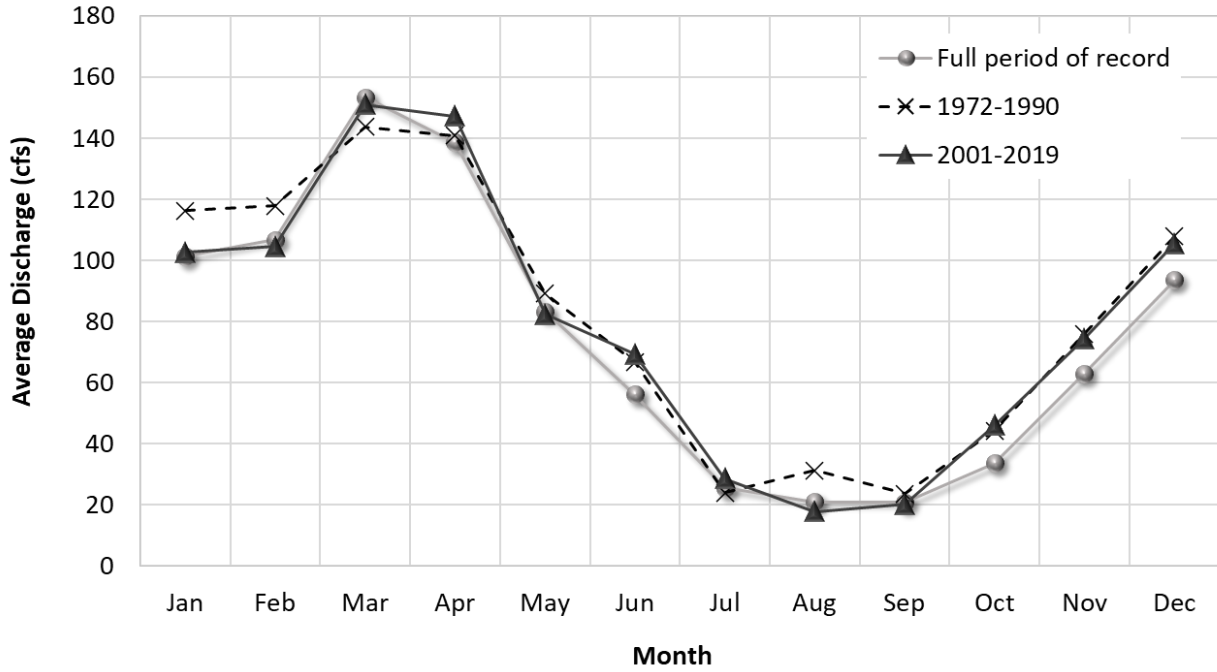
Figure 69. Monthly average discharge for the Wading River.
