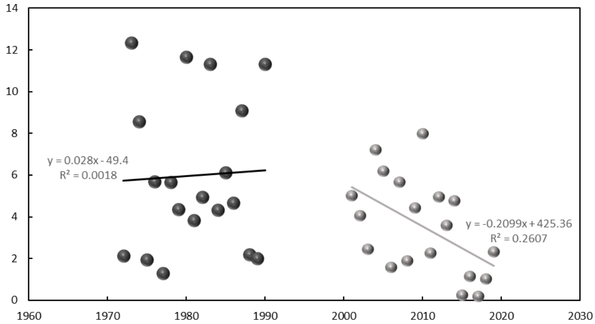
Figure 70. Comparison of 3-day minimum flows for water years 1972-1990 and 2001-2019 for the Wading River.
