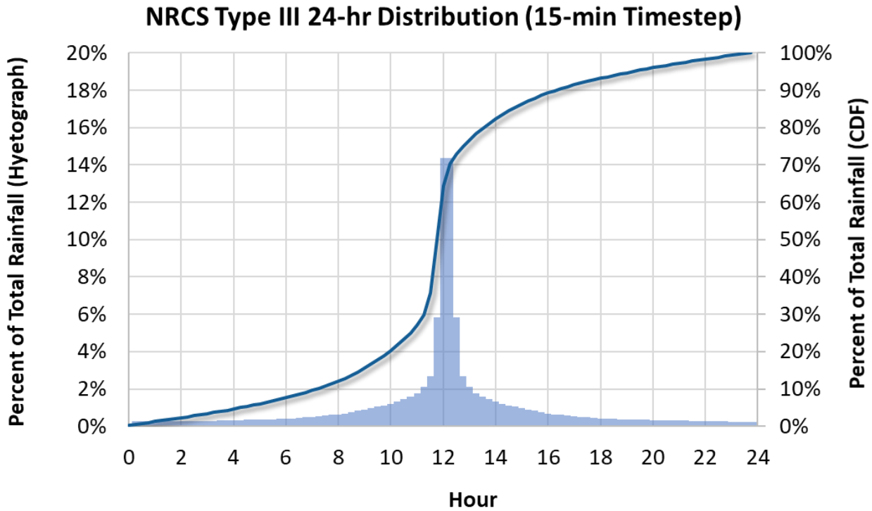
Figure 82. Massachusetts design-storm hyetograph for generating cost-effectiveness curves (NRCS).
