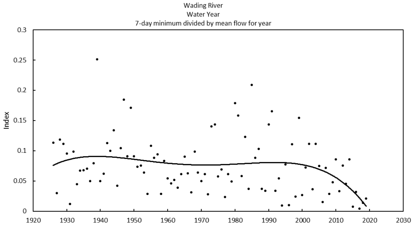
Figure 23. The minimum 7-day mean of daily mean discharges divided by the mean of mean daily discharges for the year.
