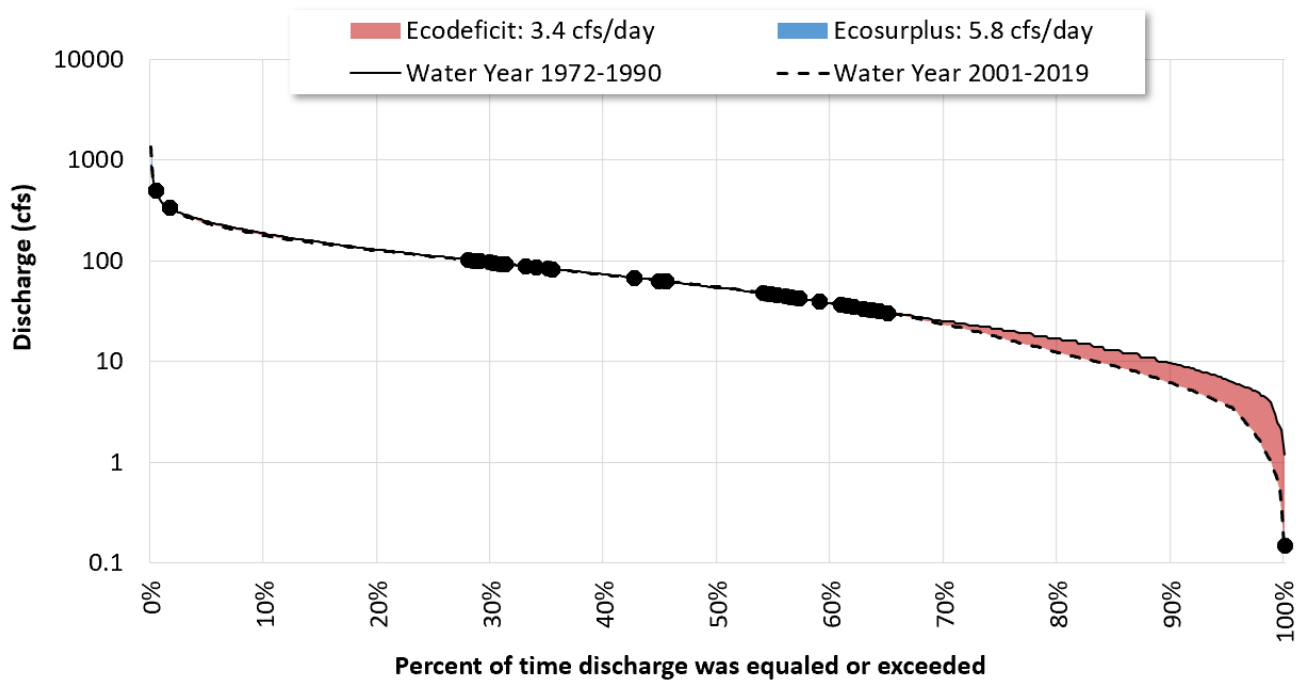
Figure 68. Ecosurplus and ecodeficit for the Wading River for 2001-2019 vs. 1972-1990. Black dots represent inflection points where the two curves change between surplus and a deficit.
