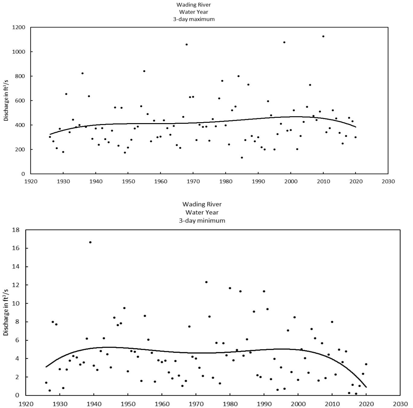
Figure 19. Maximum (top) and minimum (bottom) 3-day mean of daily mean discharges.
