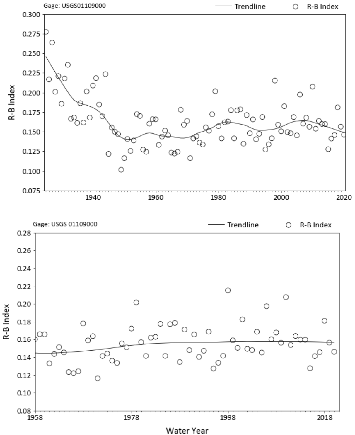
Figure 32. Richard-Baker Flashiness Index (R-B Index) for the Wading River (01109000) by water year based on daily mean discharge for the full period of record (top) and post-1958 (bottom).
