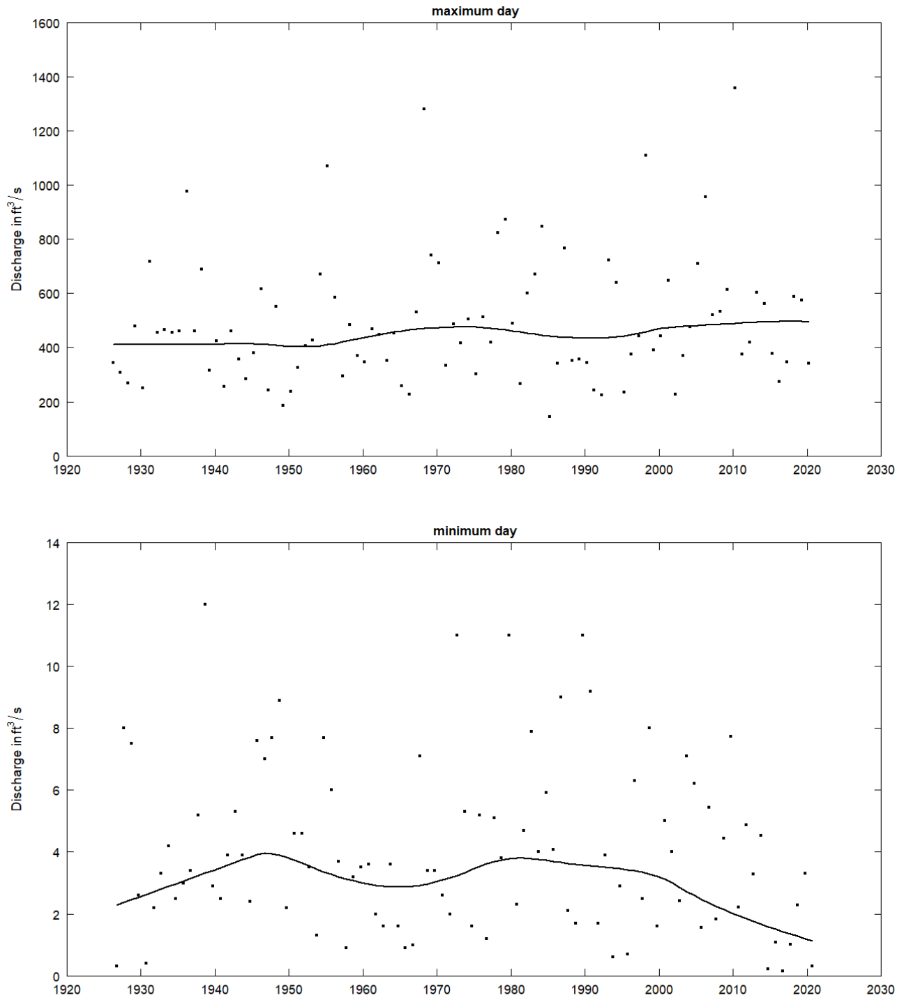
Figure 18. Maximum (top) and minimum (bottom) 1-day mean of daily mean discharges.
