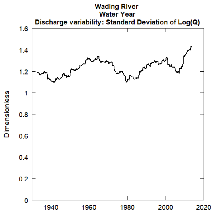
Figure 29. Discharge variability in the Wading River over time.
