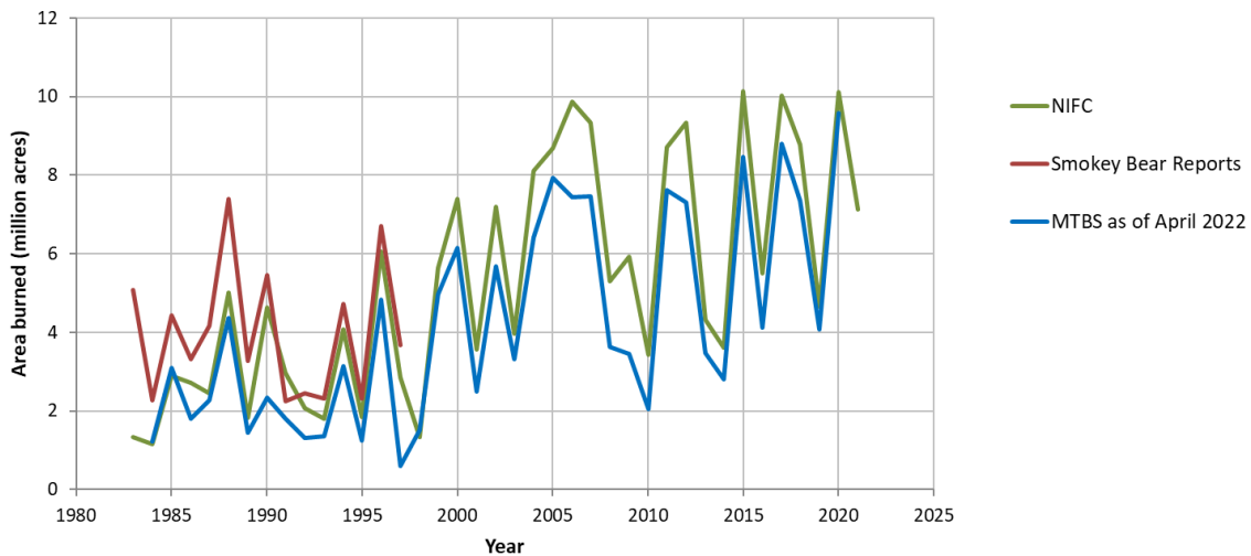
Figure TD-2. Comparison of Wildfire Extent from Three Data Sources, 1983–2021
