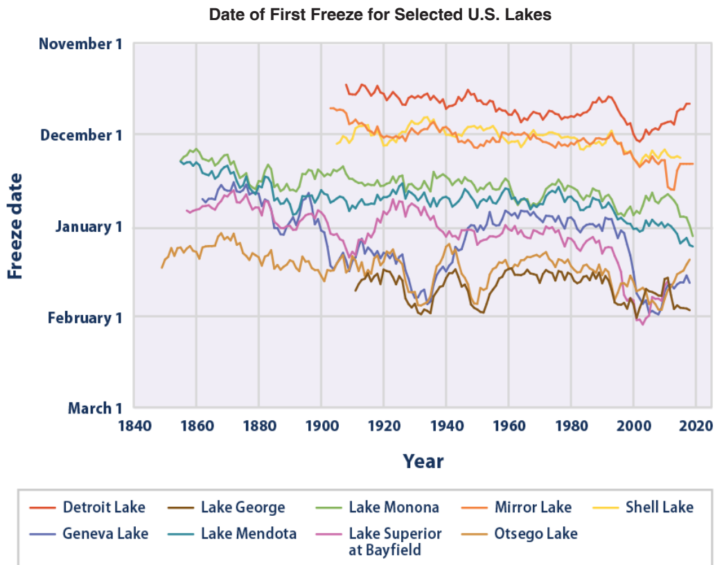
Figure 5. This graph shows the date of first freeze for nine U.S. lakes using data from 1850 to 2019. The lakes are generally freezing later than they did in the past – freeze dates have shifted at a rate of roughly half a day to one-and-a-half days per decade. Source: ( EPA Climate Change Indicators: Lake Ice webpage )
