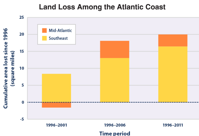
Figure 4. This graph shows the total amount of land converted to open water along the Atlantic coast during three time periods for the Southeast and Mid-Atlantic regions.
