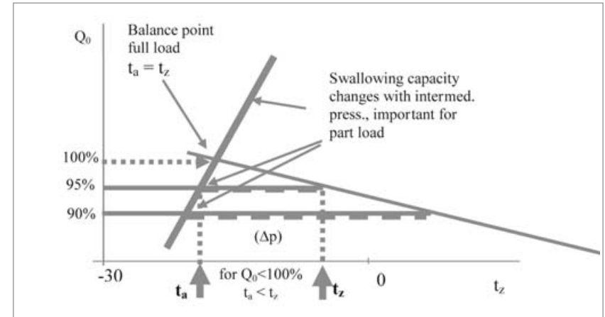
Figure 13: Intermediate-pressure control
