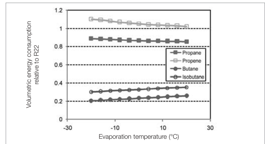
Figure 6: Volumetric energy consumption relative to R22 vs. evaporation temperature, at 40^{\circ}C condensation temperature, 0 K sub-cooling and 5 K superheat
