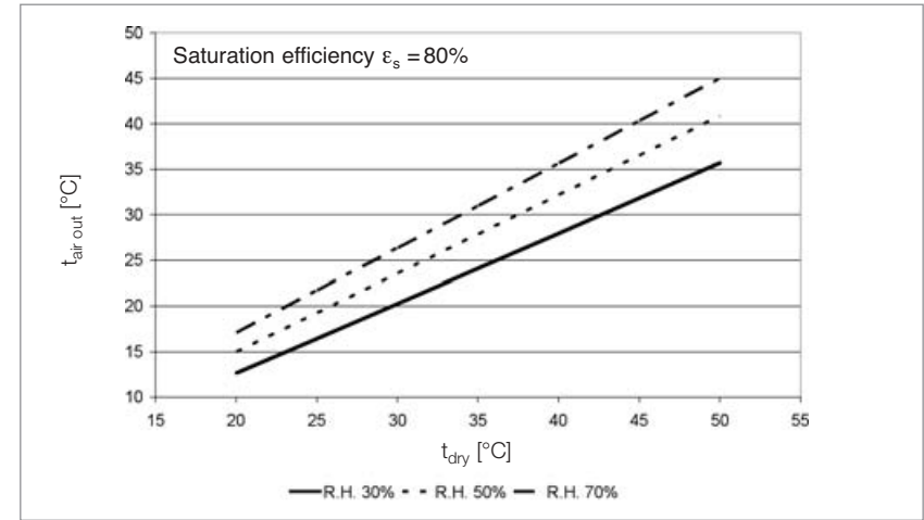
Figure 4: Calculated air temperature out of the evaporative cooling pack t_{air\ out} as a function of the air dry bulb temperature t_{dry} and for different relative humidity R.H. values
