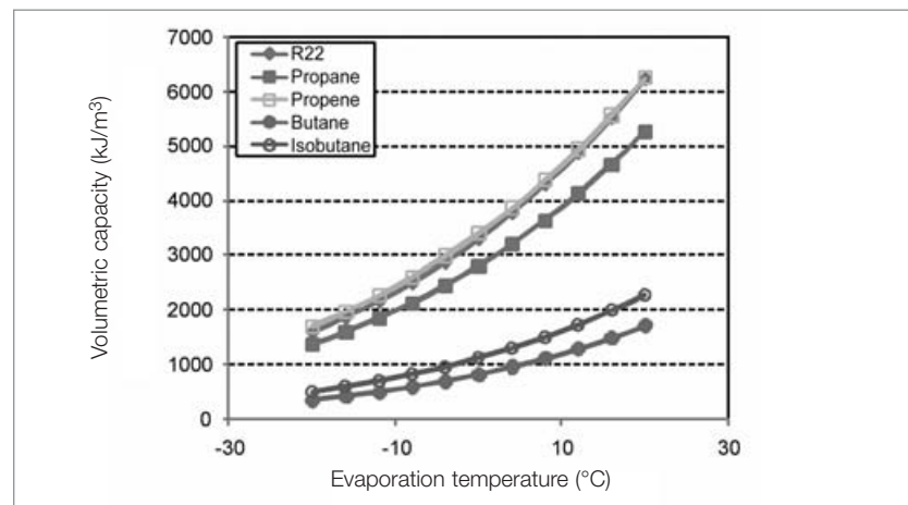
Figure 5: Volumetric cooling capacity vs. evaporation temperature, at 40^{\circ}C condensation temperature, 0 K sub-cooling and 5 K superheat
