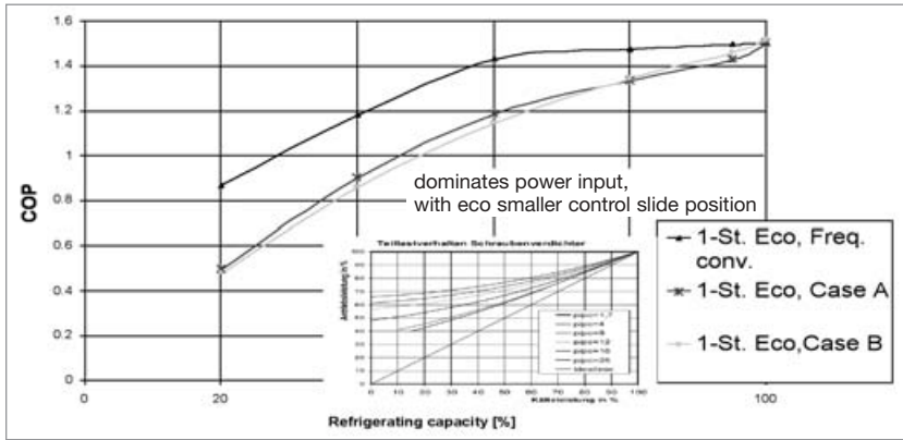
Figure 11: Variant (1) COP at full load and part load for speed control with arrangement of economizer port, case A (single-stage, economised, FC), and slide control with arrangement of economizer connection port on housing (single-stage, economised, case A), and in control slide (single-stage, economised, case B)
