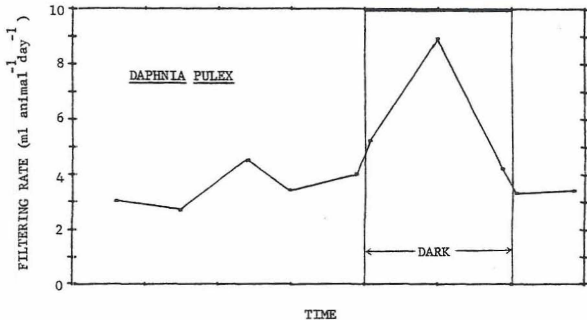
Figure 21. The diel pattern of filtering rate change at 18°C in a light:dark 16:8 photoperiod. Based on data from Starkweather (1975)
