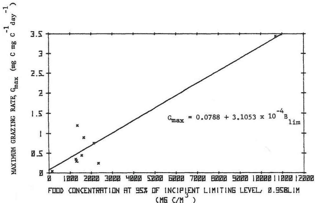
Figure 16. The relation of the maximum grazing rate, G_{\max} , to the incipient limiting food concentration, B_{\text{lim}} (values for 0.95 B_{\text{lim}} have actually been plotted because the Ivlev equation can not be directly solved for B_{\text{lim}} ). The line was fitted from values in Table 3
