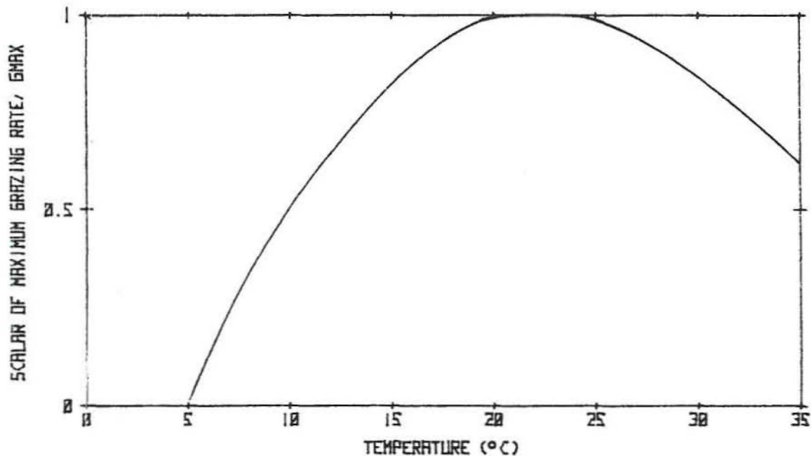
Figure 20. The relation of temperature to the relative increase in grazing rate for animals incompletely acclimated to test temperatures. In this example, the animal is fully acclimated to 20°C. The maximum grazing rate is equal to one on the ordinate to 10°C, and subjected to a sudden heat stress, than it will be for an animal acclimated to 20°C and subjected to the same relative stress. Furthermore, upper and lower lethal temperature limits will vary.
