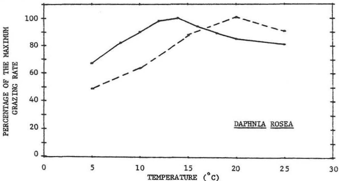
Figure 18. Grazing rate as a function of temperature for Daphnia rosea . Based on the data of Kibby (1971a) (———) and Burns and Rigler (1967) (— — —)
