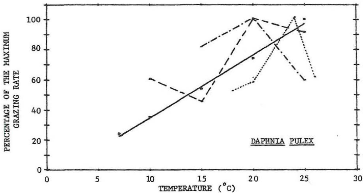
Figure 17. Grazing rate as a function of temperature for Daphnia pulex . Based on the data of Kryutchkova and Knodratyuk (1966) (.....), Burns (1969b) (-·-·-·-·), Geller (1975) (——— for long-term acclimation), and Geller (1975) (— — — for short-term acclimation)
