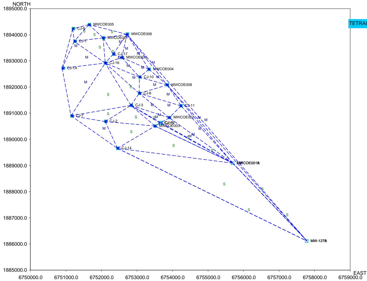
Figure 3 Source OU Well Sufficiency Results PCE
