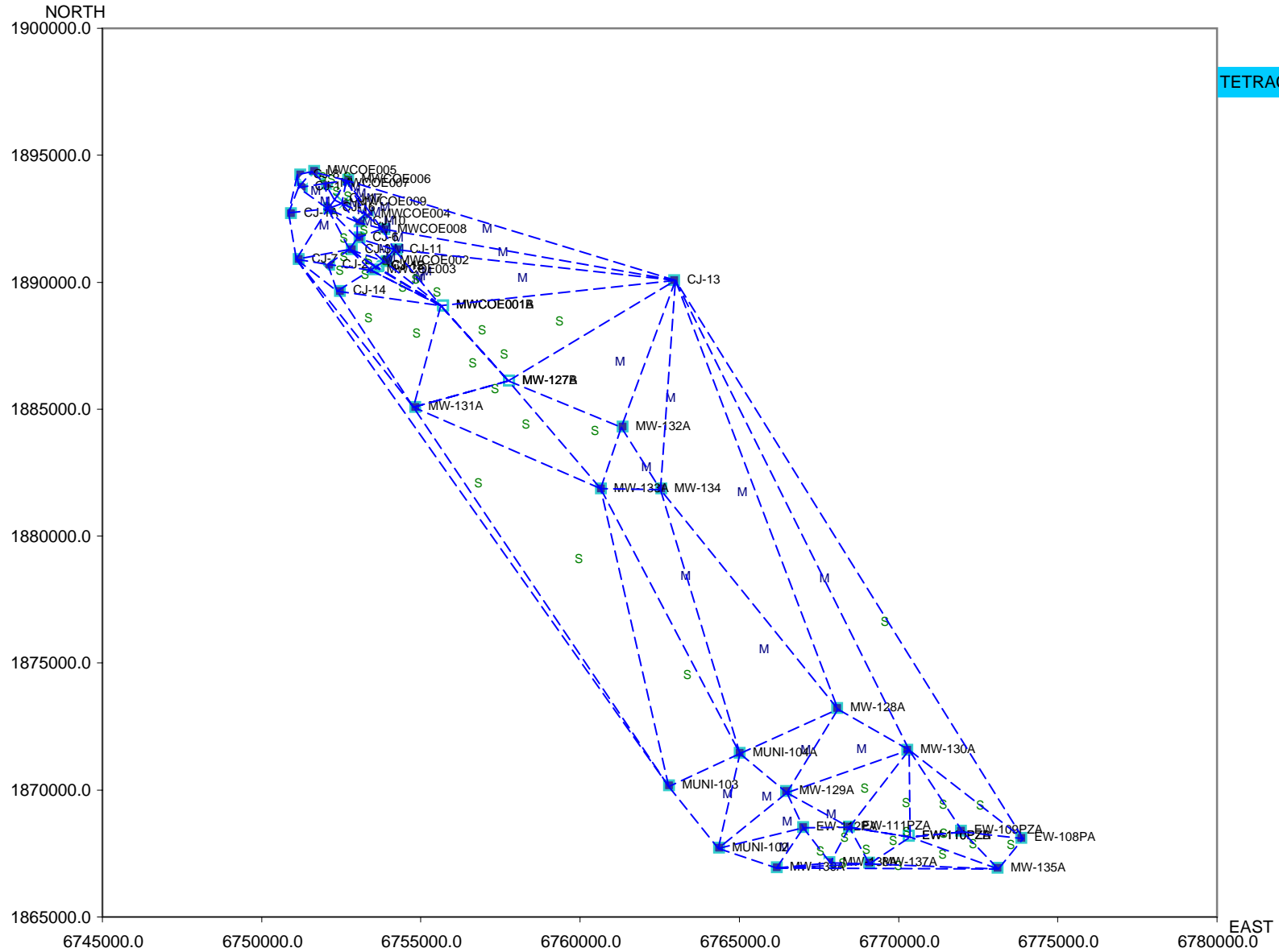
Figure 11 Muscoy Shallow Zone Well Sufficiency Results PCE
