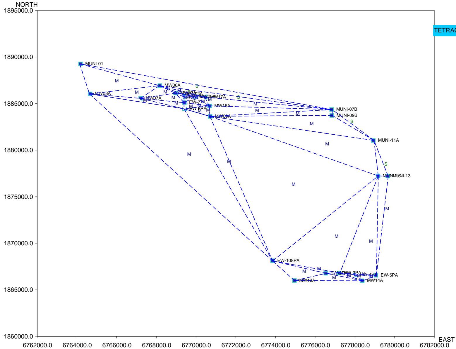
Figure 5 Newmark OU Shallow Zone Well Sufficiency Results PCE
