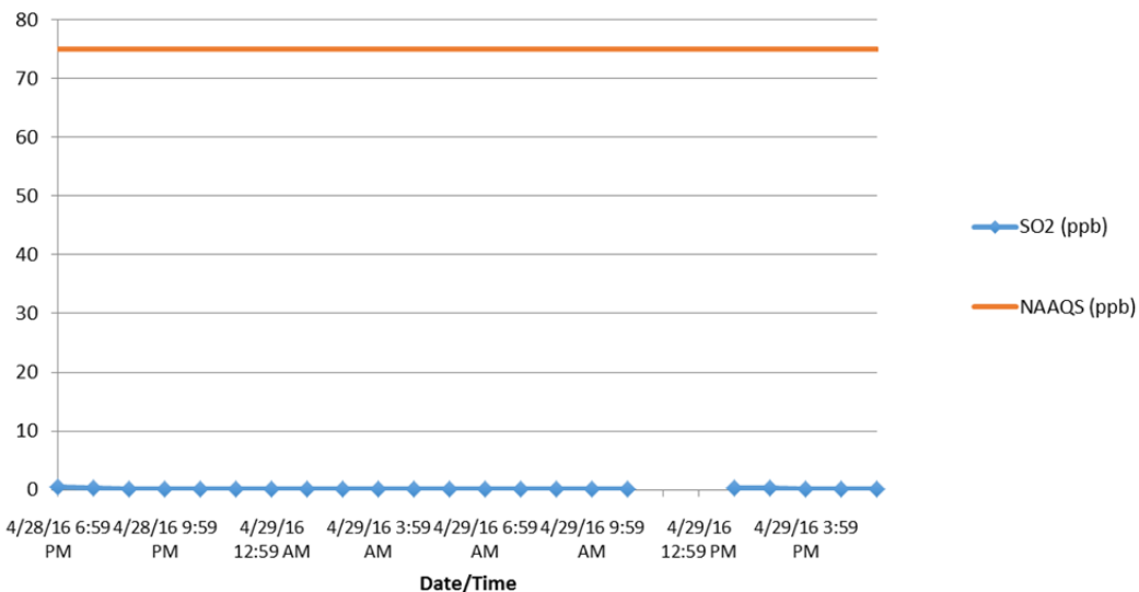
Hourly Averages SO2 (ppb)
