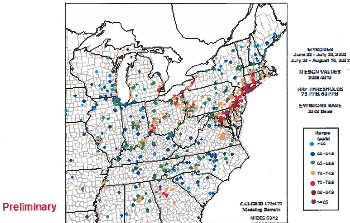
Figure 5: CALGRID 2018 “Scenario 6” Ozone Design Values (ppb)
