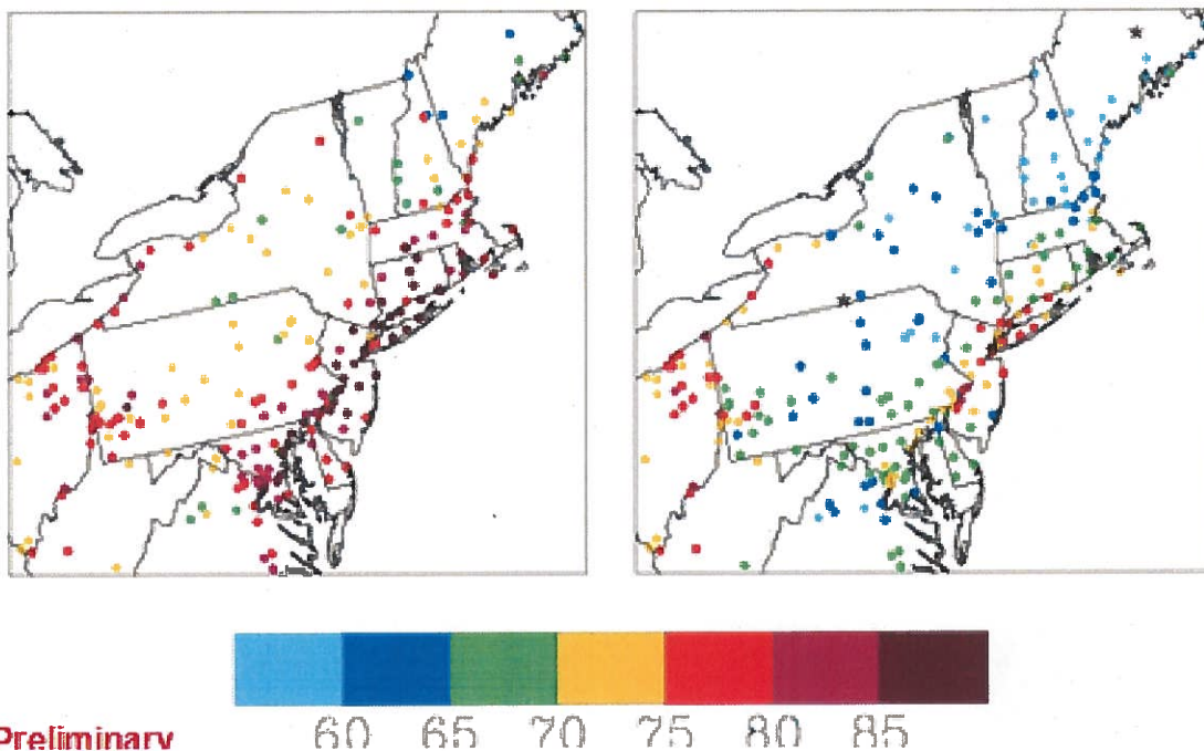
Figure 4: CMAQ 2007 Base Case and 2018 “Scenario 6” Ozone Design Values (ppb)
