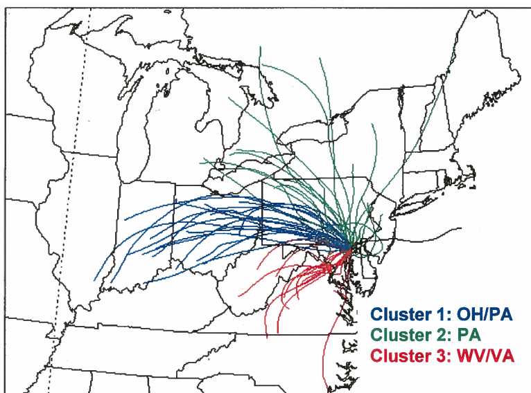
Figure A-4 HYSPLIT 48-Hour Back-Trajectory (1000 m)
