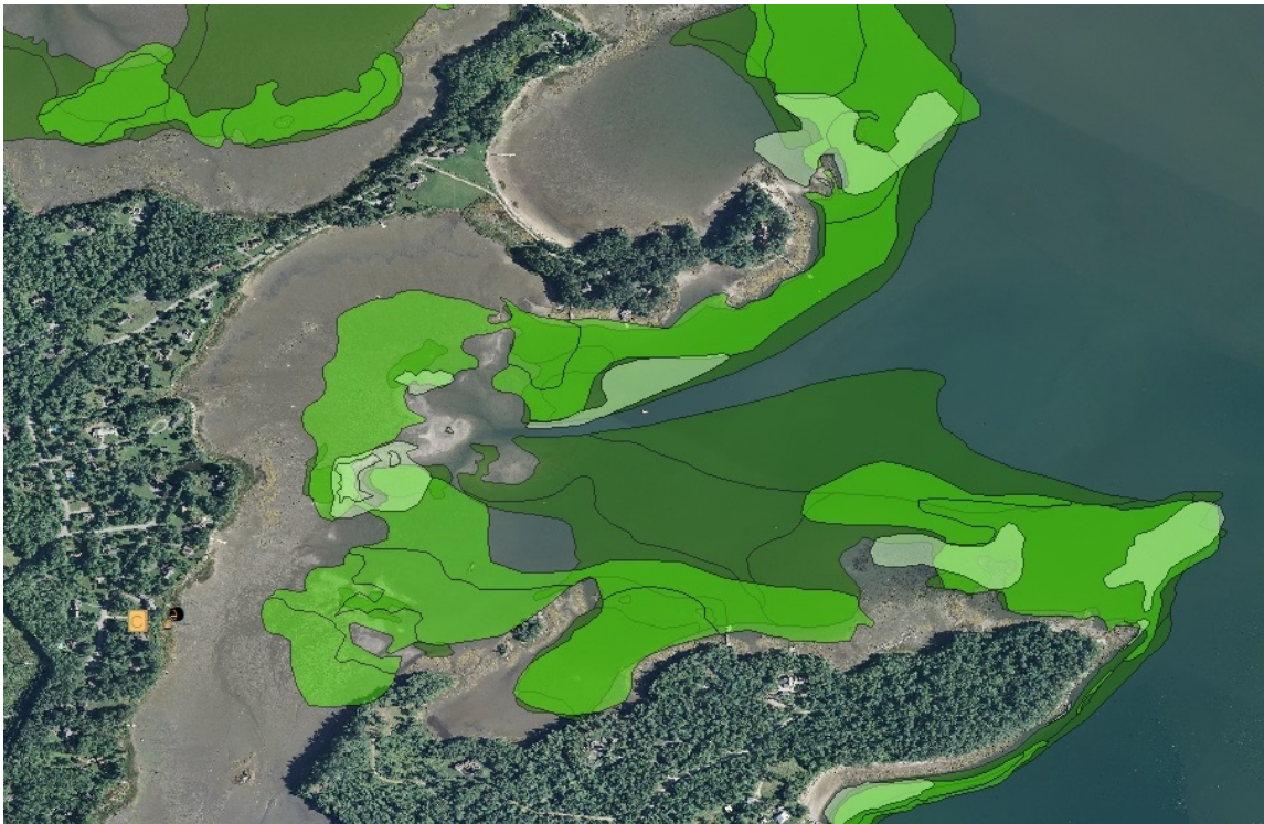
Figure 1. 2013 aerial imagery showing eelgrass distribution in 1993 (darkest green), 2001 (intermediate green) and 2013 (lightest green). Yarmouth Sea Meadows outfall location shown in the lower left corner.
