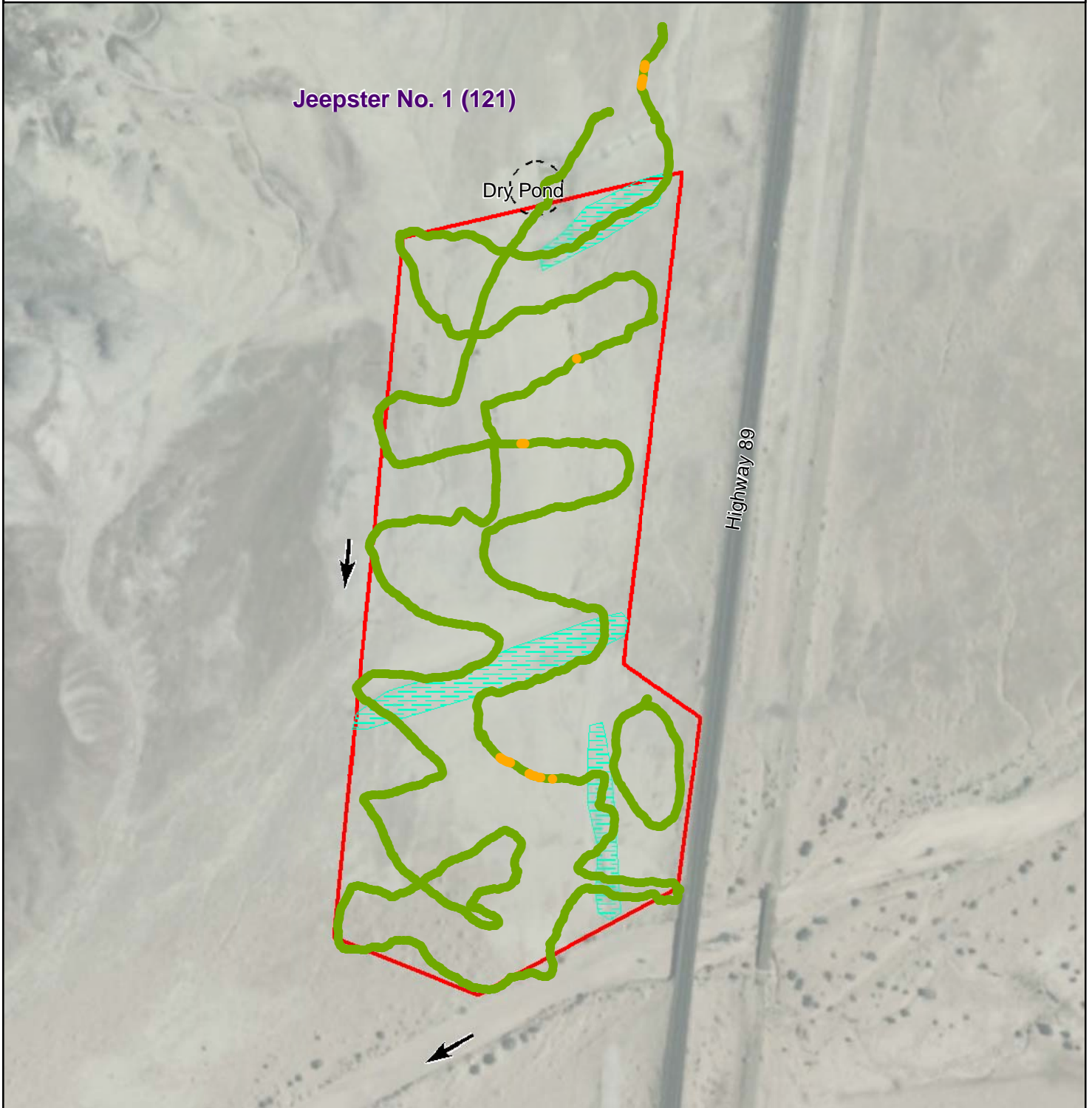
Figure 1 - Gamma Radiation Measurements, Above Two Times Background Jeepster No. 1 (121) Coalmine Mesa Chapter, Navajo Nation
