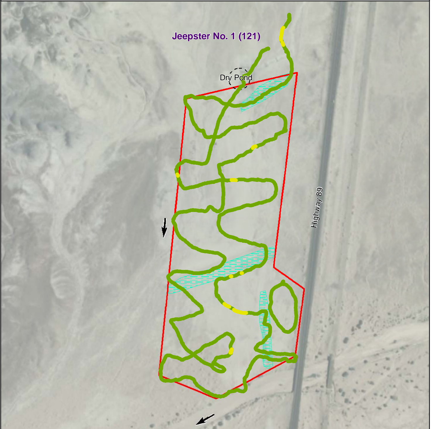
Figure 2 - Gamma Radiation Measurements Jeepster No. 1 (121) Coalmine Mesa Chapter, Navajo Nation
