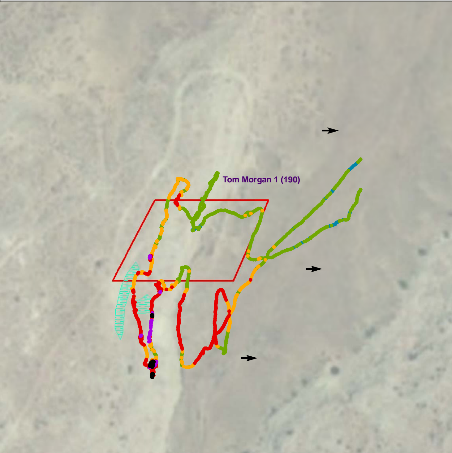
Figure 2 - Gamma Radiation Measurements Tom Morgan 1 (190) Red Mesa Chapter, Navajo Nation
