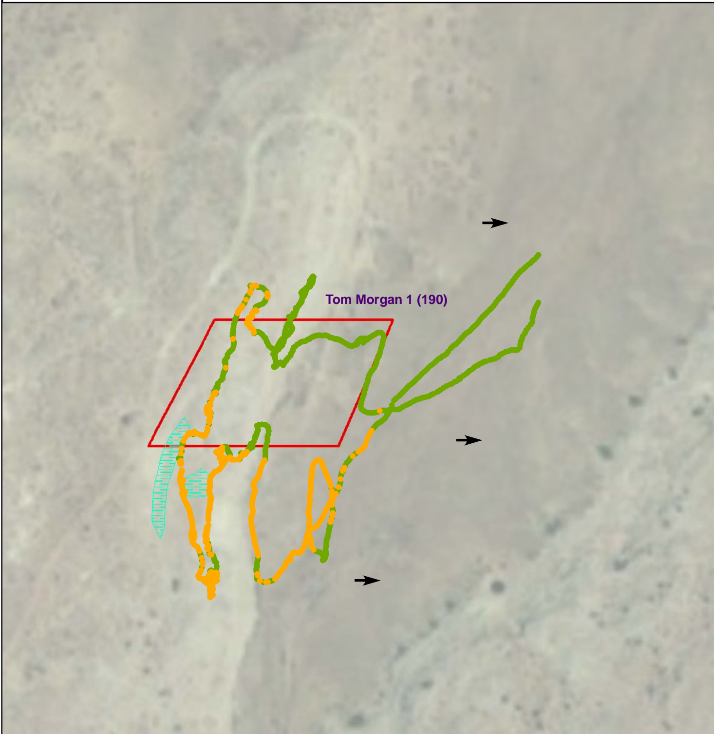
Figure 1 - Gamma Radiation Measurements, Above Two Times Background Tom Morgan 1 (190) Red Mesa Chapter, Navajo Nation
