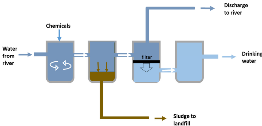
PRASA JAGUA CEIBA FLOW SCHEMATIC This diagram summarizes the WTP process.
