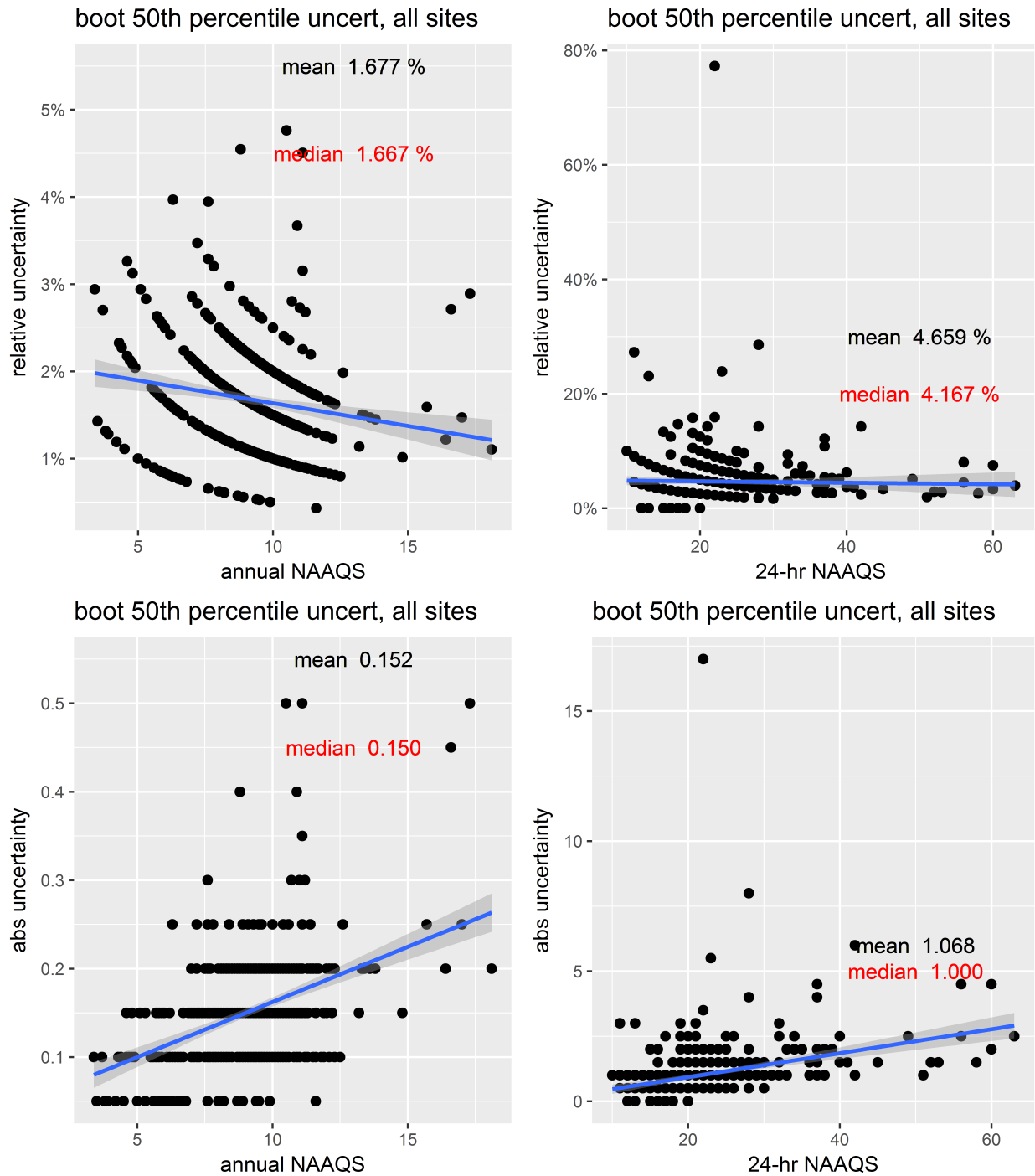
Figure 44: Bootstrap results from the 50% CIs for PM 2.5 DVs. The top two panels show the relative difference between the CI and the actual DV and the bottom two panels show the absolute difference between the values for the DVs at each site and the CI.
