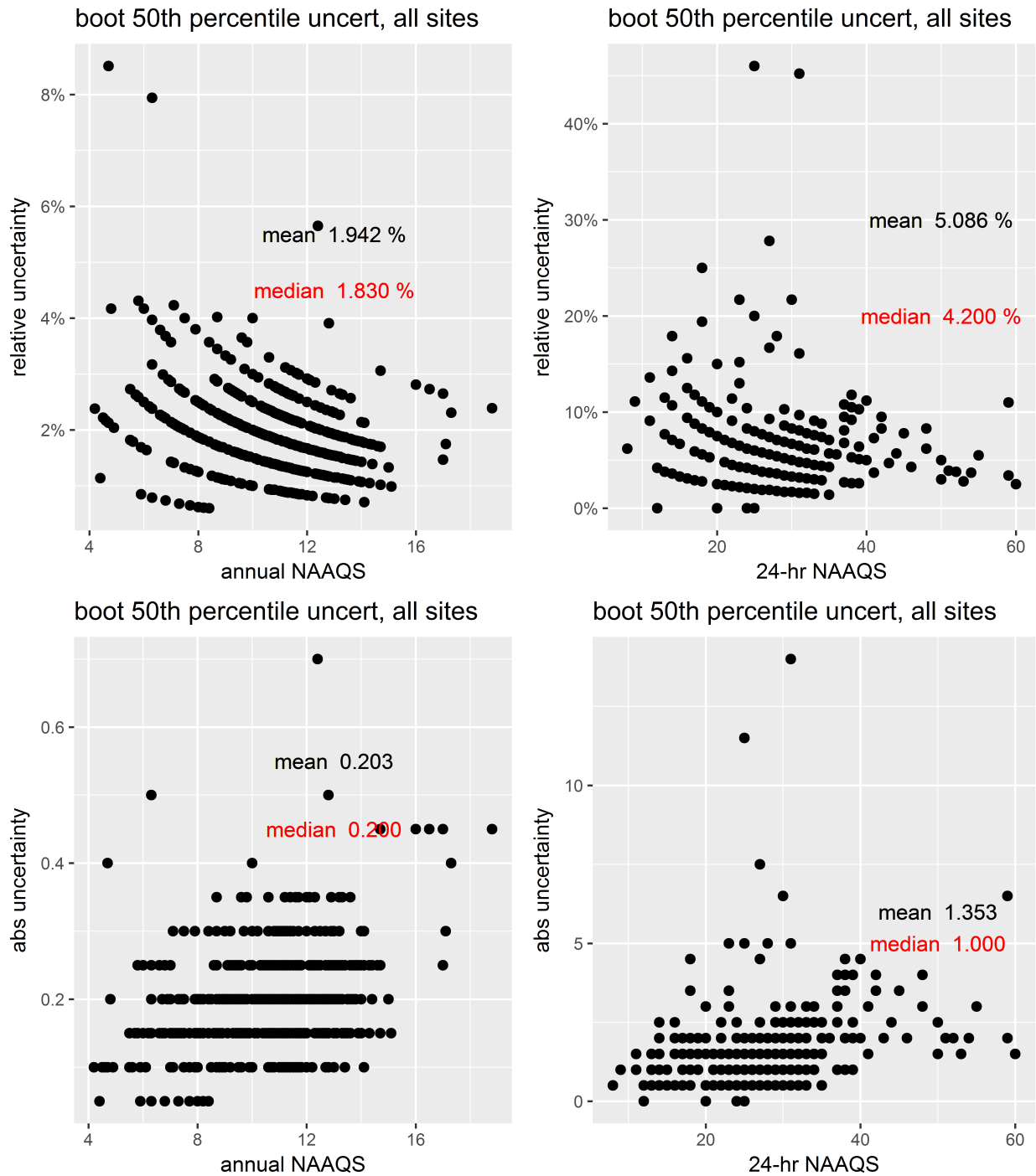
Figure 60: Bootstrap results from the 50% CIs for PM 2.5 DVs. The top two panels show the relative difference between the CI and the actual DV and the bottom two panels show the absolute difference between the values for the DVs at each site and the CI.
