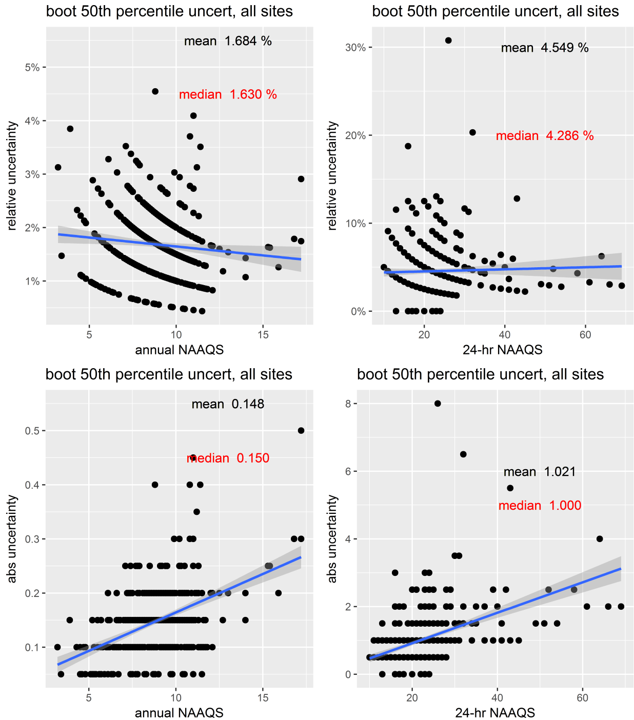
Figure 40: Bootstrap results from the 50% CIs for PM 2.5 DVs. The top two panels show the relative difference between the CI and the actual DV and the bottom two panels show the absolute difference between the values for the DVs at each site and the CI.
