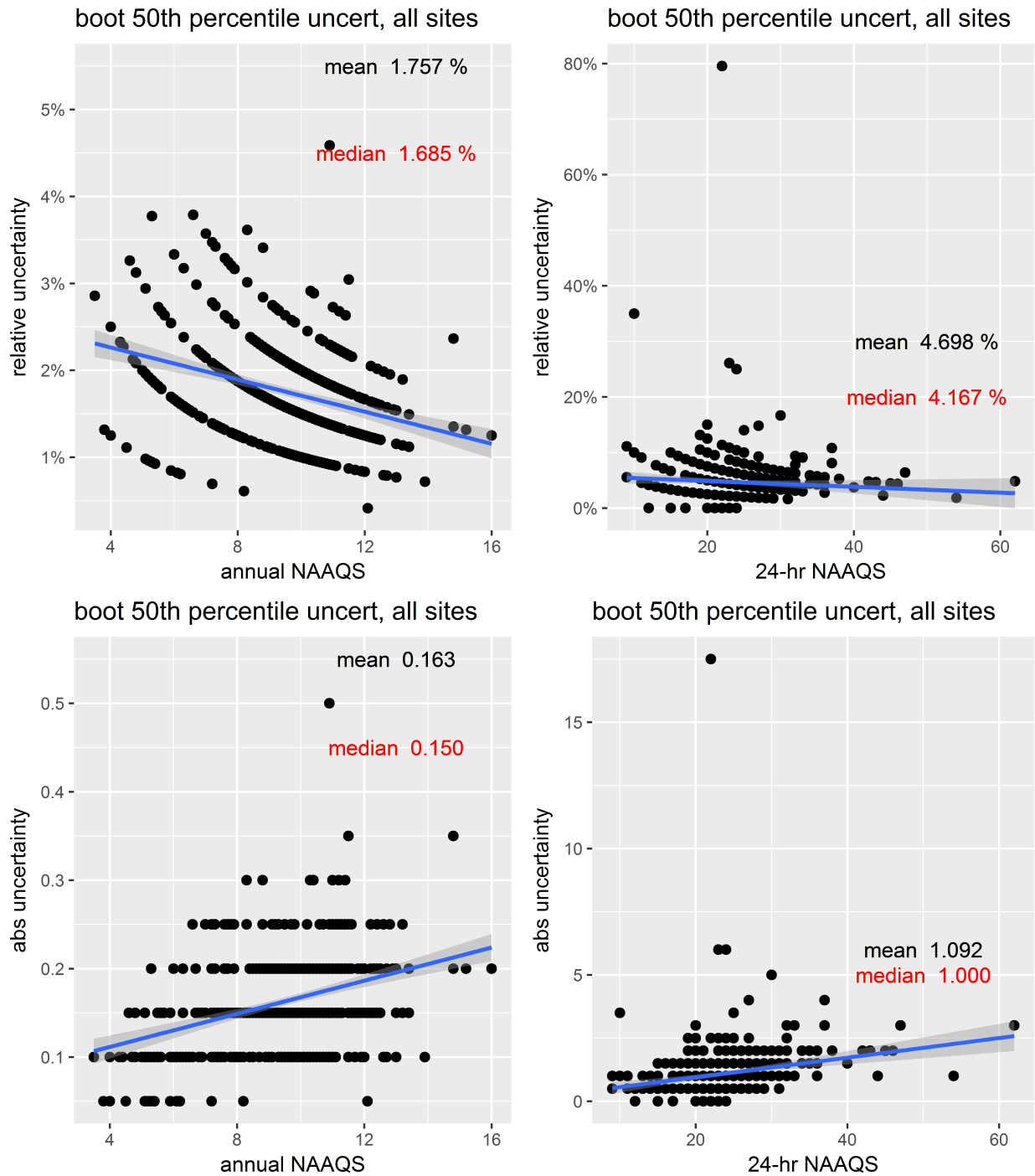
Figure 48: Bootstrap results from the 50% CIs for PM 2.5 DVs. The top two panels show the relative difference between the CI and the actual DV and the bottom two panels show the absolute difference between the values for the DVs at each site and the CI.
