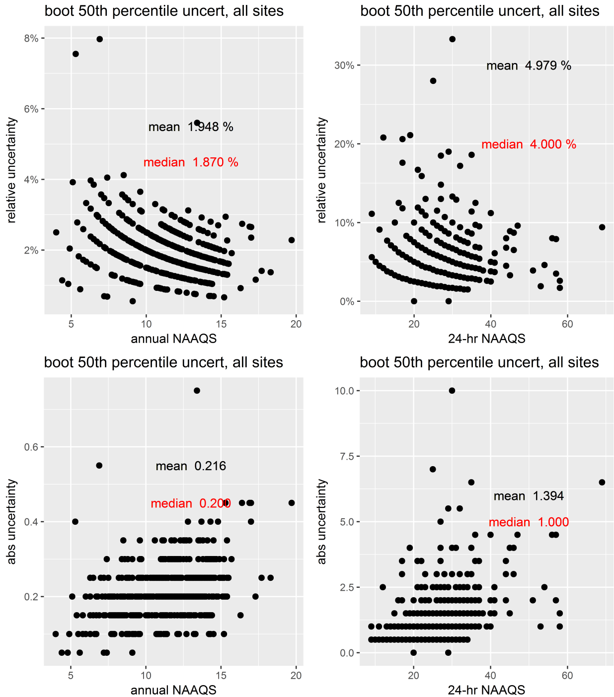
Figure 64: Bootstrap results from the 50% CIs for PM 2.5 DVs. The top two panels show the relative difference between the CI and the actual DV and the bottom two panels show the absolute difference between the values for the DVs at each site and the CI.
