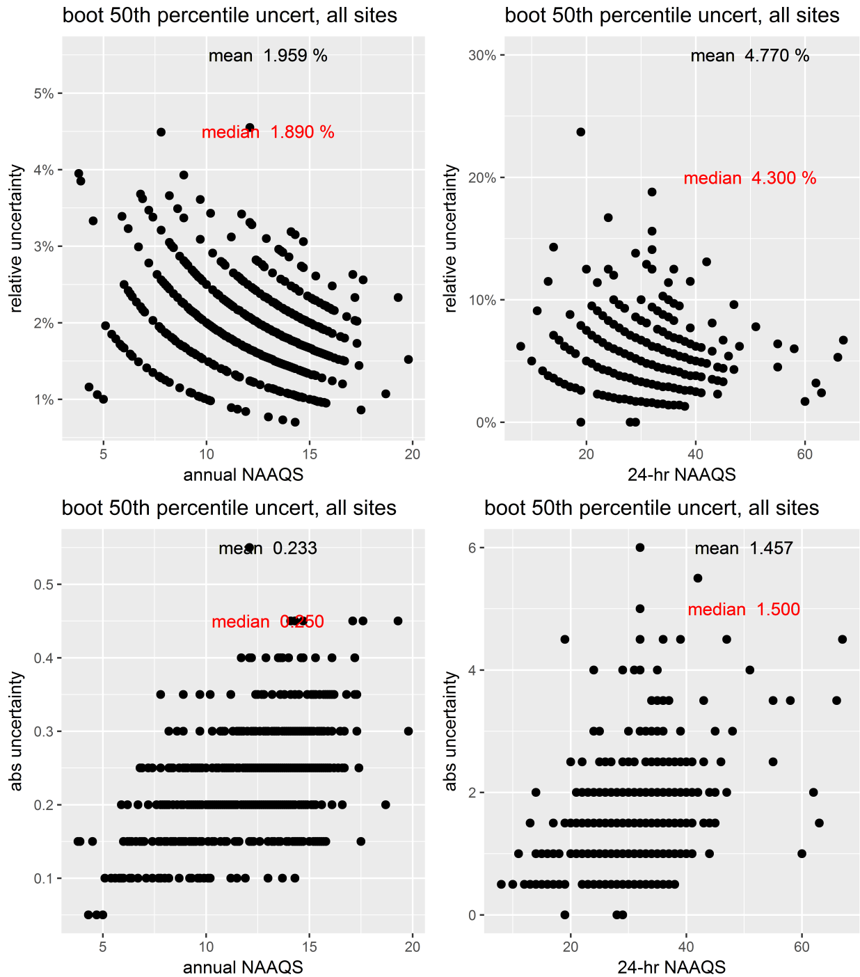
Figure 68: Bootstrap results from the 50% CIs for PM 2.5 DVs. The top two panels show the relative difference between the CI and the actual DV and the bottom two panels show the absolute difference between the values for the DVs at each site and the CI.
